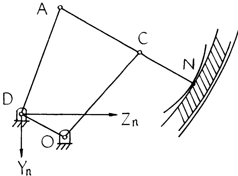
(a) GEAR TOOTH CONVEX SIDE
