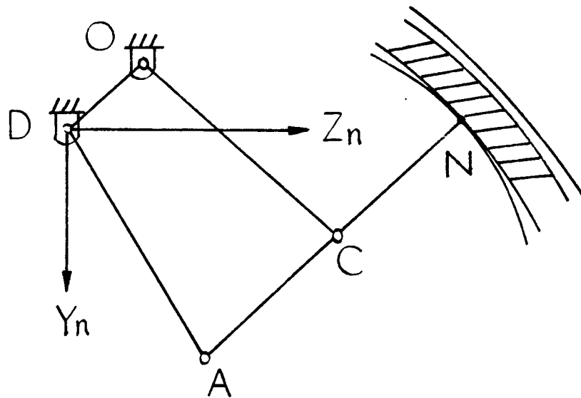
(b) GEAR TOOTH CONCAVE SIDE
