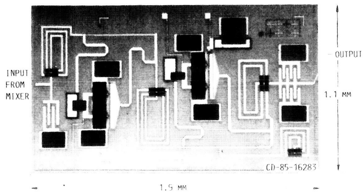
FIGURE 14. - 2- TO 6-GHz INTERMEDIATE-FREQUENCY AMPLIFIER.
