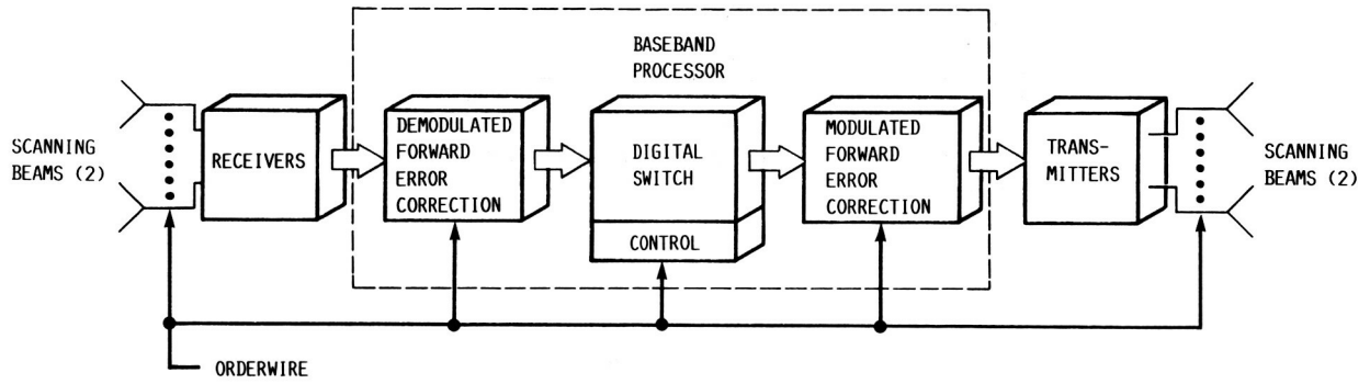
FIGURE 2. - COMMUNICATIONS PAYLOAD FOR EXPERIMENTAL FLIGHT SYSTEM BASED ON PHASED-ARRAY ANTENNA AND BASEBAND PROCESSING TECHNOLOGY.
