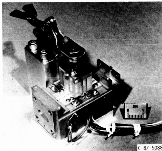
FIGURE 7. - 20-GHz TEST FIXTURE FOR CHARACTERIZING PACKAGED MMICs. THE TRANSITION TO MICROSTRIP IS ACCOMPLISHED USING E-PLANE WAVEGUID PROBES.
