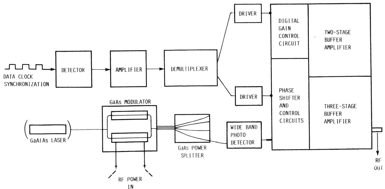
FIGURE 17. - BLOCK CIRCUIT DIAGRAM OF OPTICAL/MMIC INTERFACE.
