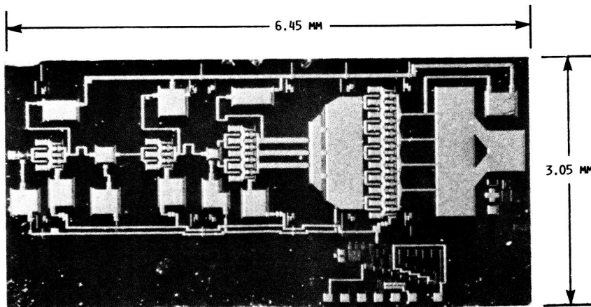
FIGURE 5. - MMIC CHIP FOR 20-GHz VARIABLE-POWER AMPLIFIER.
