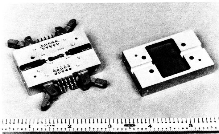
FIGURE 10. - 30-GHZ INTERCONNECTED RECEIVE MODULE CONSISTING OF THE LOW-NOISE AMPLIFIER, GAIN CONTROL AMPLIFIER, AND PHASE SHIFTER SUBMODULE. SHOWN ARE THE THREE CHIPS, FINLINE TRANSITIONS, OFF CHIP BIAS FILTERS, AND WR-Z8 WAVEGUIDE HOUSING.
