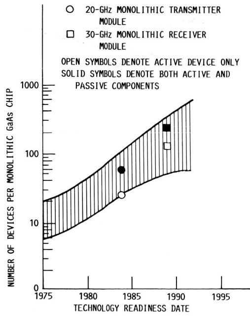
FIGURE 1. - LEVEL OF MONOLITHIC INTEGRATION OF MICROWAVE DEVICES AND PASSIVE COMPONENTS ON GaAs SUBSTRATE.
