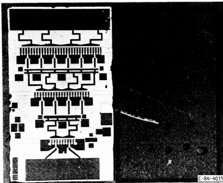
FIGURE 8. - DUAL-STAGE AMPLIFIER.
