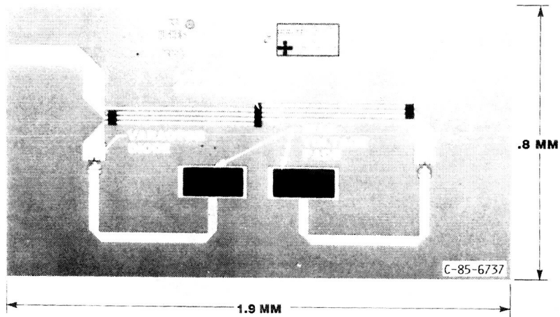
FIGURE 16. - 23.5-GHZ PHASE SHIFTER.
