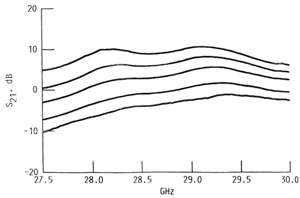
FIGURE 11. - FIVE GAIN STATES OF THE INTERCONNECTED RECEIVE MODULE AT ZERO PHASE SHIFT. BIAS ON THE SECOND GATE OF EACH STAGE WAS VARIED DISCREETLY FROM 0 TO -0.75 V.
