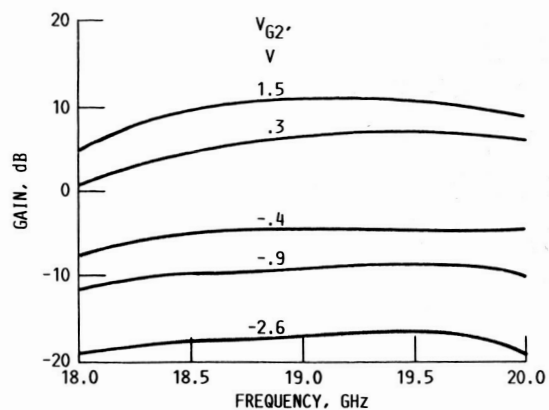
FIGURE 6. - MEASURED GAIN VERSUS FREQUENCY RESPONSE OF VARIABLE-POWER AMPLIFIER. RF INPUT: 0 dBm. DRAIN VOLTAGE: 5.5 V. DRAIN CURRENT: 300 mA. FIRST GATE VOLTAGE: 0.73 V. SECOND GATE VOLTAGE ( V_{G2} ) IS VARIED AS SHOWN.
