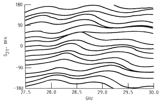
FIGURE 12. - DIFFERENTIAL INSERTION PHASE FOR 16 PHASE STATES OF THE INTERCONNECTED RECEIVE MODULE AT MAXIMUM GAIN.
