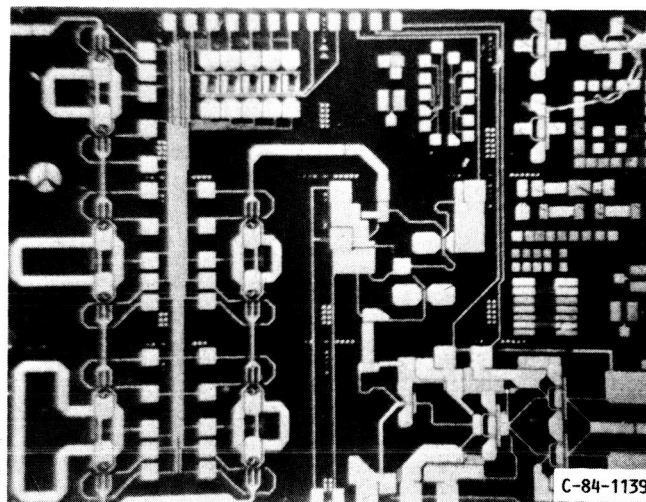
FIGURE 3. - 20-GHz MONOLITHIC PHASE SHIFTER MODULE (4.8x6.4x0.127 MM).
