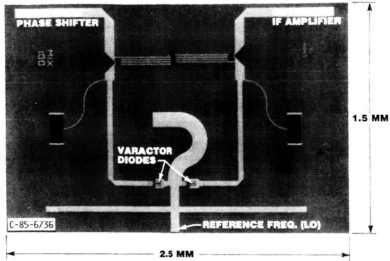
FIGURE 15. - K_a BAND MIXER.
