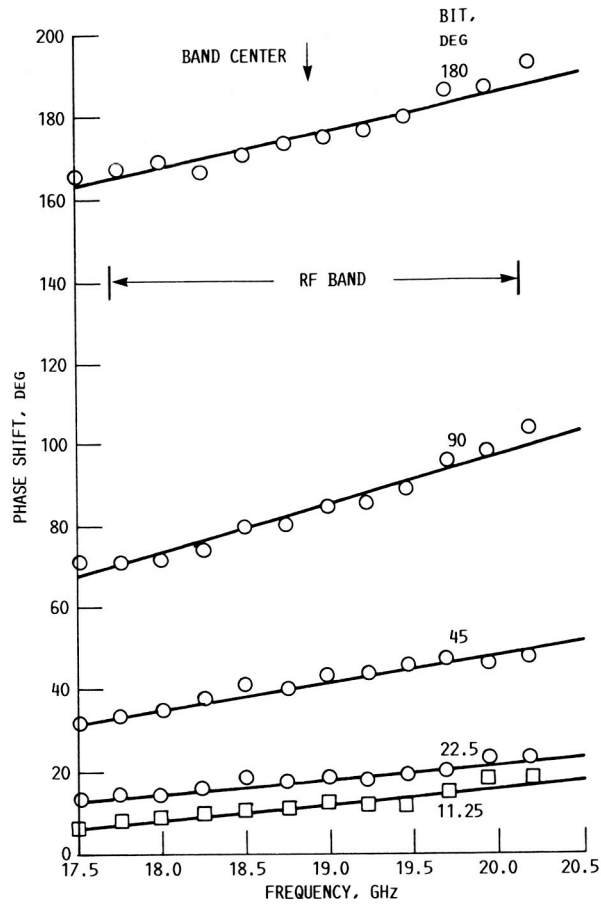
FIGURE 4. - PHASE SHIFT VERSUS FREQUENCY FOR FIVE PHASE SHIFTER STATES FOR 20-GHz VARIABLE-PHASE-SHIFTER MODULE.
