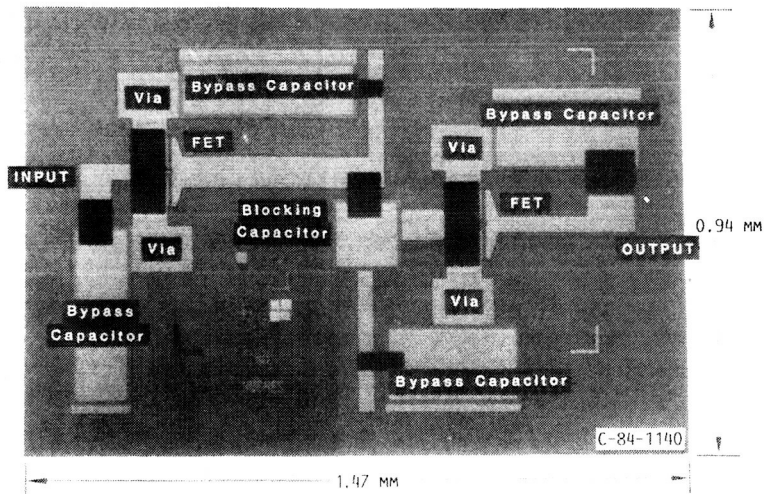
FIGURE 13. - 27.5- TO 30-GHz MONOLITHIC LOW-NOISE AMPLIFIER.
