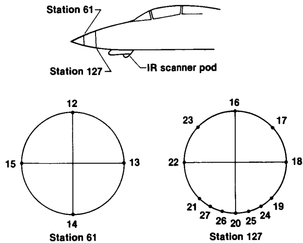
Figure 6. Nose section pressure orifices (numbered locations as viewed from front of nose cone).
