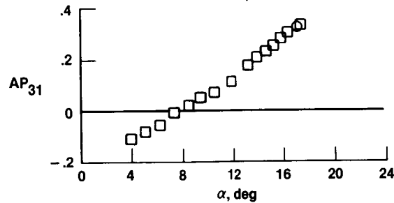
(i) M = 1.23 , orifices at station 127.
