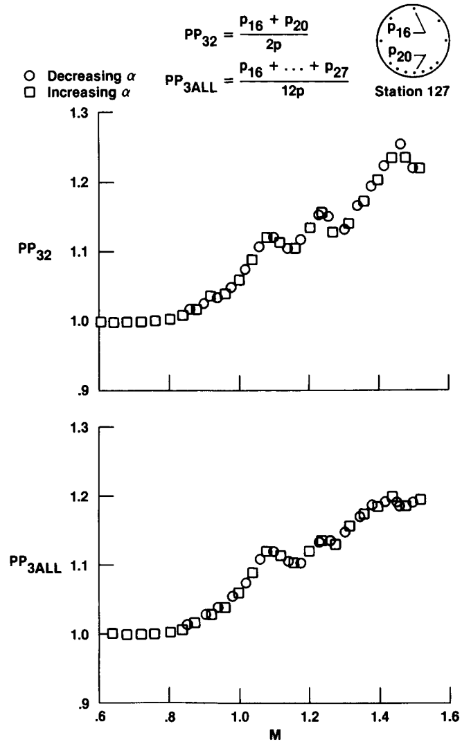
(b) Orifices at station 127.
