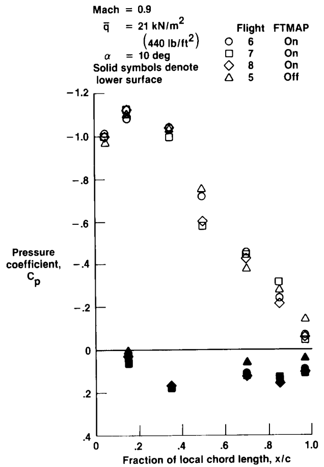
(b) 0.937 wing semispan.
