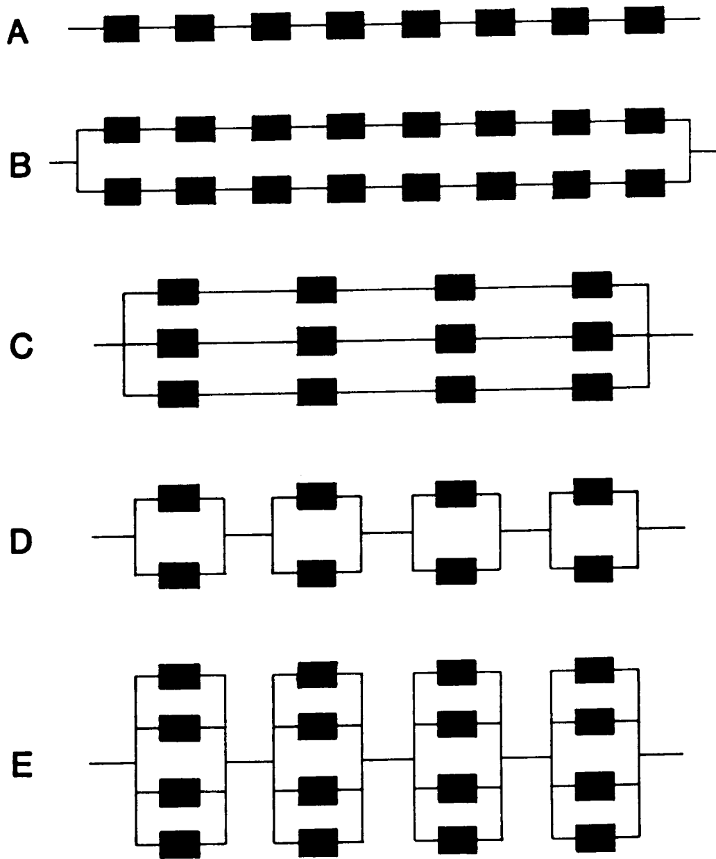
Figure 3. Battery configurations of 8, 12 and 16 cells.
