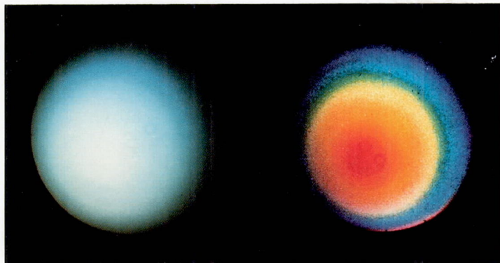
In January 1986, Voyager 2 made its closest encounter with the planet Uranus. It returned never-before-seen close-up views of a planet barely visible from the Earth's surface.
