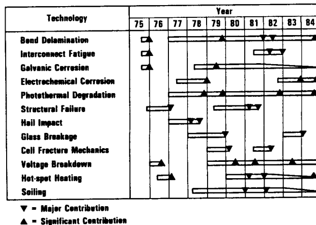
Figure 74. Reliability and Durability Developments, 1975 to 1984
