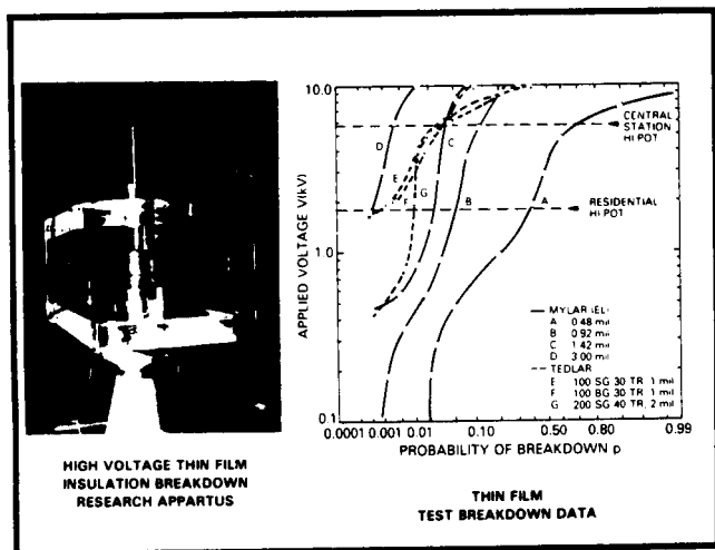
Figure 73. Insulation Breakdown Research
