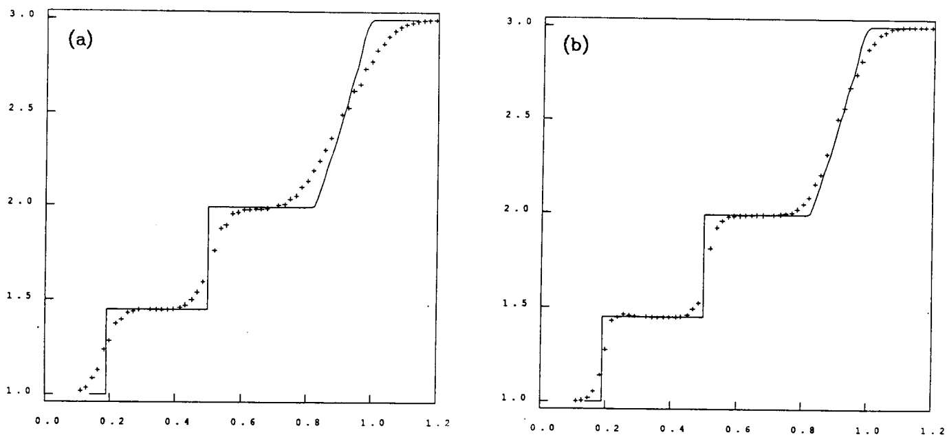
Figure 9.2 Density in the shock tube along the lower wall. Values in the boundary cells are plotted versus arclength. The solid line is the true solution. (a) First order method. (b) With high resolution correction waves included.
