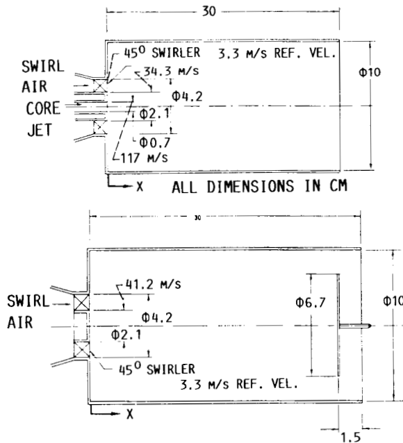
CONFINED SWIRL-DRIVEN FLOW ALTGELD, ET AL (1983)
