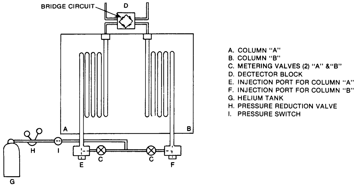
FIGURE 1B. G.C. SYSTEM
