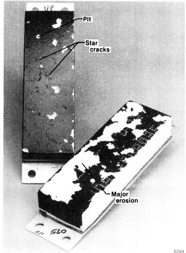
Fig. 12 Examples of the three definable stages of damage to TPS LI900 tiles.
