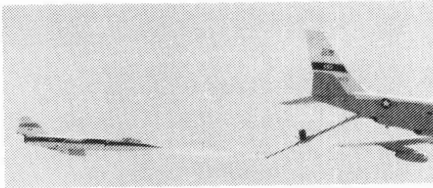
Fig. 8 In-flight photo of USAF KC-135 water spray tanker and F-104 test aircraft.
