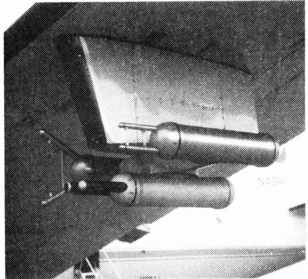
Fig. 6 Three particle measurement probes mounted on the WP-3D left wing tip pylon.
