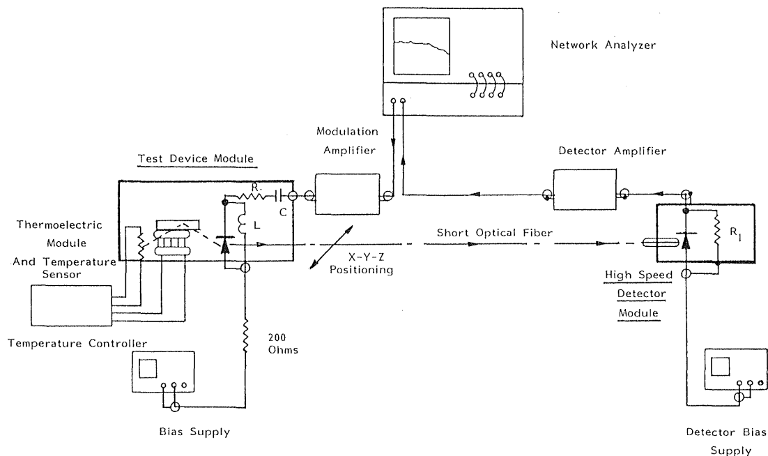
Figure 57. Schematic of the setup used to characterized the frequency response of DFB lasers.
