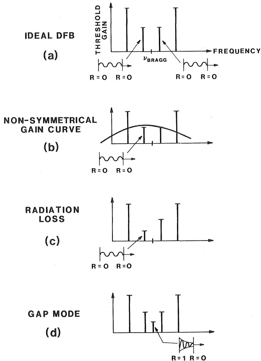
Figure 56. Schematic diagram illustrating the various spectra obtainable from ideal DFB lasers. (The meaning of these figures is explained in the text.)
