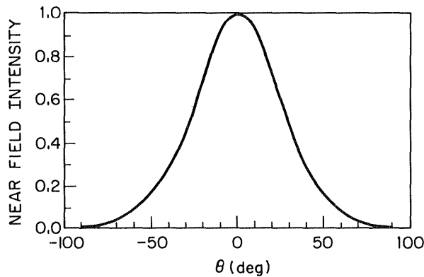
Figure 54. Calculated near-field pattern for structure equal to that measured in Fig. 53.
