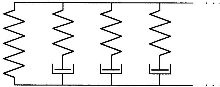
Figure 2. Conceptual schematic of Prony Series material model.
