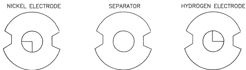
Components for Compression Measurement in Assembly
