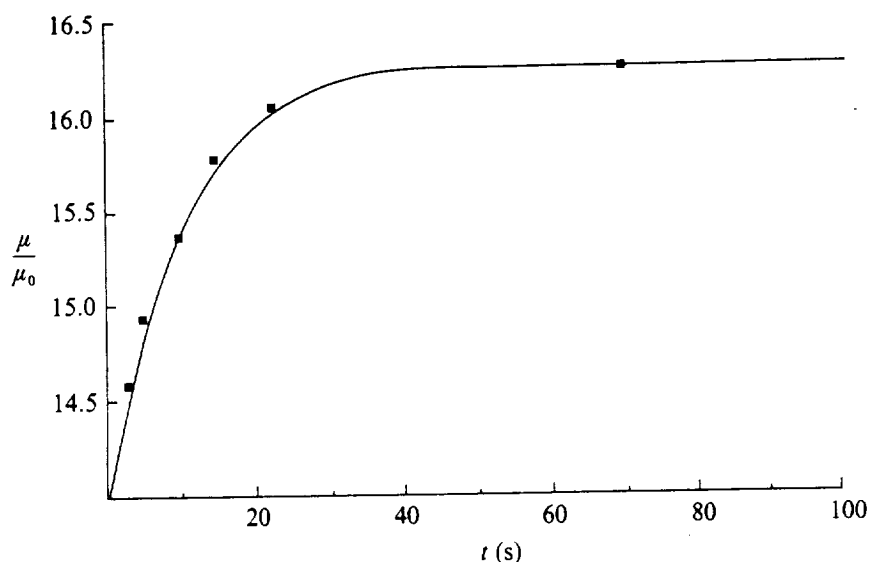
FIGURE 3 Short-term viscosity increase with shearing, 46 \mu\text{m} polystyrene suspension. Model parameters were: \bar{\phi} = 0.45 , \dot{\gamma} = 2.4 \text{ s}^{-1} , \hat{D}_{\parallel} = 1.8 , B_1 = 0.062 .
