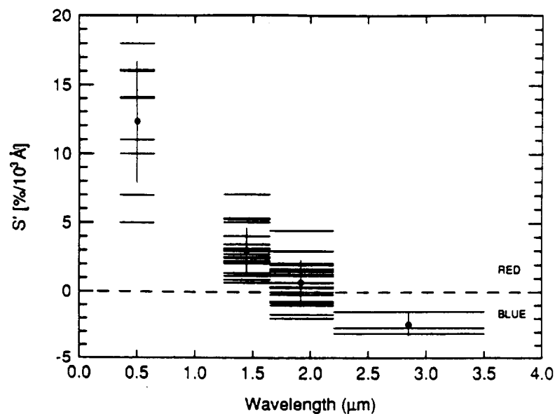
Figure 1. The normalized reflectivity gradient, S'(\lambda_1, \lambda_2) , measured in \% / 10^3 \text{ Å} , is shown as a function of the wavelength of observation \lambda (in \mu\text{m} ). Each comet is represented by a horizontal bar connecting the end point wavelengths \lambda_1 and \lambda_2 . Neutral scattering is indicated by the dashed horizontal line at S'(\lambda_1, \lambda_2) = 0 . Reddening of the scattered radiation is indicated by S' > 0 while enhanced blue scattering is indicated by S' < 0 . The mean S' within each measured wavelength interval is plotted with a black dot and the 1 \sigma standard deviation on the mean is shown with a vertical line. The figure shows that the color of the scattered radiation varies systematically with the wavelength of observation.
