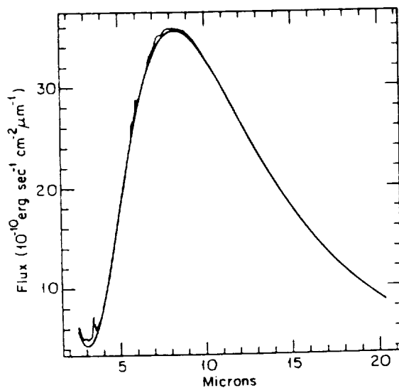
Fig. 3. The Comet Halley 2-20 μm spectrum predicted by our model, compared to that of a 350 K blackbody.
