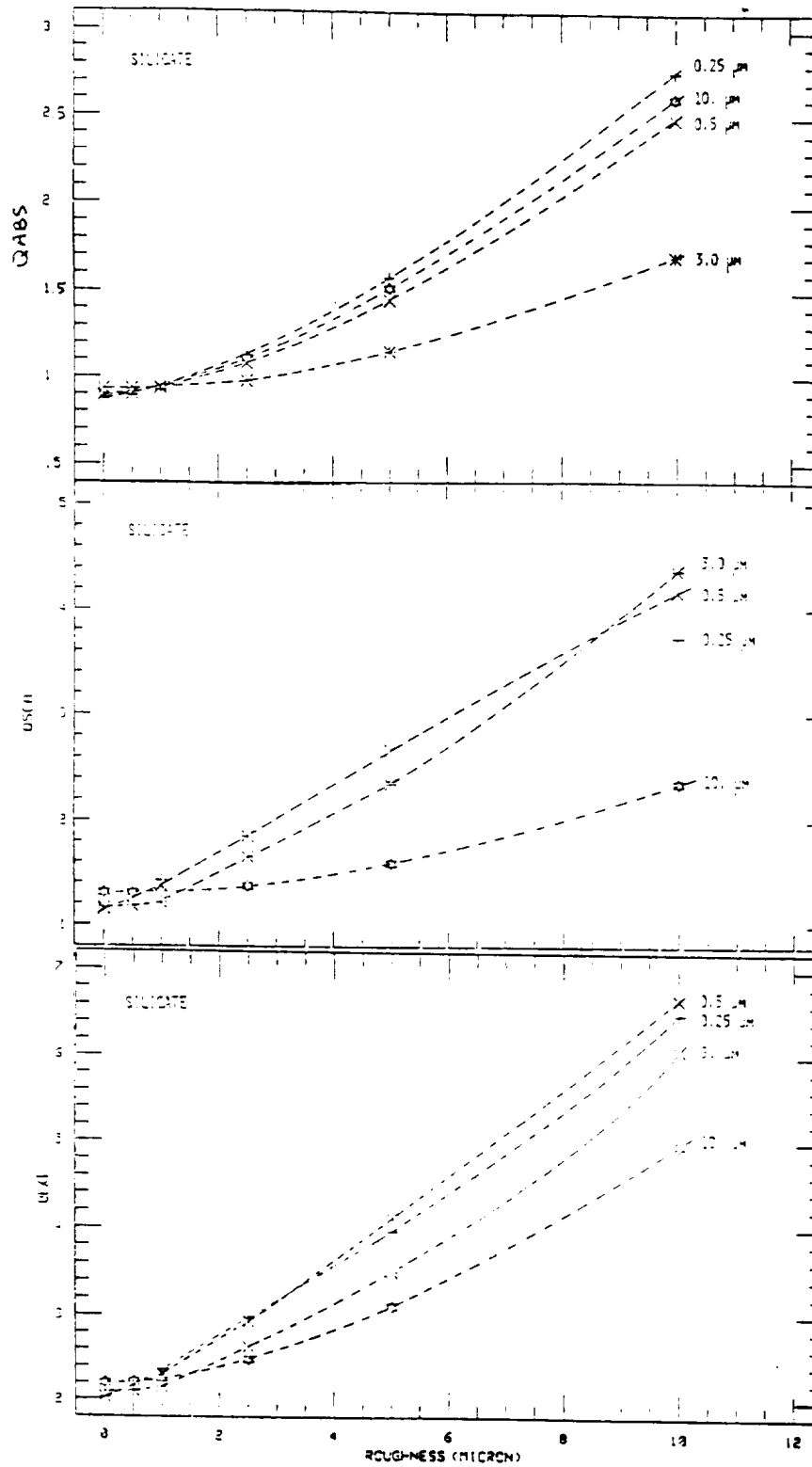
Figure 2.2 - Efficiency factors as a function of roughness for a 50 \mu m silicate particle at various wavelengths (Lamy, abstract this report).
