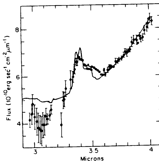
Fig. 2. Best fit (solid curve) to 3-4 μm spectrum of Comet Halley observed by Wickramasinghe & Allen ( Nature 323, 44-46 [1986]). The absorption feature at ~ 3.1 μm, probably O-H stretch, is not modeled.
