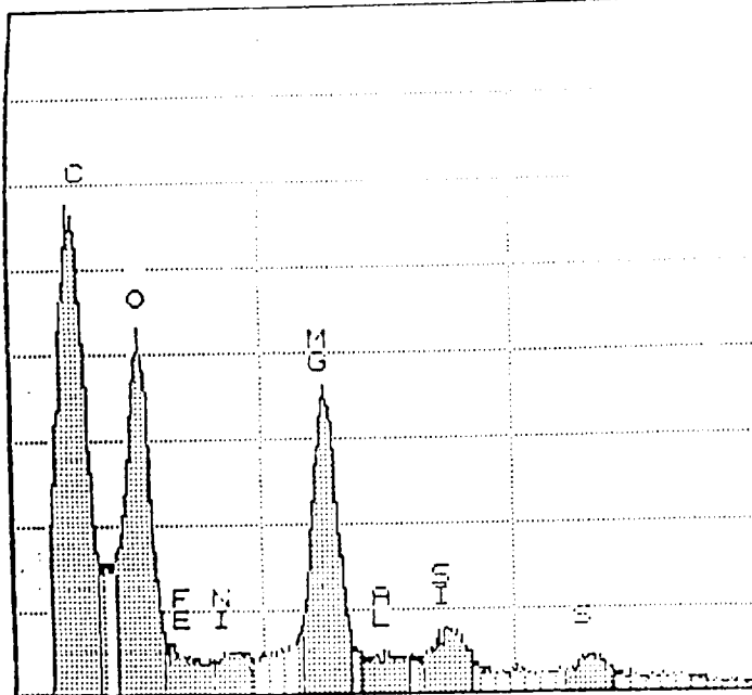
Figure 5: EDX spectrum of a C-rich fragment ( \leq 1 \mu\text{m} in size) of the crushed IDP, Smash (U2033M1), taken with an ultra-thin window detector. In contrast, only an occasional fragment from the carbonaceous meteorites Murchison and Ivuna, shows a discernible C peak.
