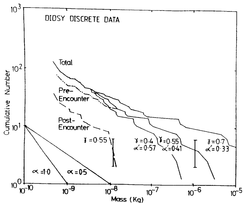
Figure 1. Relative fluence for DIDSY discrete data. The performance limit of the front shield is taken as 3 \times 10^{-6} kg. The different curves correspond to different values of the momentum derating exponent (see text).
