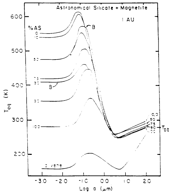
Figure 2.7 - Equilibrium grain temperatures at 1 AU computed for blends of "astronomical" silicate and magnetite, based on Maxwell-Garnett theory and Bruggeman theory (B) (Lien 1987).
