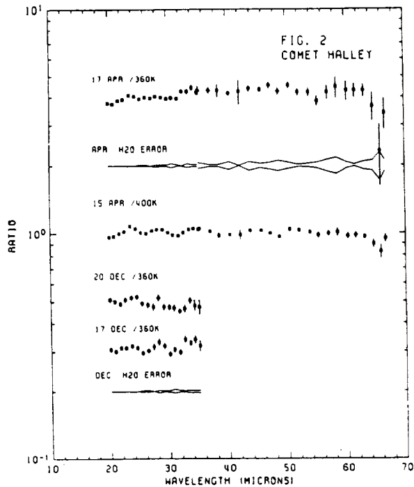
Fig. 2. Spectra of Comet Halley relative to blackbodies. To increase the contrast we have divided each spectrum by a blackbody which fits the overall 20-65 \mu m spectrum. Also shown are the effects on the spectra by a change of \pm 20\% in the ratio of boresight water vapor on the comet and calibration legs. The data for the April flights is the same as in Fig. 1. For the December flights we have used a different calibration procedure. The comet data are calibrated to \alpha Ori assuming it has a smooth spectrum and using values for water vapor from the on-board radiometers. The 28 \mu m feature appears as a 9.5% \pm 3.8% excess in one channel; to remove it by adjusting water vapor requires a change by a factor of 3 in the ratio of boresight water vapor (as measured by the on-board radiometers) on the comet leg and the \alpha Ori leg. Such a large error in the values obtained by the water vapor radiometers is unlikely, as this ratio has a standard error of 25% for the 5 other objects on the flight. If we assume that we can determine the ratio to \pm 10\% on those objects by removing the water lines. The 25% standard error is typical. We cannot rule out the possibility of the feature being due to a change in sensitivity of that detector during the flight, but such changes are rare and have never been seen in that channel, and nothing was unusual about any other objects on that flight either before or after the comet.
