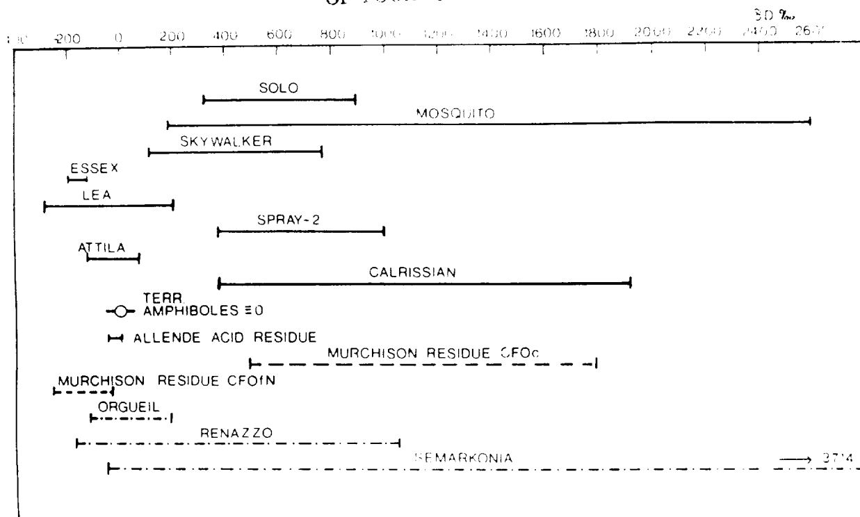
Figure 1: \delta D values for several IDPs. The horizontal lines show the full range of measured values for different fragments of a given particle. Since the measurement errors are \leq 200\text{‰} , the large spread shows that the deuterium enrichments are inhomogeneously distributed. Data are taken from McKeegan et al. (1985). Similar data for meteorites are shown on bottom.
