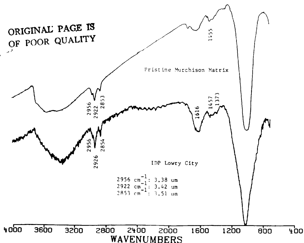
Figure 3: Infrared absorption of the IDP, Lowry City, as measured by Fourier transform microspectrometry. In addition to the typical major 10\ \mu\text{m} feature identifying this particle as a layer-lattice silicate type, there is a prominent triplet at 3.4\ \mu\text{m} . Data from Swan et al. (1987).
