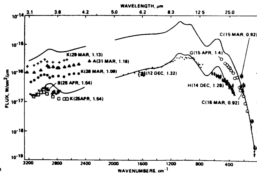
Figure 2. Comparison of the calculated and observed infrared emission from 3 to 160\mu\text{m} for Comet Halley. The solid curves are for r=1.32 and 0.92 AU with \alpha=-3.5 and X=40 . The observational data are from the numbered and lettered references in the reference list.
