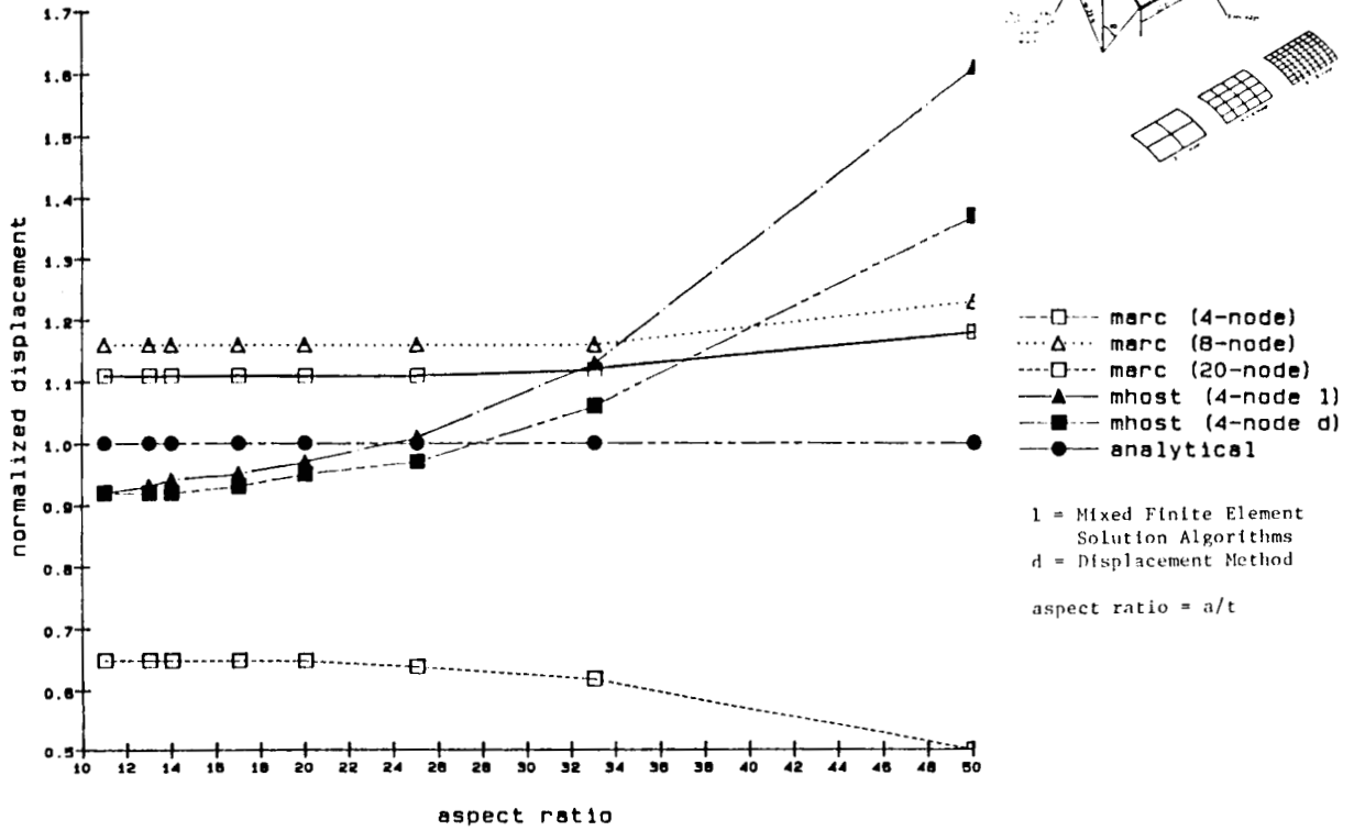
Figure 1 Displacement of Center for Cylindrical Shell Roof
