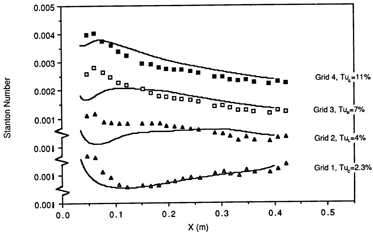
FIGURE 5 Comparison of the calculations with the data from case 6 of Rued
