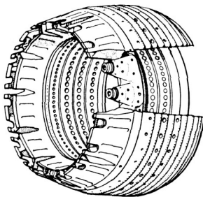
COMBUSTOR LINER
