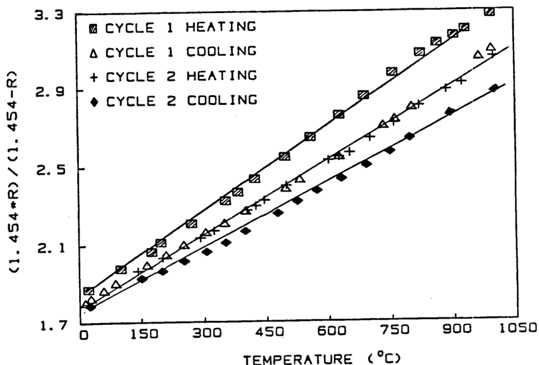
Fig. 17. (R_{\text{max}} \times R) / (R_{\text{max}} - R) vs. temperature for ZrC. R_{\text{max}} = 1.454 ohm corresponds to \text{max} = 1000 microhm-cm.
