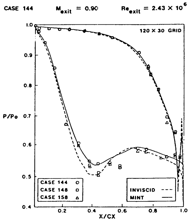
Fig. 2 Pressure Coefficient Distribution.
