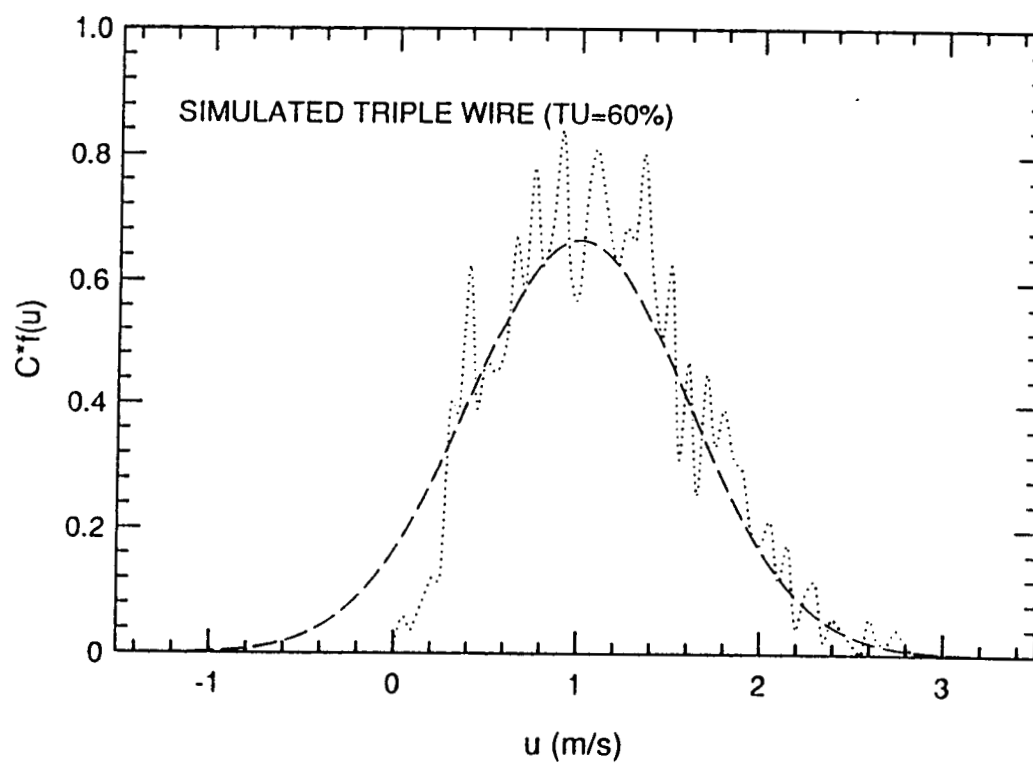
Figure 10 u-component velocity pdf for simulated triple wire.
