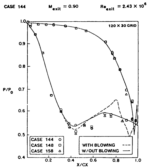
Fig. 4 Pressure Coefficient Distribution.
