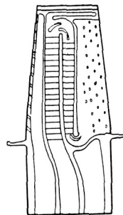
TURBINE BLADE
