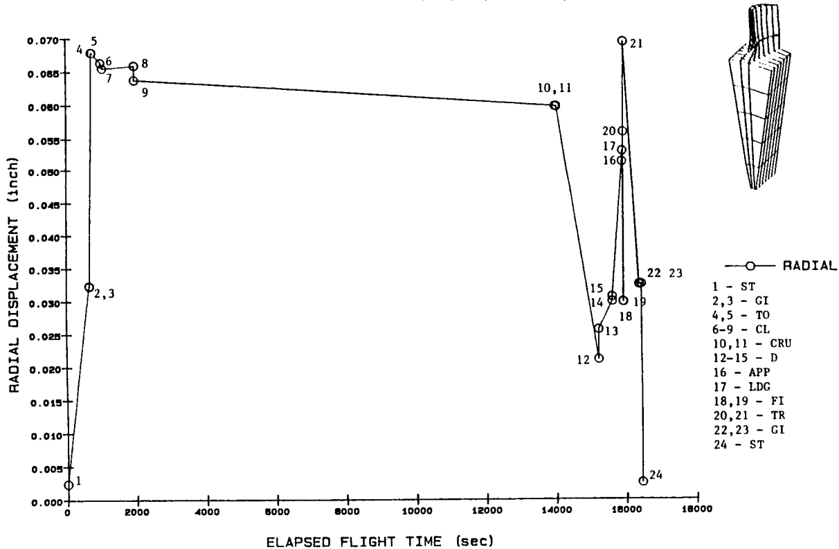
Figure 4 Radial Displacement of Leading Edge Tip ( Static )
