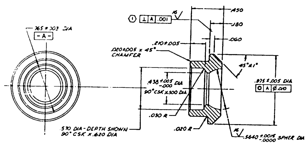
Figure 4. Double swivel toggle components.
