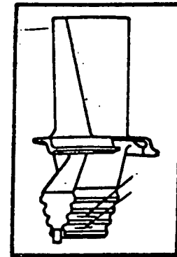
(h) TRANSVERSE FIR TREE LOBE
