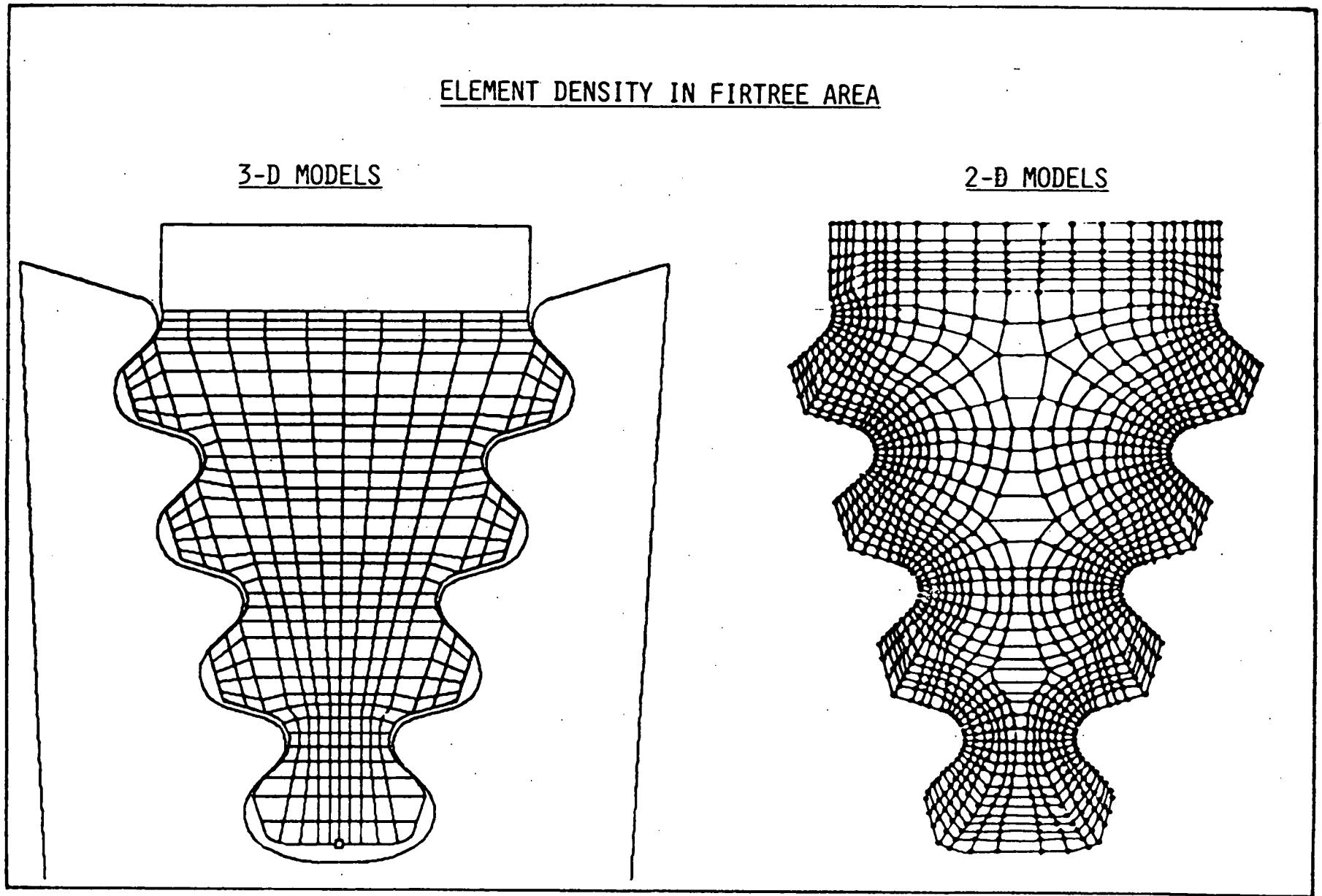
Figure 12. 2D and 3D fir tree element density.
