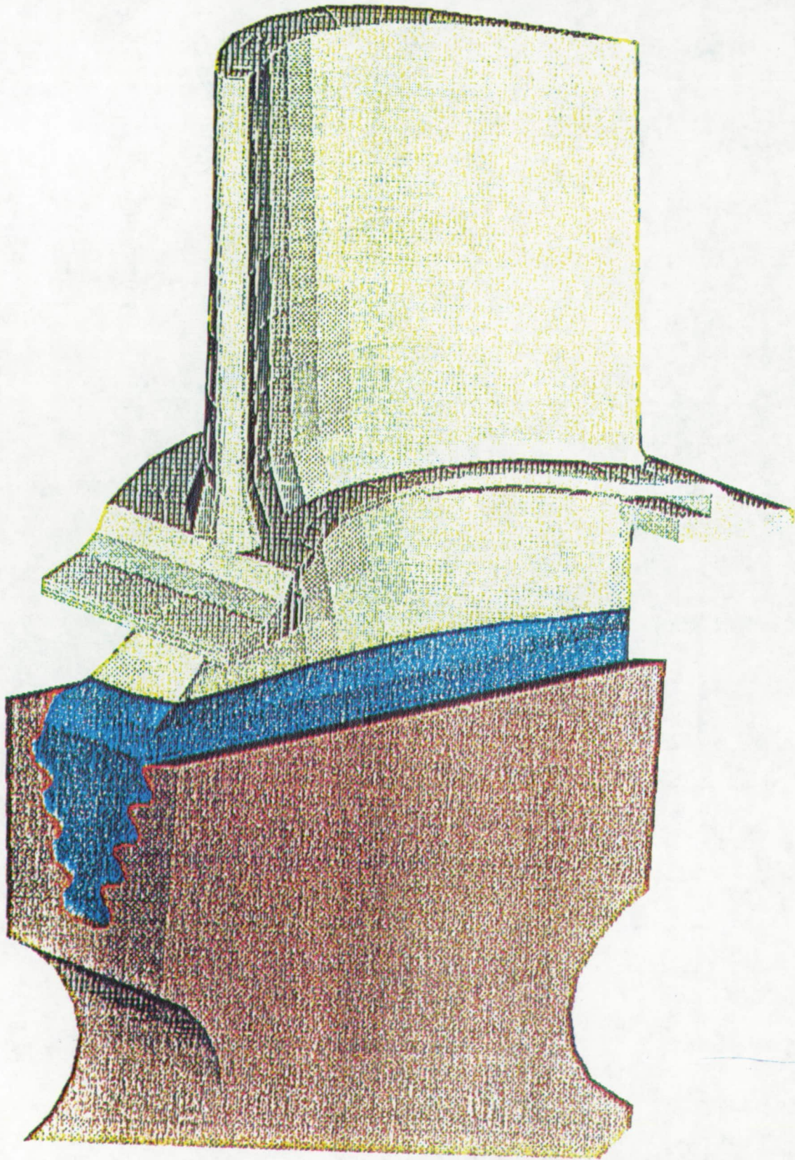
Figure 15. Blade/rotor attachment region.
