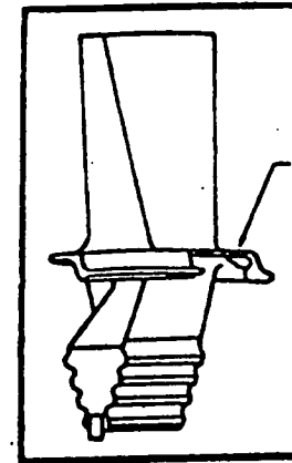
(c) CRYSTALLOGRAPHIC PLATFORM
