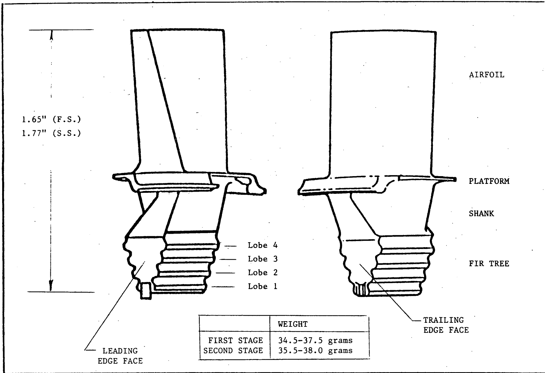
Figure 2. First- and second-stage blades.
