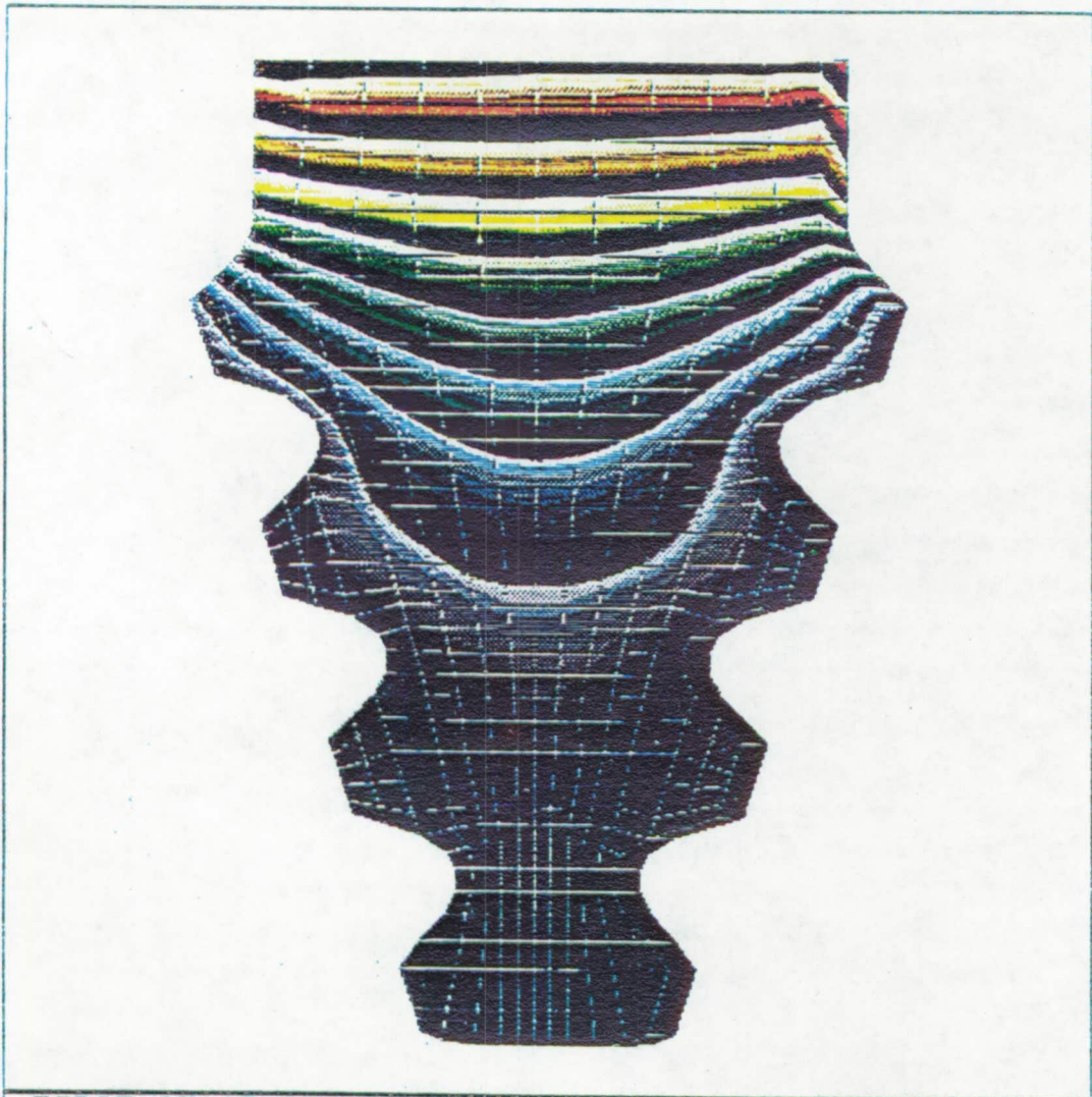
FIRST STAGE FIR TREE W/DISK- FACE 15(CENTER)
