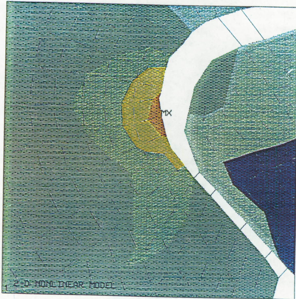
Figure 21. First-stage 2D strain contour.
