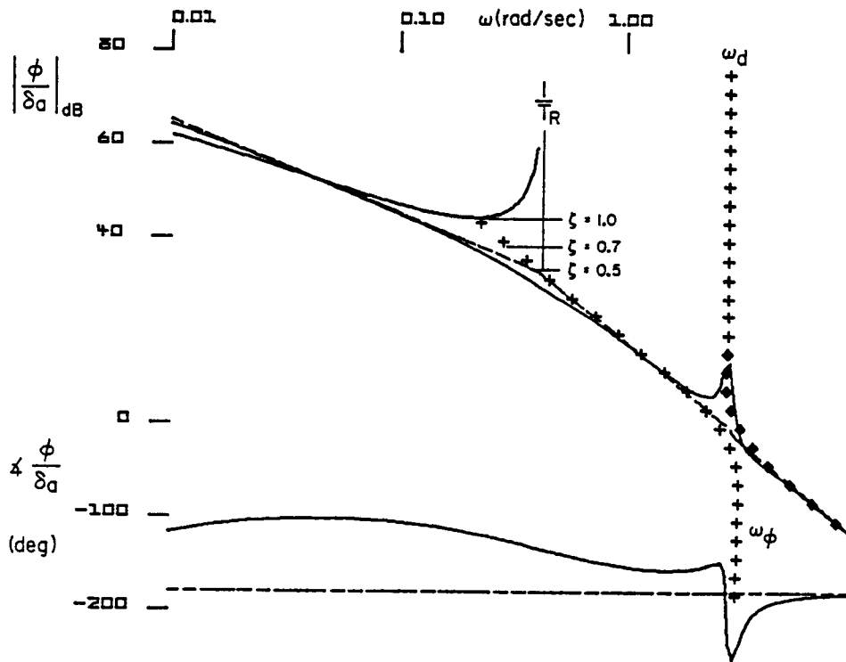
b) j\omega -Bode and Bode Root Locus
