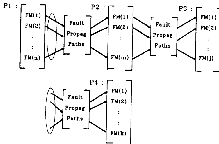
Figure 5. Fault Propagation Digraph of a Process
