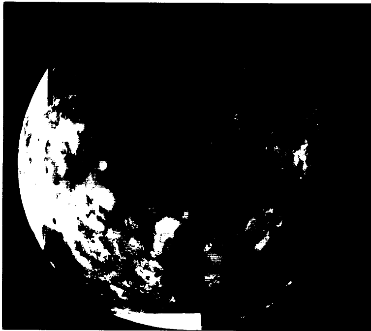
Voyager 1 and 2 photographs of Jupiter and its moon Io. Above, the violent weather patterns that constantly swirl around the edges of the Great Red Spot, the huge storm which is larger than Earth. Below, the vivid surface of Io, punctured with volcanoes and stained with their flow.
