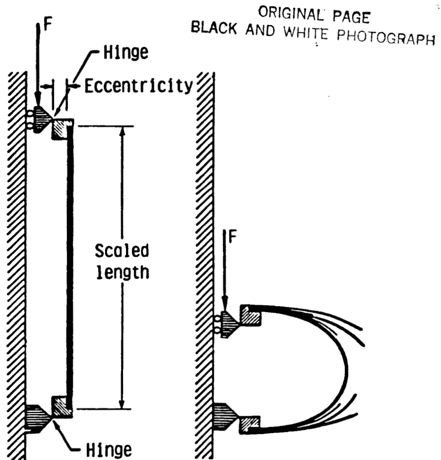
Figure 2. Schematic drawing of the test configuration.
