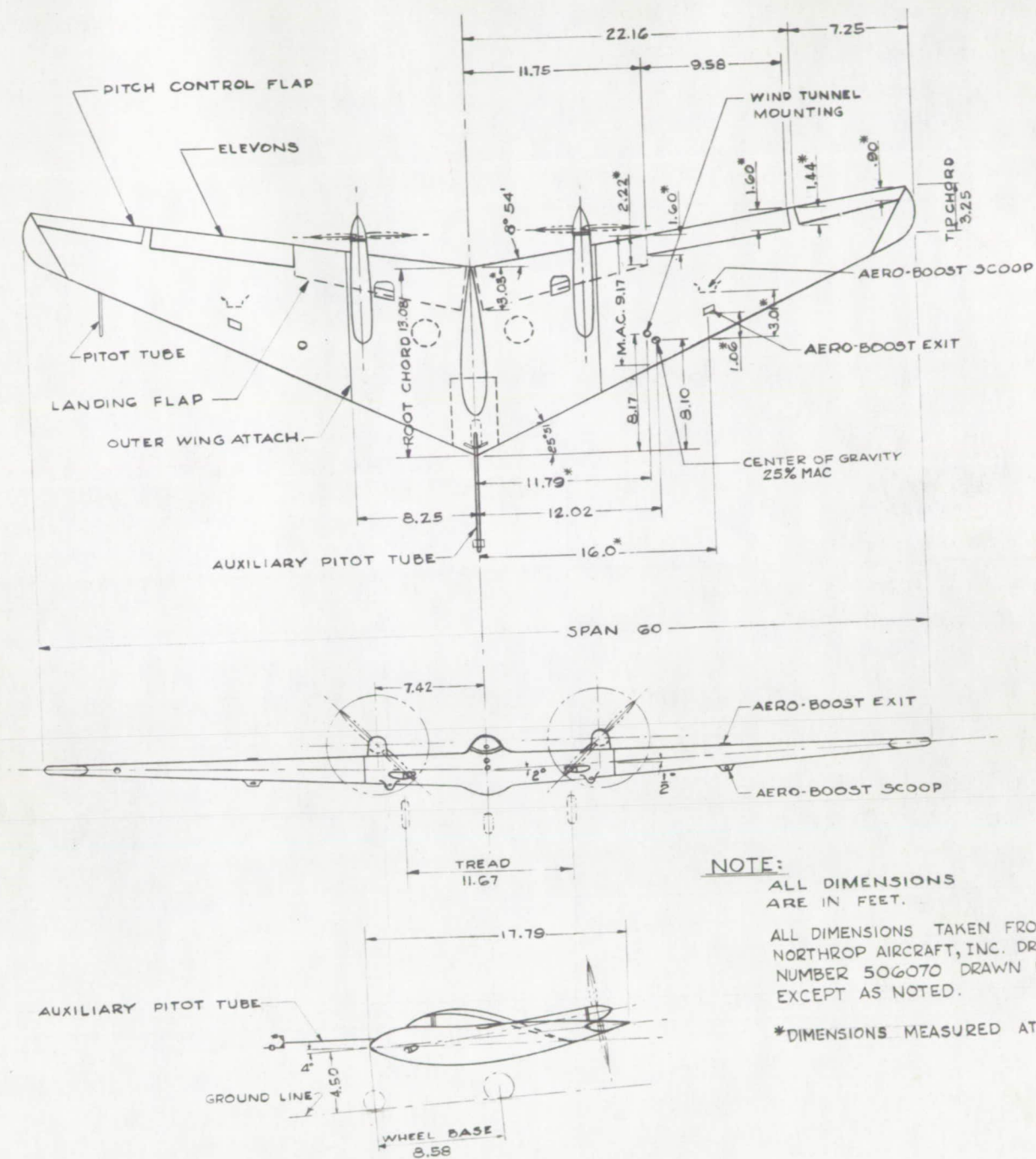
FIGURE 1. - THREE-VIEW DRAWING OF NORTHROP N9M-2 AIRPLANE
