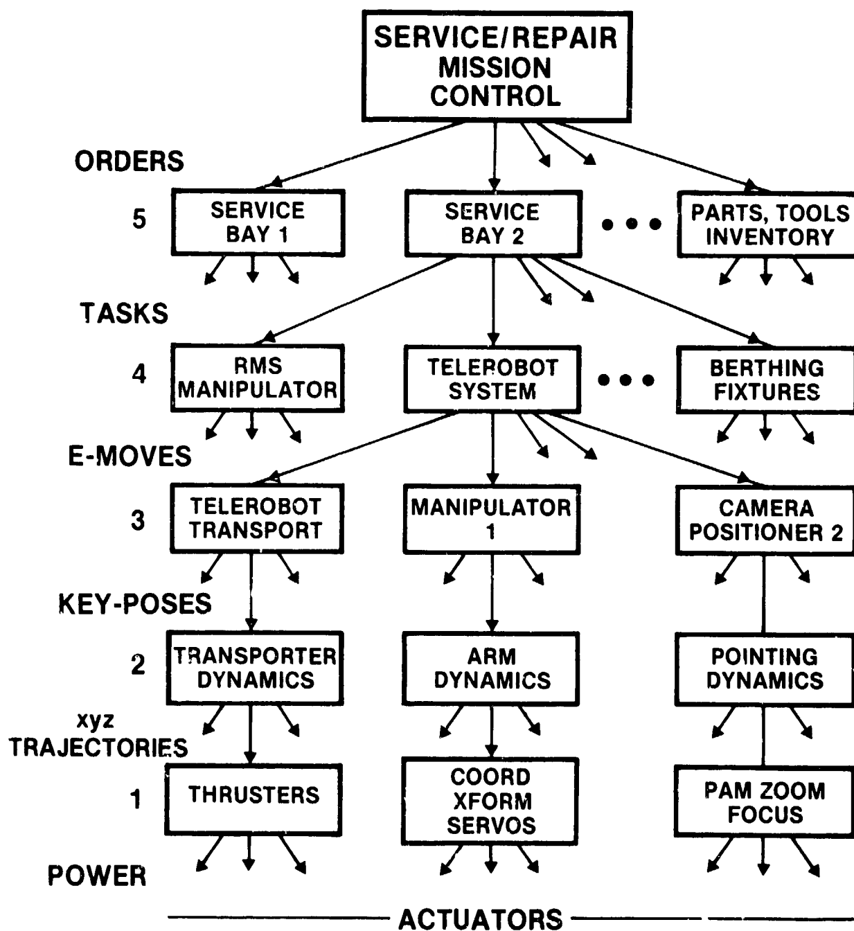
FIGURE 8: A six level hierarchical control system proposed for telerobots.
