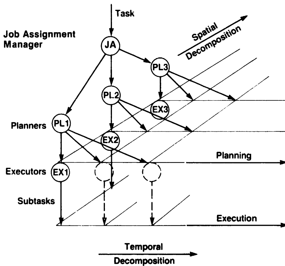
FIGURE 2: The job assignment JA performs a spatial decomposition of the task. The planners pl (j) and executors EX (j) perform a temporal decomposition.
