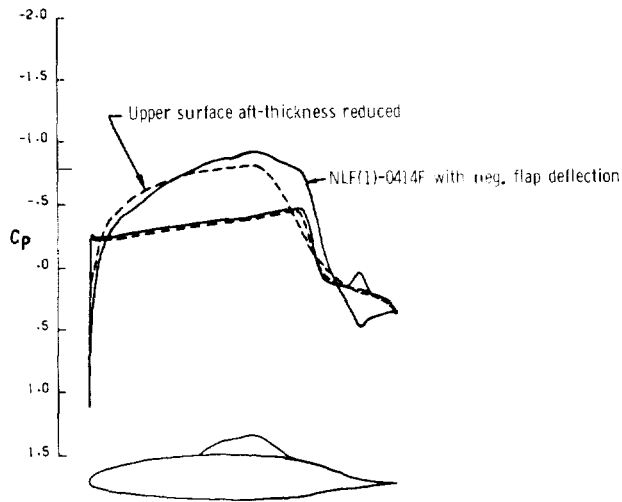
HSNLF(1)-0213 AIRFOIL DESIGN PRESSURE DISTRIBUTION ( M = 0.7 )
