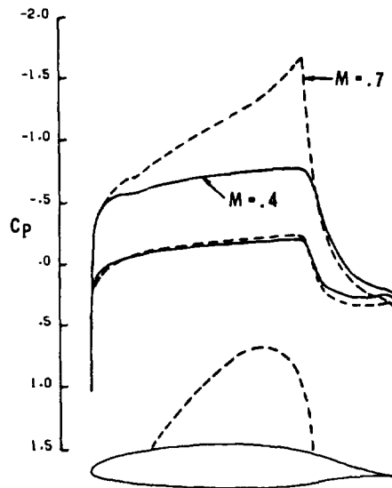
EFFECT OF MACH NUMBER ON PRESSURE DISTRIBUTION OF NLF(1)-0414F
