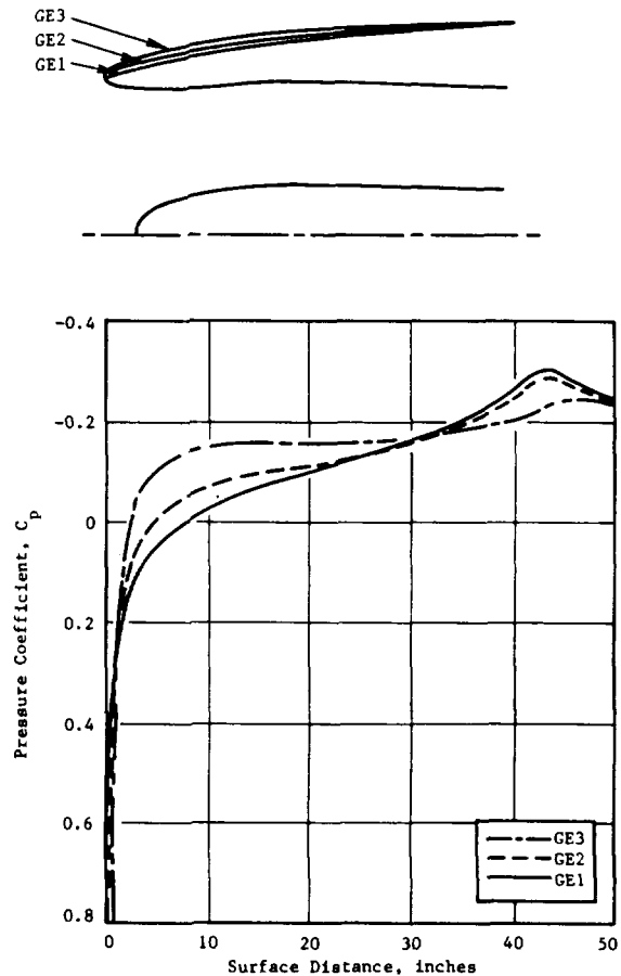
Pressure Distributions
