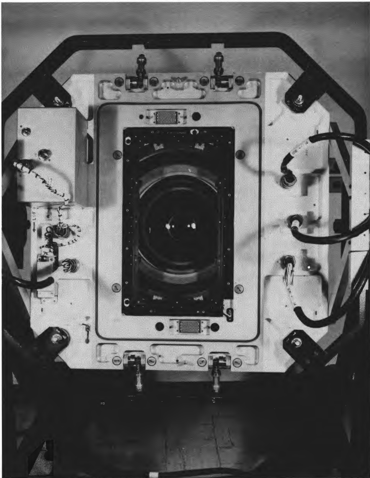
Figure 1-7.- The aft end of the LFC lens assembly. Shown are the format mask, the rear lens elements, the film magazine attach points, and the electrical connector interfaces (NASA photo S81-31664).
