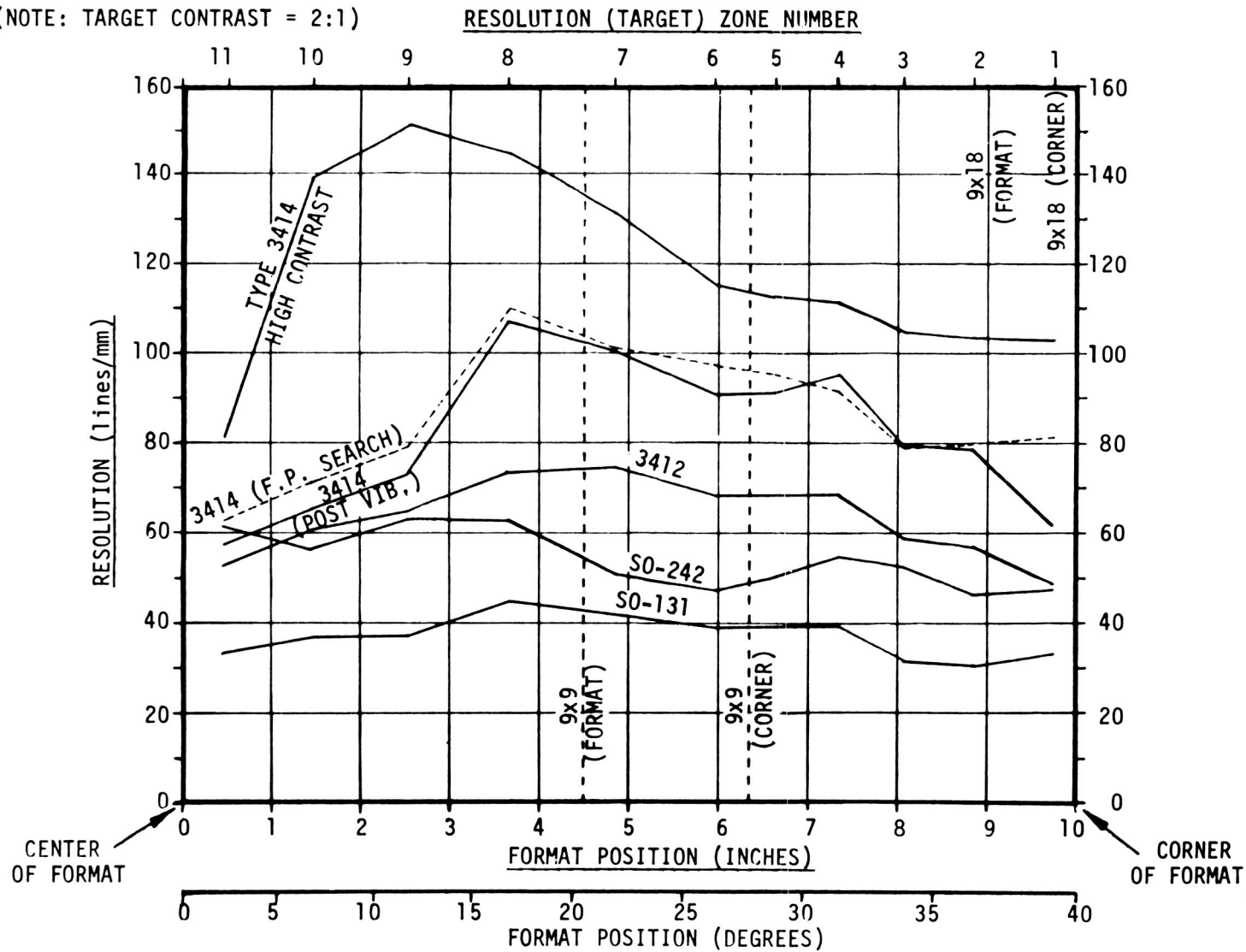
Figure A-8.- Static resolution of the LFC lens assembly. Plotted as a function of field position using the center of the frame format at the point of origin.
