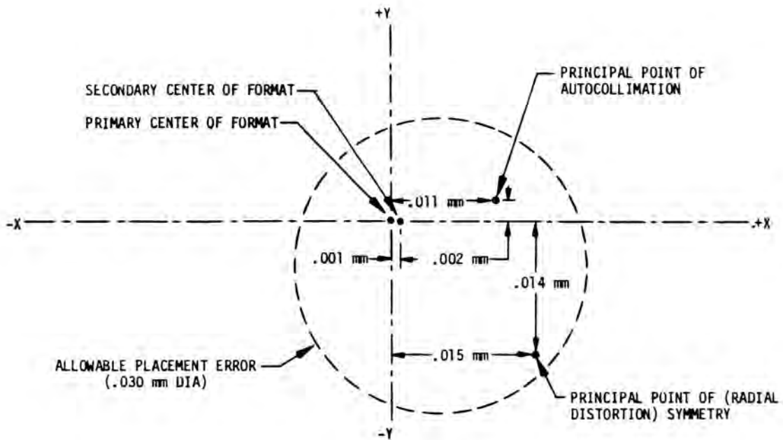
Figure A-6.- Coordinates for the geometric centers of the LFC cartographic lens assembly, serial number (S/N) 001.
