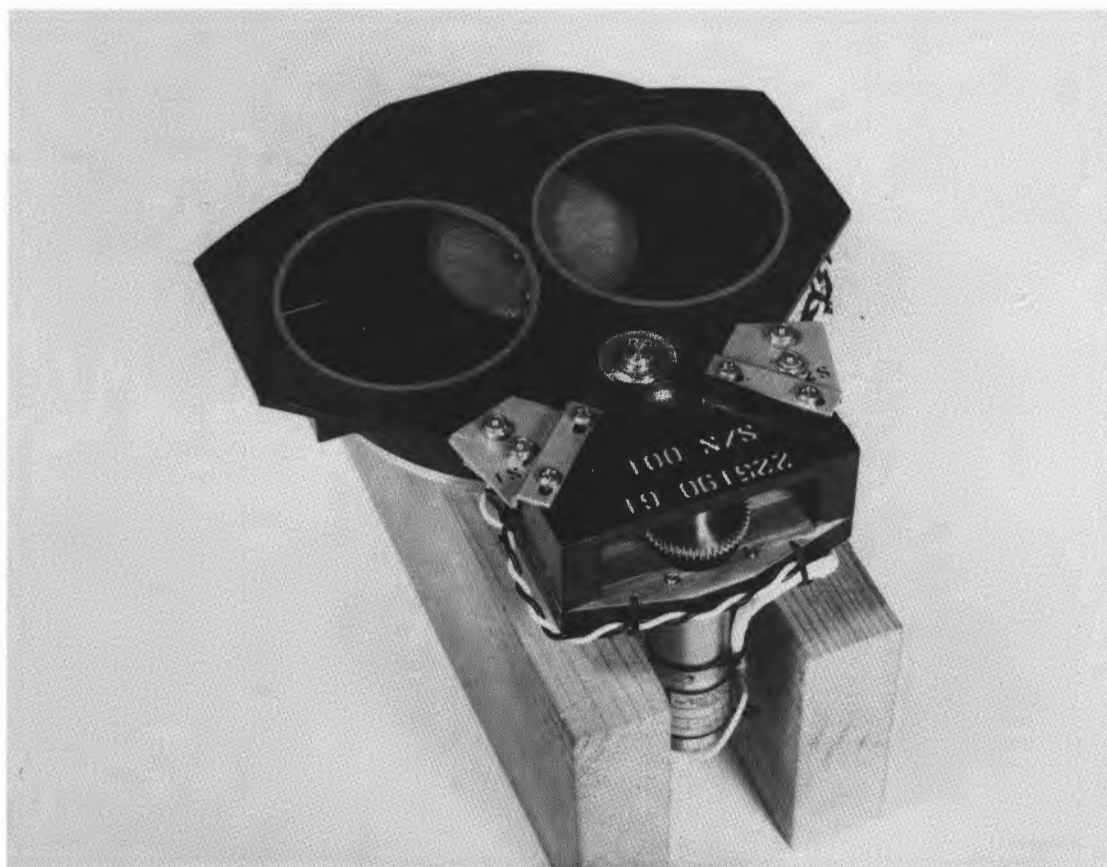
Figure 1-11.- The filter holder and drive mechanism. Shown stopped at a point halfway between the two select positions; view is prior to installation of the two spectral filters (NASA photo 80-26243).
