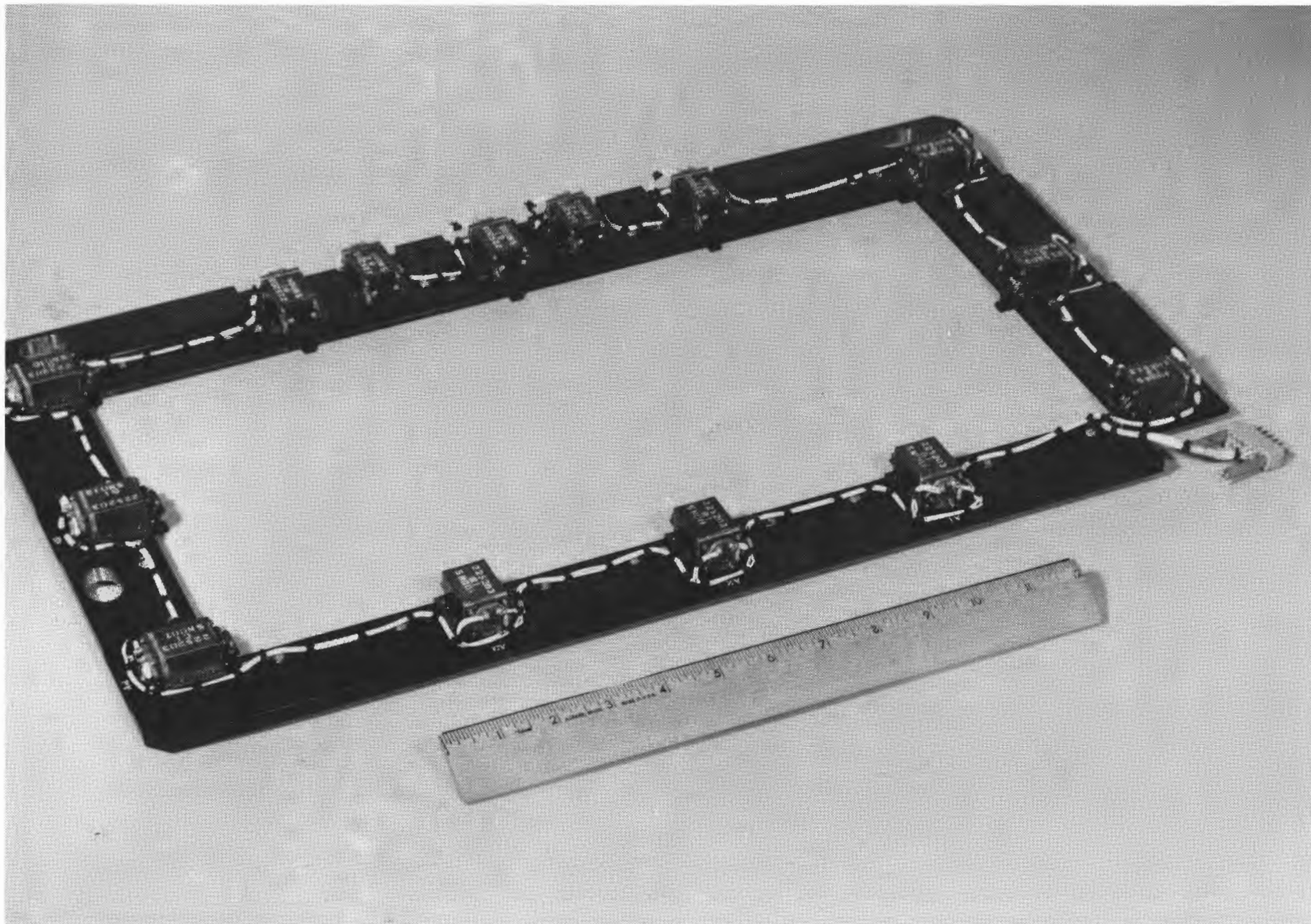
Figure 1-13.- The under side of the LFC focal frame prior to assembly. Shown are the 12 fiducial projectors (A), the 2 lens serial number projectors (B), and the film magazine serial number illuminations (C). (NASA photo S80-26270.)
