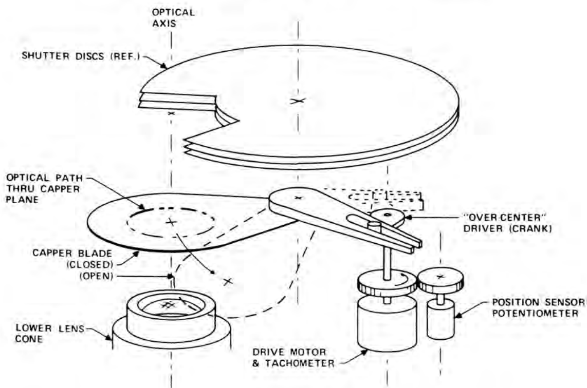
Figure 1-9.- Schematic presentation of the LFC capping shutter action.
