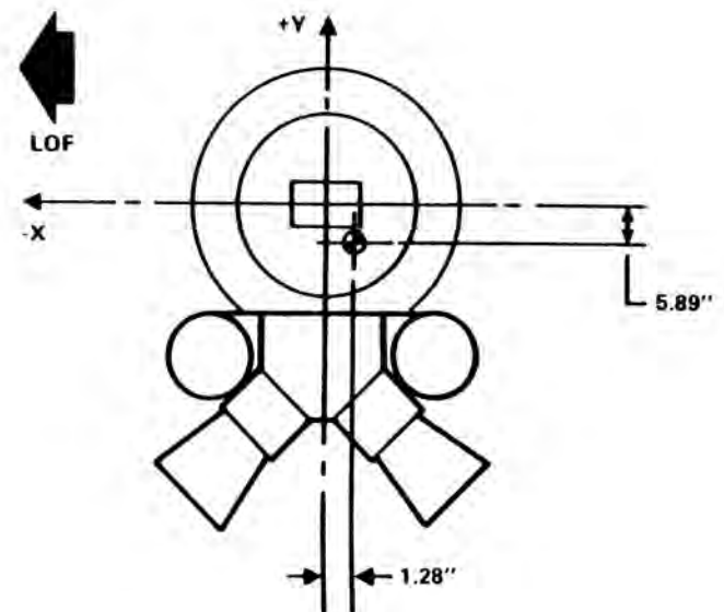
Figure 2-9.- Mounting options for attachment of the SCA to a constant LOF of the LFC.
