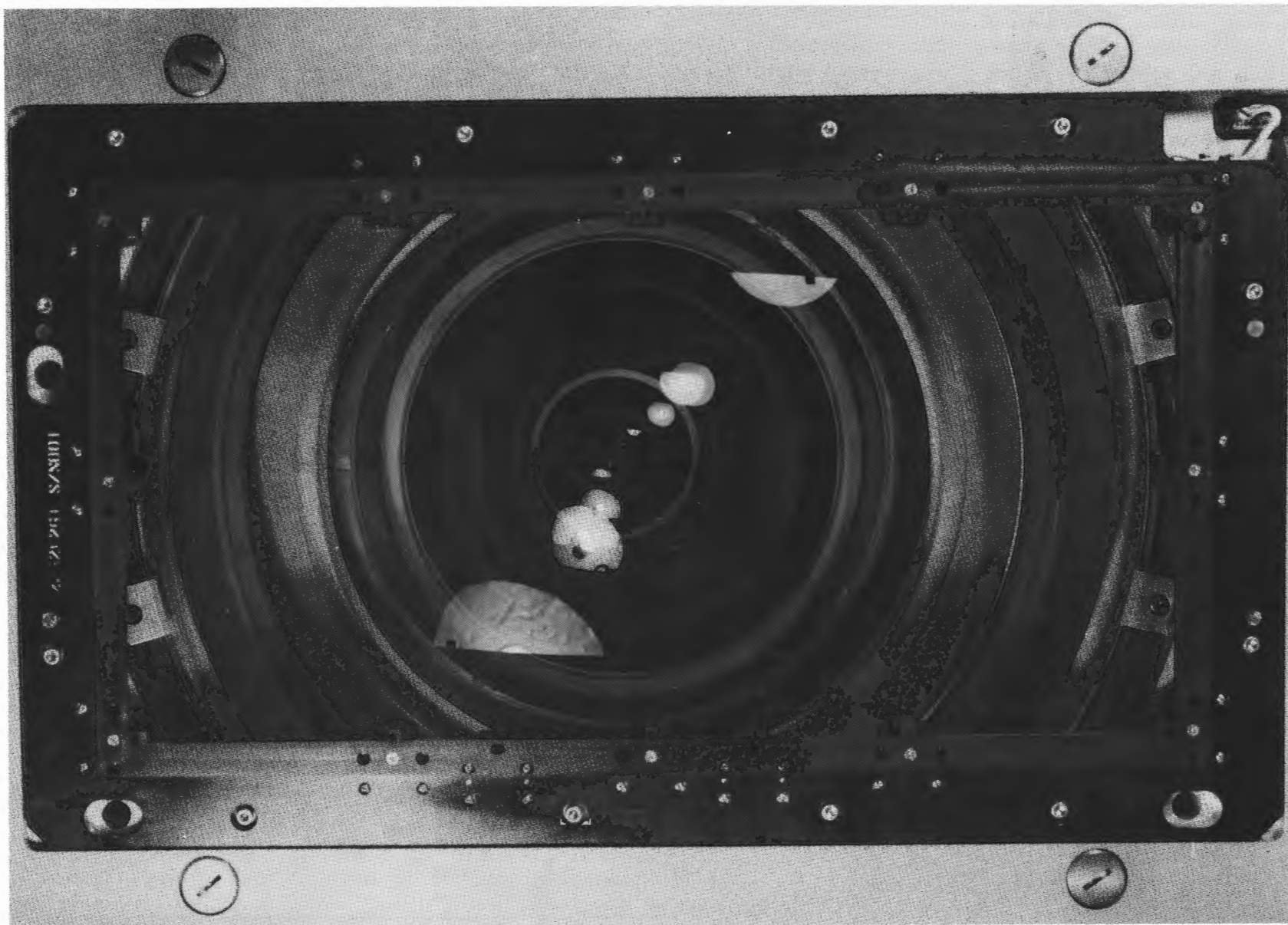
Figure 1-12.- The LFC focal frame. Shown attached to the camera support structure (NASA photo S81-31659).
