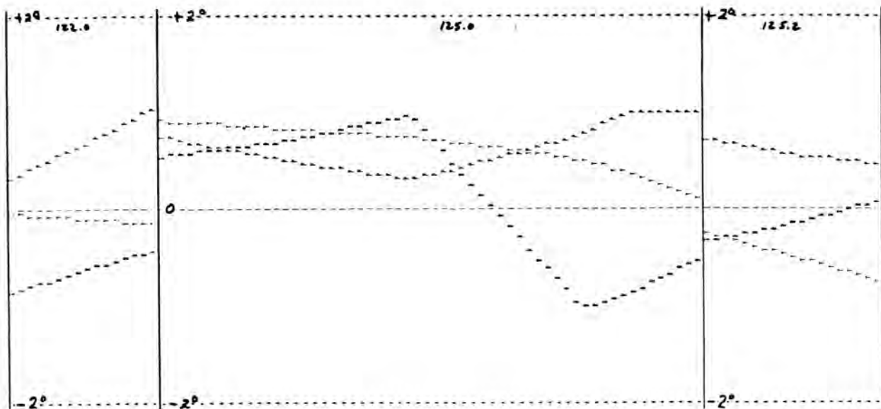
Figure 2-10.- Roll, pitch, and yaw deadband with the crew awake and performing onboard activities – data pass 125.0. (Sampled at 10-sec intervals.)
