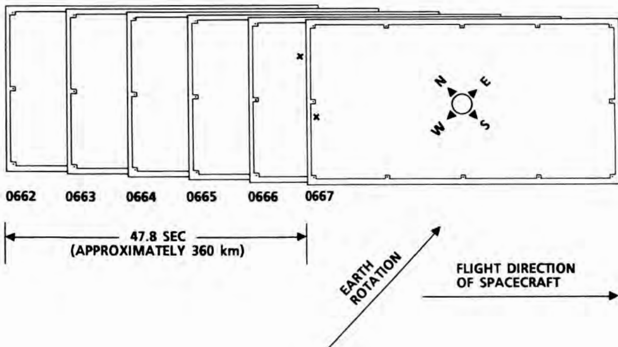
Figure 1-21.- Image point drift. Figure shows drift across a format area on successive frames, at 80-percent forward O/L, due to the easterly rotation of the earth (top), and the effect of successive frame offset due to this rotation (bottom).
