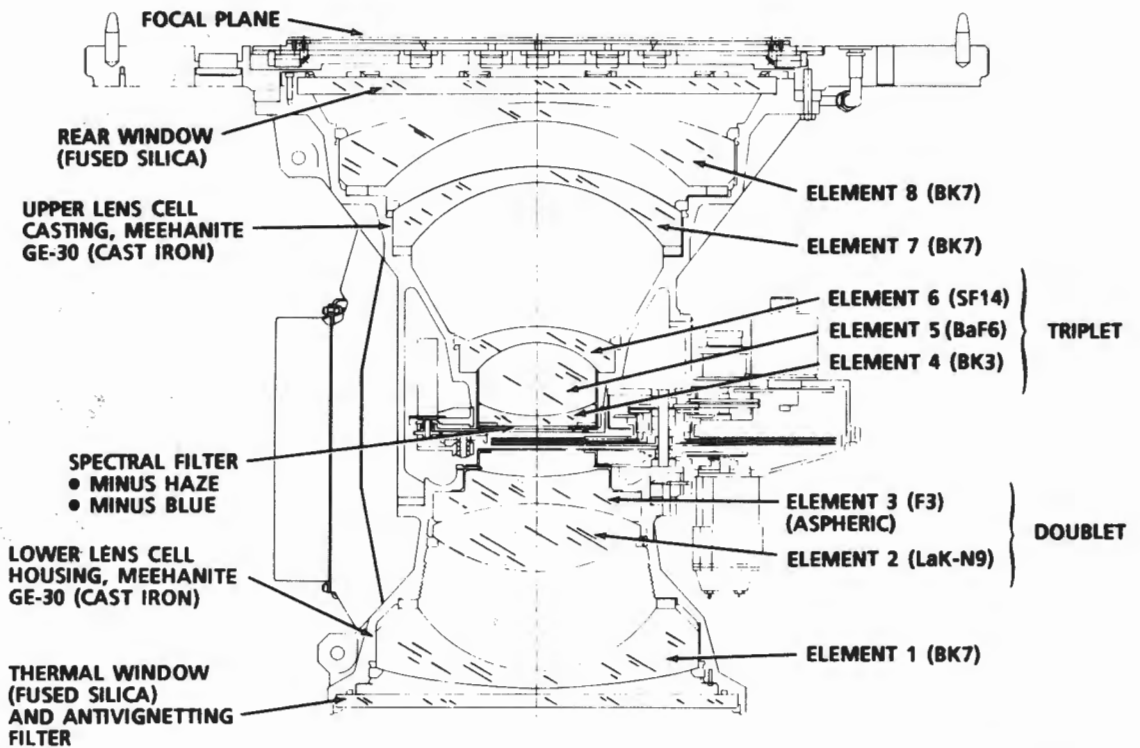
Figure 1-4.- Schematic of the LFC cartographic lens assembly. This schematic shows the types of glass used for manufacture of the individual lens elements.
