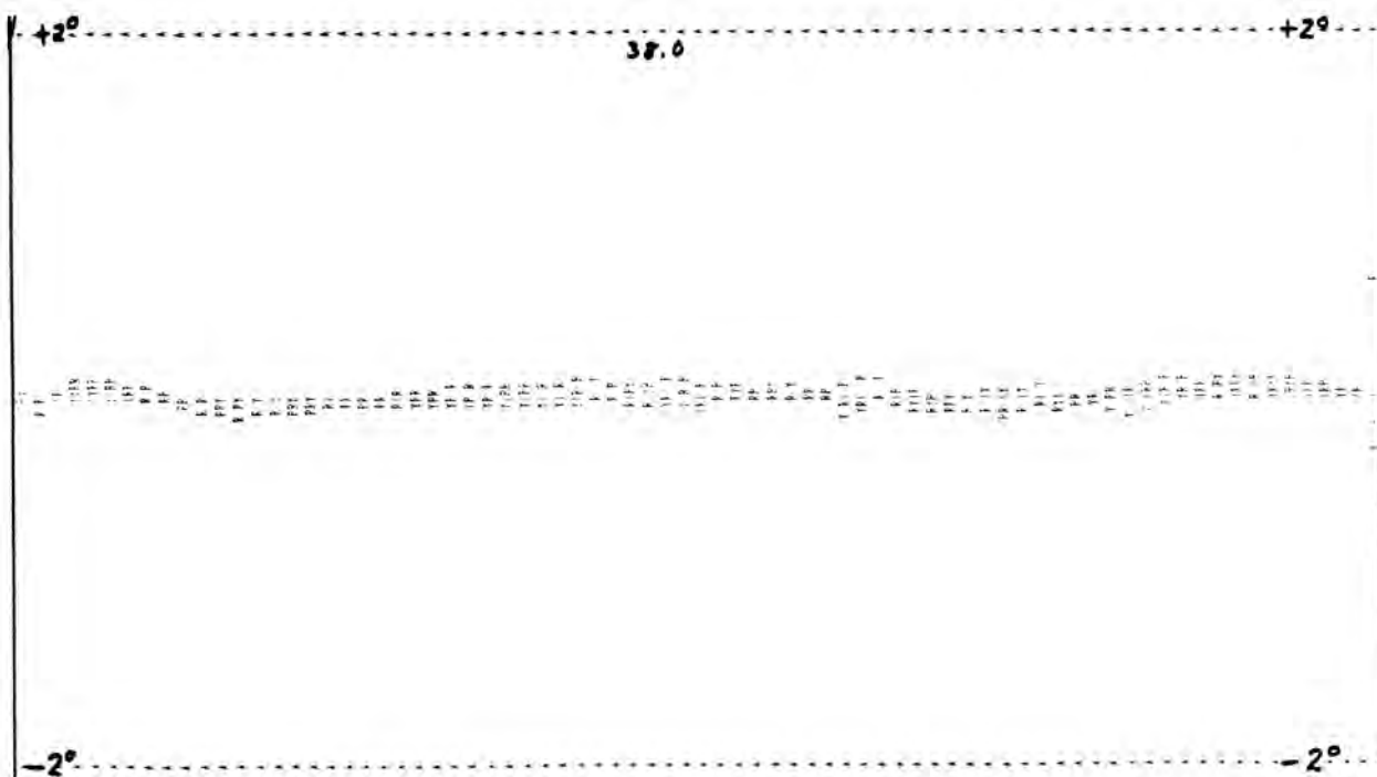
Figure 2-11.- Roll, pitch, and yaw deadband maintenance during crew sleep period – data pass 38.0. (Sampled at 10-sec intervals.)
