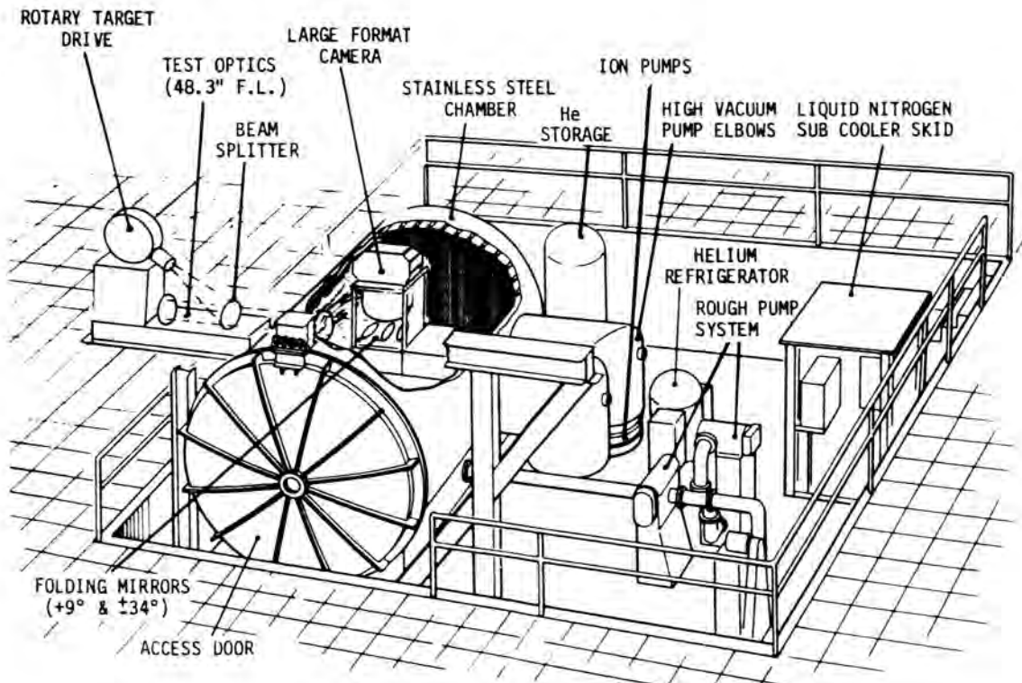
Figure A-7.- Thermal vacuum and dynamic resolution test chamber.
