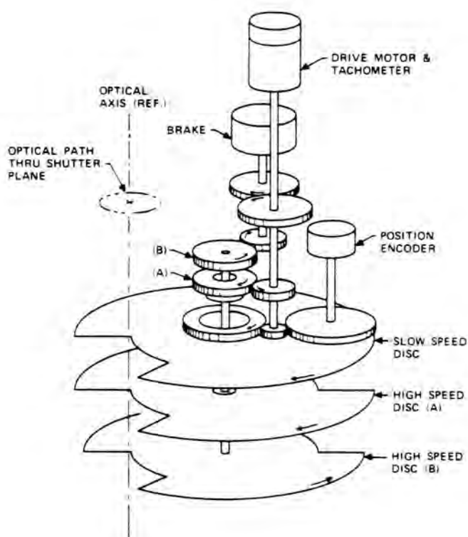
Figure 1-8.- Schematic layout for the LFC rotary shutter blades.
