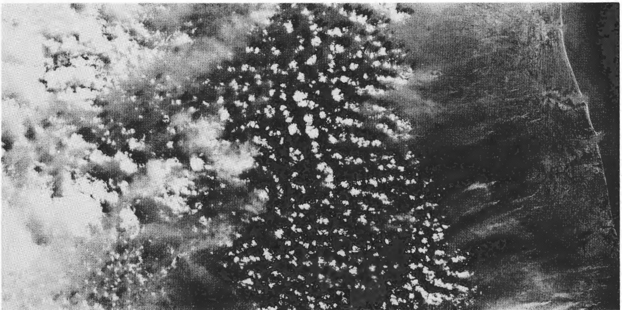
Figure 3-110. - Major thunderstorms in the making over the southeastern coast of Africa at Quelimane, Mozambique. Smoke plumes from burning fields indicate the direction of strong winds offshore, where ocean moisture forms clouds which increase in size and severity as they move inland. Frame 1429, orbit 66 (GMT 283:1312), altitude 226.57 km, type 3414 film. Original scale 1:743,000 (shown at 1:2,124,000). Area covered is 25,700 sq km. Spacecraft nadir coordinates are 17.18°S 36.02°E.
