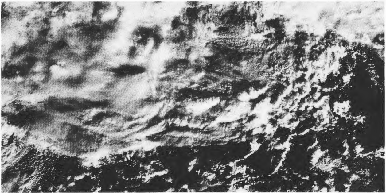
Figure 3-107.- Cloud formations over the Bering Sea at about the Near Islands of the Aleutians. Low sun elevation emphasizes both cloud structure and elevations. Frame 0302, acquired orbit 23 (GMT 280:2050:12), altitude 269.34 km, type 3414 film. Original scale 1:884,000 (shown at 1:2,526,000). Area covered is 36,300 sq km. Spacecraft nadir coordinates are 53.19° N 165.32° E.
