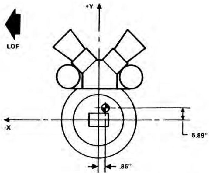
Figure 2-9.- Mounting options for attachment of the SCA to a constant LOF of the LFC.
