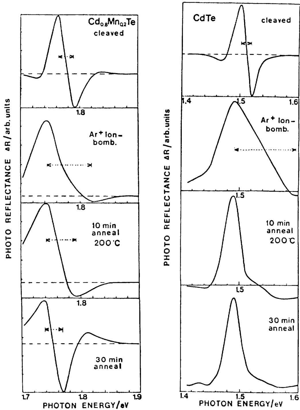
Figure 5. Line broadening and recovery of the photorefectance signal after radiation damage and annealing of \text{CdTe} and \text{Cd}_{1-x}\text{Mn}_x\text{Te}
