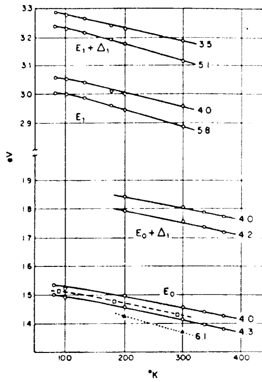
Figure 3. Positions of the interband transitions of GaAs where \nabla_k(E_c - E_v) = 0 (top) and temperature dependence of these transitions determined by modulation spectroscopy (bottom) 8 .
