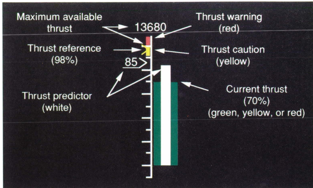
Figure 6. Thrust indicator.
