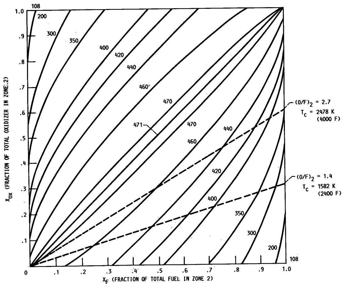
FIGURE 3. - CONTOURS OF ODK VACUUM SPECIFIC IMPULSE AS DETERMINED BY A 2-ZONE ANALYSIS OF AN H 2 O THRUSTER. (O/F)_T = 4.5 , P_c = 500 PSIA AREA RATIO 40:1.
