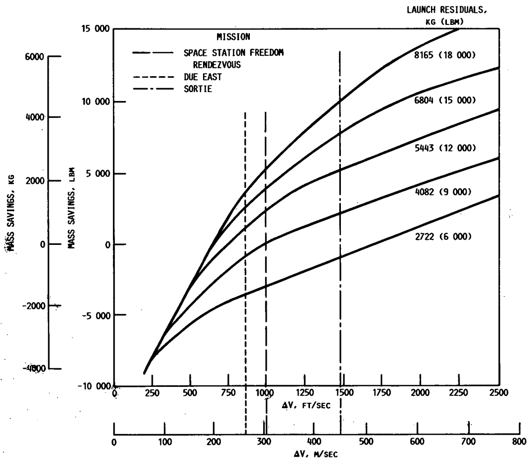
FIGURE 5. - PROJECTED MASS SAVINGS GAINED BY USING INTEGRATED H/O AUXILIARY PROPULSION INSTEAD OF STATE-OF-THE-ART AUXILIARY PROPULSION WITH UPRATED OMS ENGINES.
