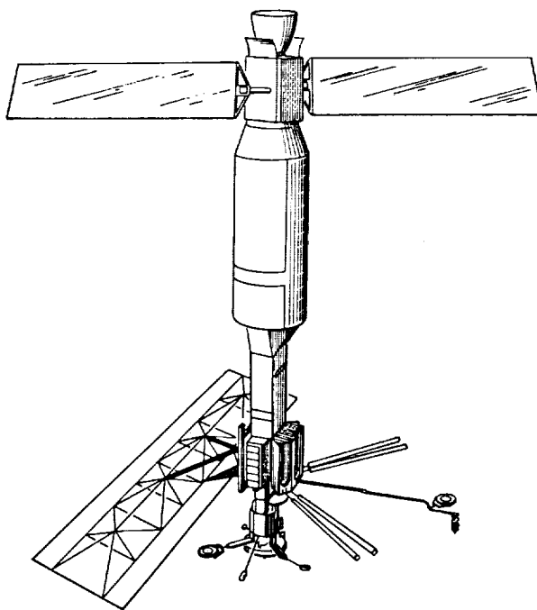
Figure 6. Extendible support structure for SEASAT synthetic aperture radar antenna
