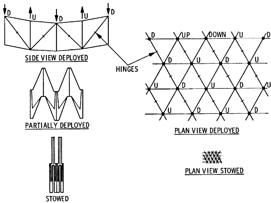
Figure 11. PACTRUSS concept
