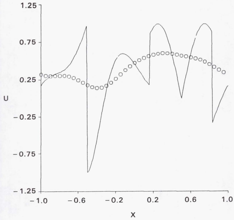
Figure 9a. First-order accuracy
