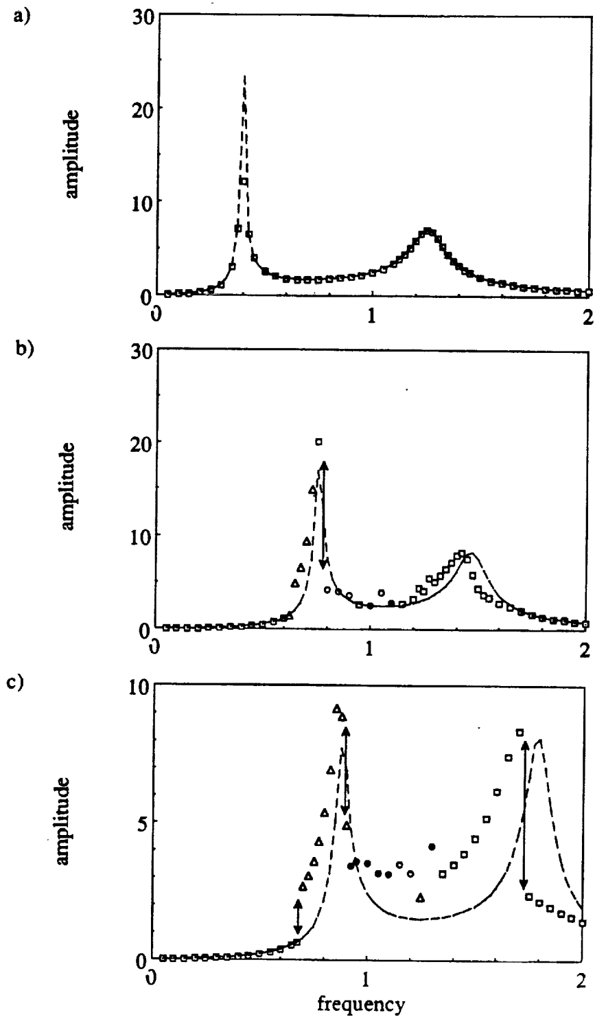
Figure 3.36. y_{gia} versus \Omega_b plots for the case of deep-groove ball bearings; F_m=10 , F_{ah}=5 , F_{bi}=0 , b_h=0 , b_{bi}=b_c=0.001\text{mm} , a) k=1 , b) k=5 , c) k=10 ; □ harmonic, Δ period-one nonharmonic, ○ period- n subharmonic, ● quasi-periodic or chaos, ----- corresponding linear response.
