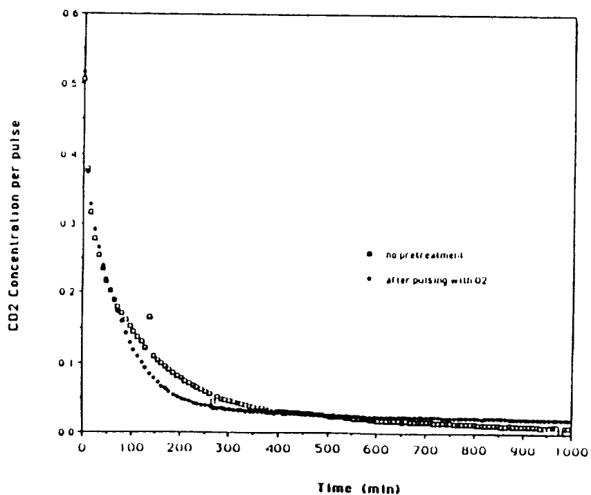
Figure 10: A comparison of CO 2 yields for the 5.8% Pt/SnO 2 /SiO 2 catalyst with no pretreatment \square , and after the pretreated catalyst had been exposed to O 2 \diamond .
