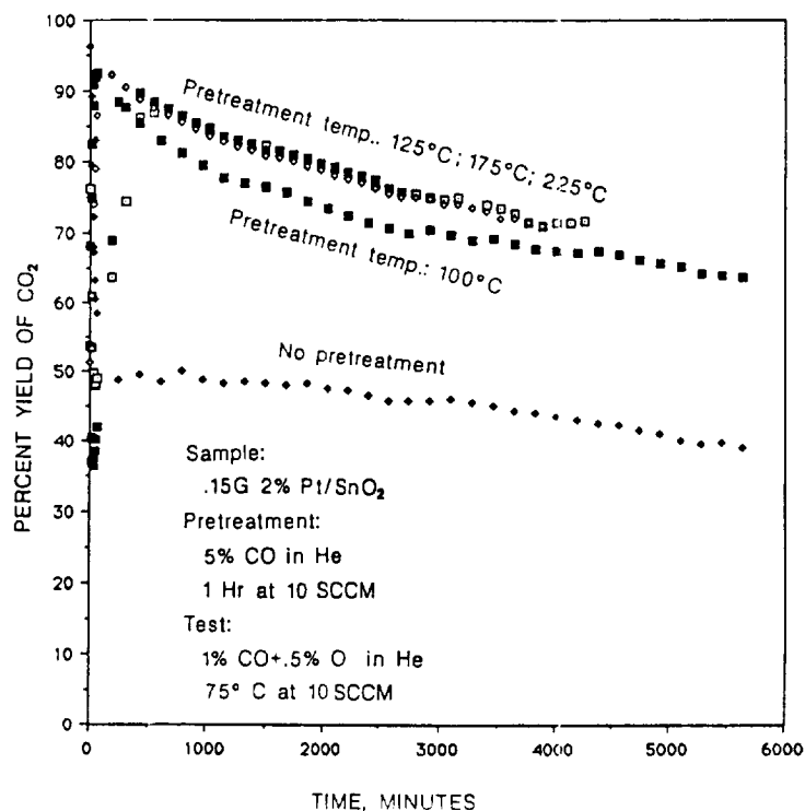
Figure 1. Catalytic activity of the Engelhard platinized tin oxide catalyst for CO oxidation shown as a function of time and pretreatment temperature. The pretreatment and reaction test conditions are given in the figure.
