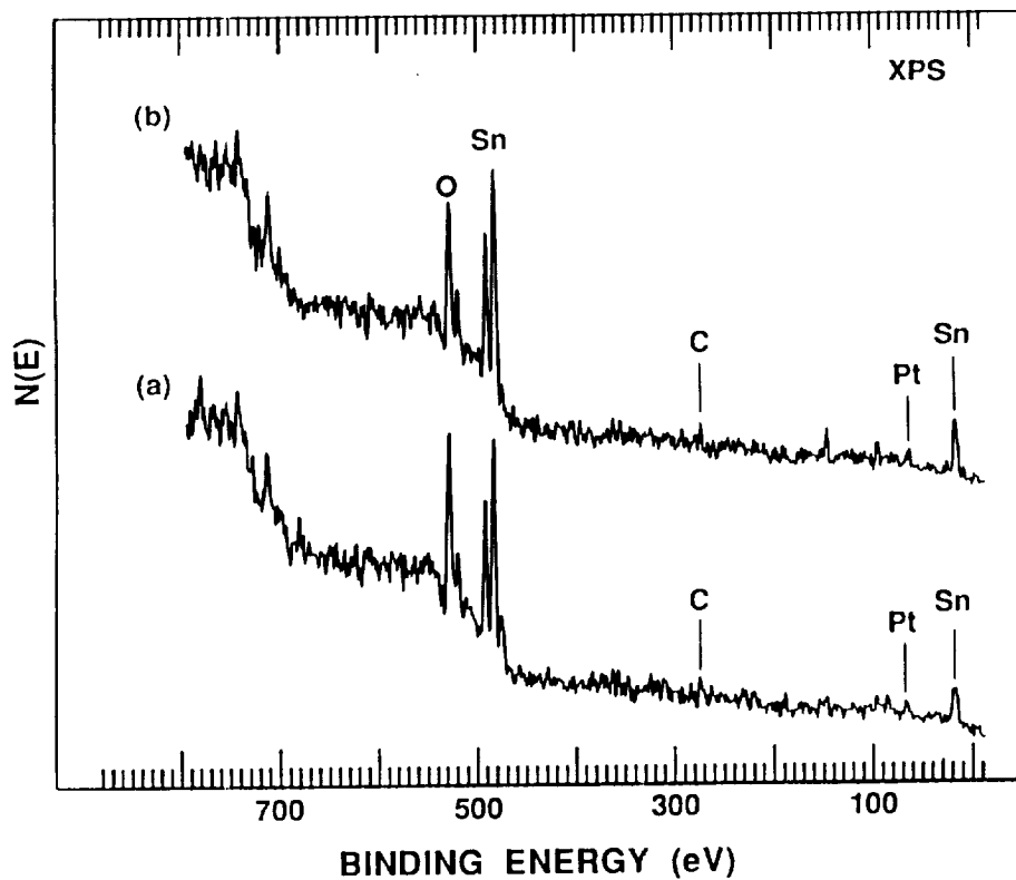
Figure 2. XPS survey spectra taken from the platinized tin oxide surface of sample B (a) before and (b) after CO reduction at 250 °C.
