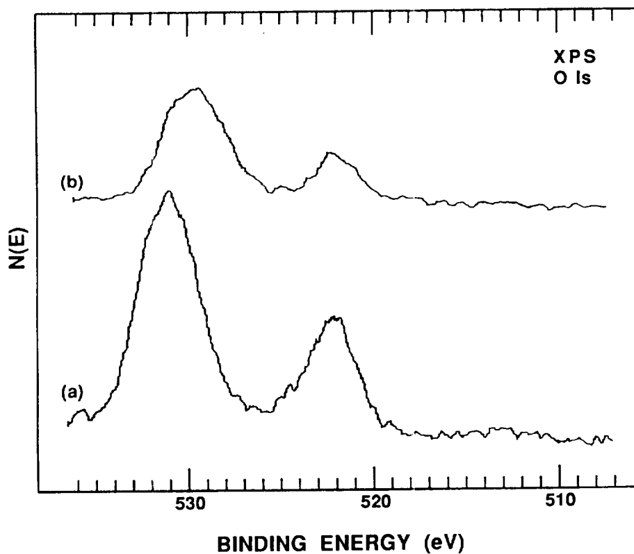
Figure 8. O 1s XPS spectra taken from sample B (a) before and (b) after CO reduction at 250 °C.
