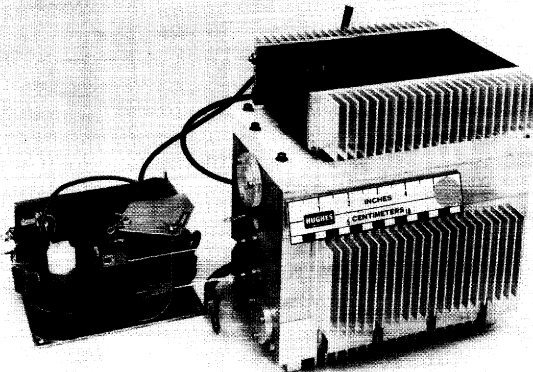
Figure 3. Modular TE laser.
