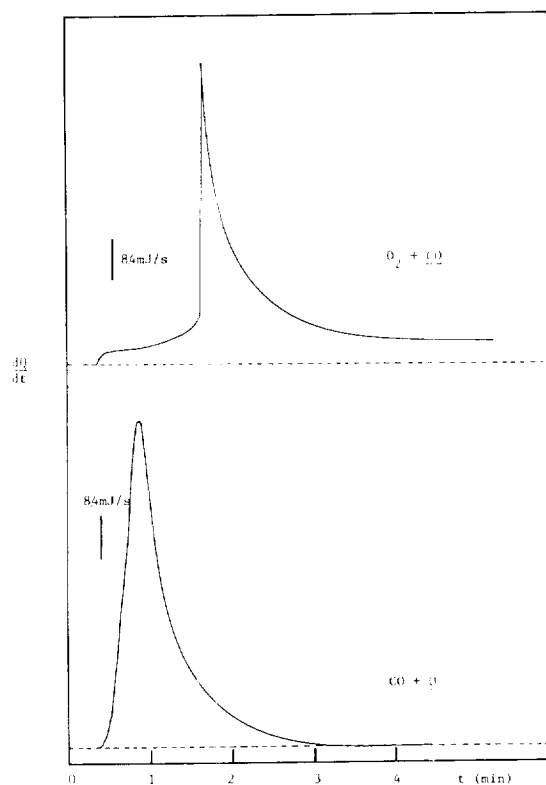
Figure 1 Thermokinetic profiles during titration of pre-adsorbed \underline{\text{O}} by \text{CO}(\text{g}) and preadsorbed \underline{\text{CO}} by \text{O}_2(\text{g}) on \text{Pt/SiO}_2 (S6).
