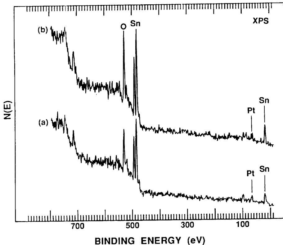
Figure 1. XPS survey spectra taken from the platinized tin oxide surface of sample A (a) before and (b) after CO reduction at 125 °C.
