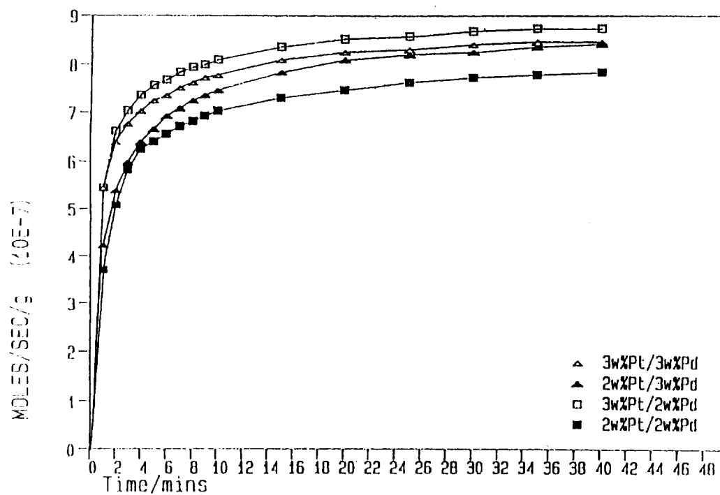
Figure 3. Activity tests of group 3 catalysts.
