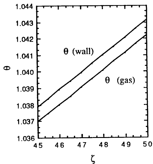
Figure 4. Dimensionless temperatures for Table 1 case.
