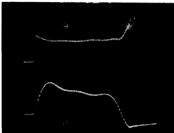
Fig. 3. Main discharge voltage and current waveforms. 5 KV/div, 45 A/div, 5 \mu S/div
