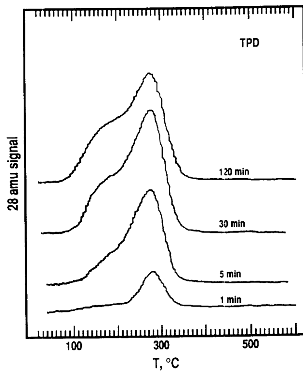
Figure 5. 28 \text{ amu} TPD spectra obtained after exposing polycrystalline Pt to CO at 1 \times 10^{-8} Torr and room temperature for various periods.
