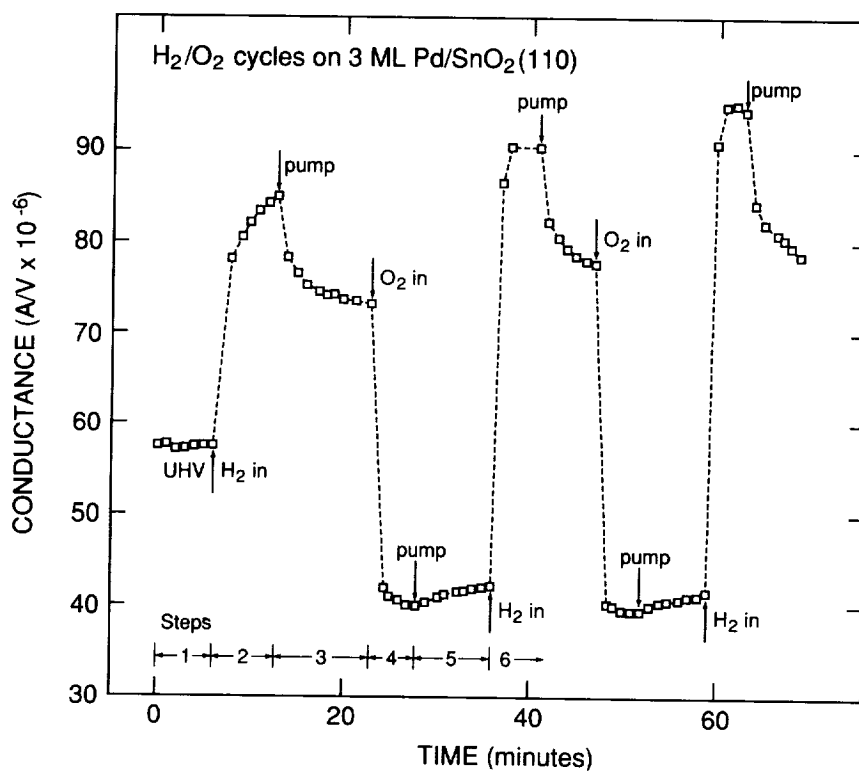
Figure 5. Conductance versus time for sequential hydrogen and oxygen exposures of the 3 ML Pd/ \text{SnO}_2(110) surface at 400K. All gas exposures were performed at a constant pressure of 10^{-5} mbar. Refer to text for further details.
