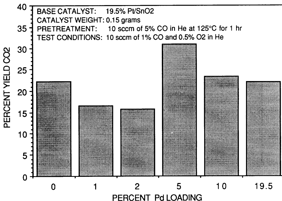
Figure 6. Activity at 20,000 minutes of some (Pt+Pd)/SnO 2 catalysts
