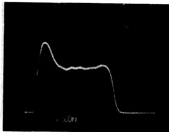
Fig. 2 Transmitted primary current collected at cathode. 10 mA/div. 5 \mu S/div
