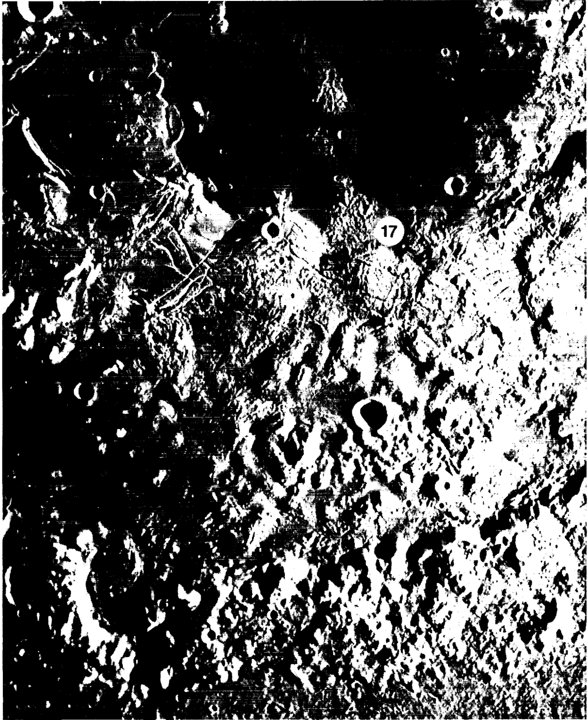
Figure V-3b. High resolution photograph of suggested landing site on the Mauser Formation inside the Orientale basin. This site would allow collection of impact melt (light-colored material next to the number) and probably some mare basalt (dark material nearby, to the north) thrown to the landing site by impacts on the mare.
