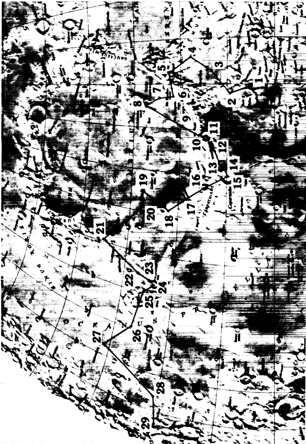
Figure VI-7. The route of a proposed traverse across the Imbrium-Procellarum region is illustrated here on a National Geographic (Lambert equal area) base map. Numbers refer to the prime field sites described in Table VI-3. Although segments are drawn as straight lines, they would actually be sinuous as the crew made numerous shorter stops along the way.
