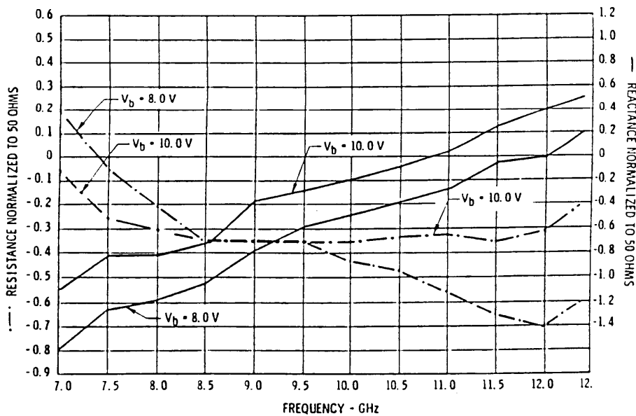
Figure 4.4: Effect of bias level on the impedance of a typical X-band oscillator diode (Clark and Swartz, 1971).
