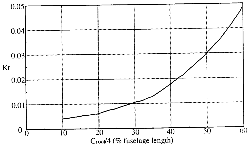
Figure 6: Fuselage Stability Coefficient ( K_f ) vs. Position of Wing Root Quarter-Chord ( C_{\text{root}/4} ) (Reproduced from Reference 4)
