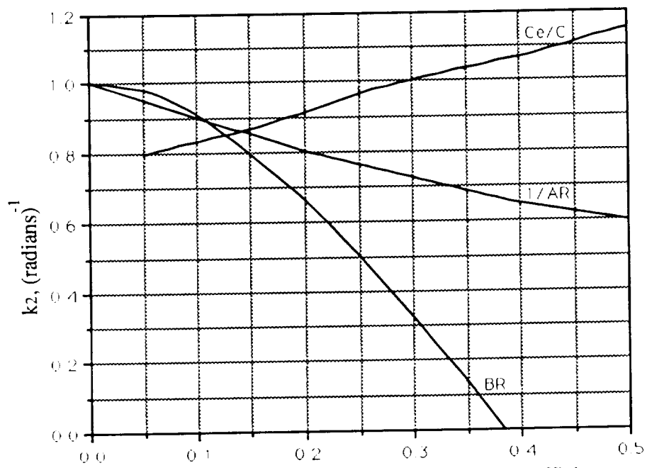
Figure 20: Curves Used in Determining the k_2 Coefficients to Calculate Stick-Free Effects. BR, 1/A, Ce/C
