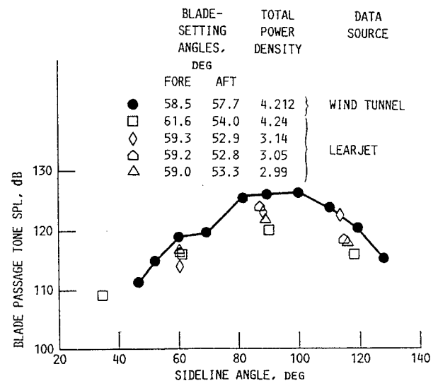
FIGURE 25. - UDF FUNDAMENTAL TONE DIRECTIVITY MEASURED IN FLIGHT, COMPARED WITH SCALED MODEL DATA; F7/A7 BLADE CONFIGURATION AT MACH 0.72 CRUISE CONDITIONS. SIDELINE DISTANCE, 47.2 M (155 FT) ALTITUDE, 10688 M (35000 FT).
