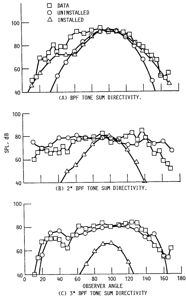
FIGURE 26. - COMPARISON OF PREDICTION WITH FLY-OVER UDF DATA FROM GROUND PLANE MICROPHONE - 100% THRUST. M = 0.255 , PRESSURE ALTITUDE = 1323 m (4340 FT).
