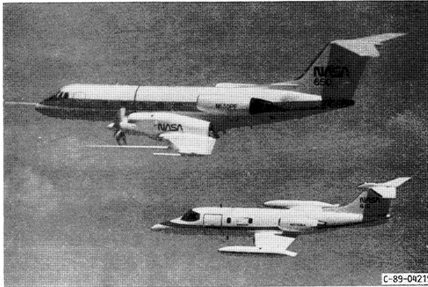
FIGURE 21. - PROPELLER TEST ASSESSMENT (PTA) GULFSTREAM II AIRCRAFT WITH 9 FOOT (2.74 M) DIAMETER SR-71 PROPELLER MOUNTED ON THE WING. LEWIS INSTRUMENTED LEARJET IN FORMATION.
