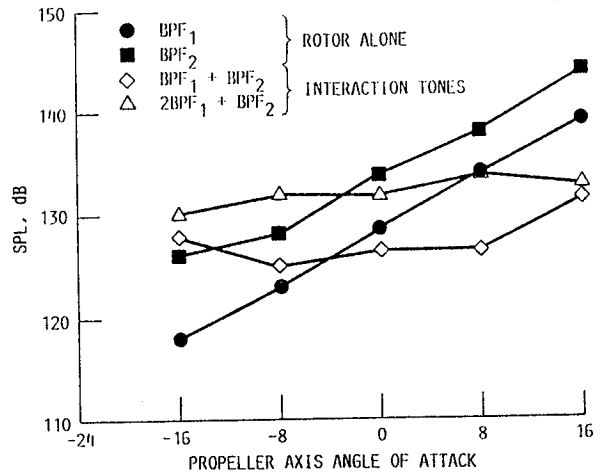
FIGURE 14. - ANGLE OF ATTACK EFFECTS ON COUNTERROTATION TONES IN AFT PROPELLER PLANE, BELOW THE AIRCRAFT. F7/A7, 11X9; \beta_1/\beta_2 = 36.4^\circ/36.5^\circ ; 90% SPD; M_\infty = 0.2 .
