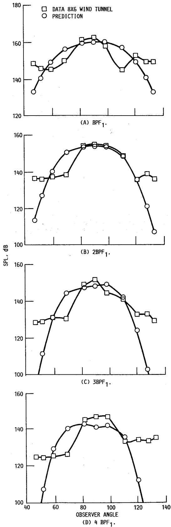
FIGURE 16. - COUNTERROTATION PROPELLER NEAR FIELD TONE DIRECTIVITY AT CRUISE CONDITIONS, F1/A1, 9X8, M = 0.72, 100% SPEED.
