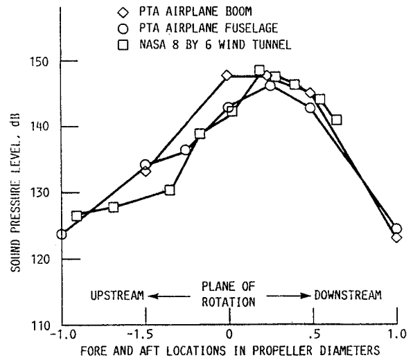
FIGURE 5. - COMPARISON OF SCALED ACOUSTIC DATA FROM THE 8 BY 6 WIND TUNNEL WITH FULL SCALE PTA FLIGHT DATA, M = 0.8 (DATA CORRECTED TO PTA FUSELAGE CONDITIONS ON A 3.05 M (10 FT) SIDELINE).
