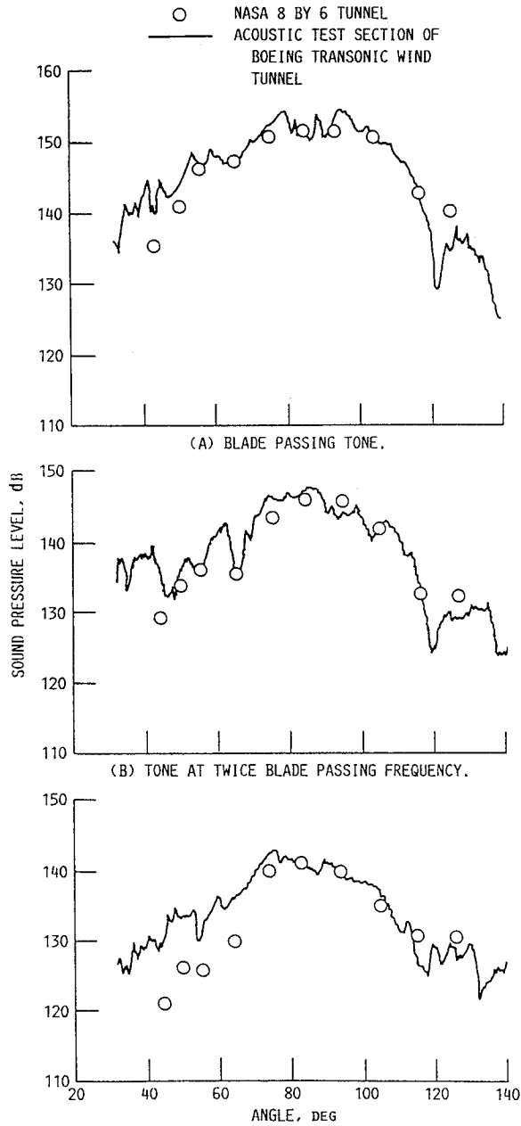
FIGURE 4. - COMPARISON OF ACOUSTIC DATA FOR THE F7/A7 COUNTERROTATION PROPELLER MODEL IN THE NASA LEWIS 8 BY 6 AND BOEING TRANSONIC WIND TUNNELS. (100% SPEED, M = 0.72 , DATA ADJUSTED TO BOEING CONDITIONS ON A 67 CM (2.2 FT) SIDELINE).
