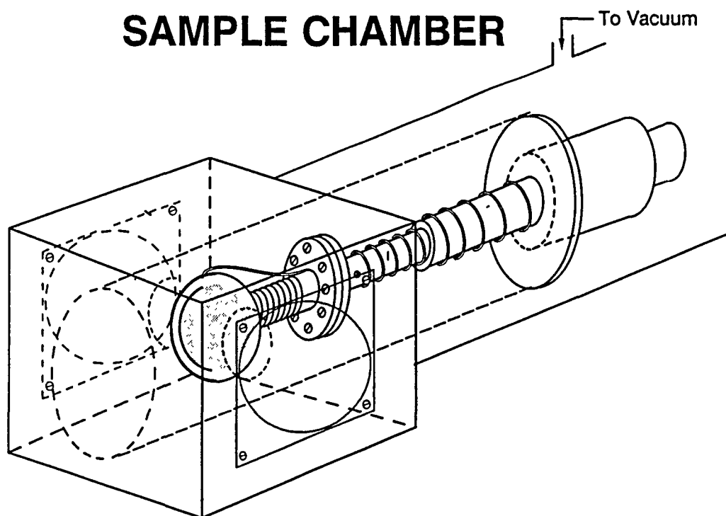
Figure 1. Sample chamber for TFIR vapor pressure experiments.
