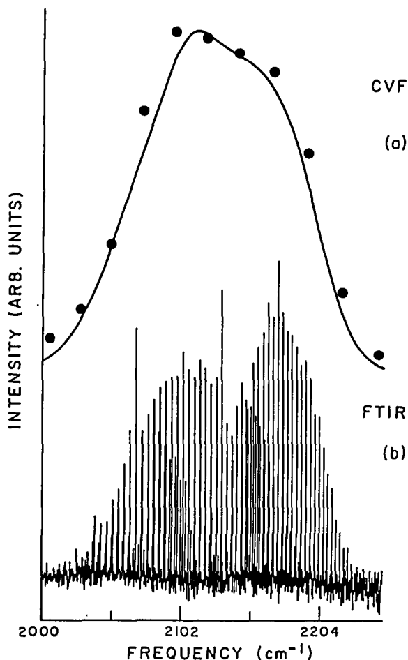
Fig. 4. Comparison of CO emission spectra following acetone photodissociation taken with (a) a low resolution circular variable filter (CVF) and (b) the high resolution FTIR.
