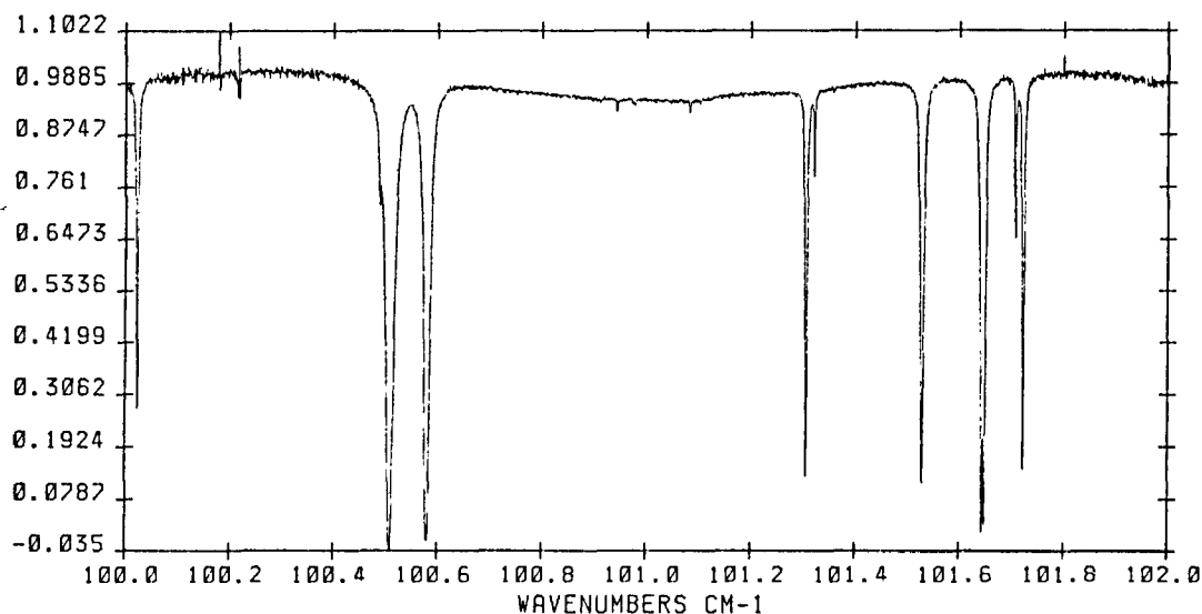
Fig. 9: Bruker Spectrum of HDO at 2 Torr Pressure
