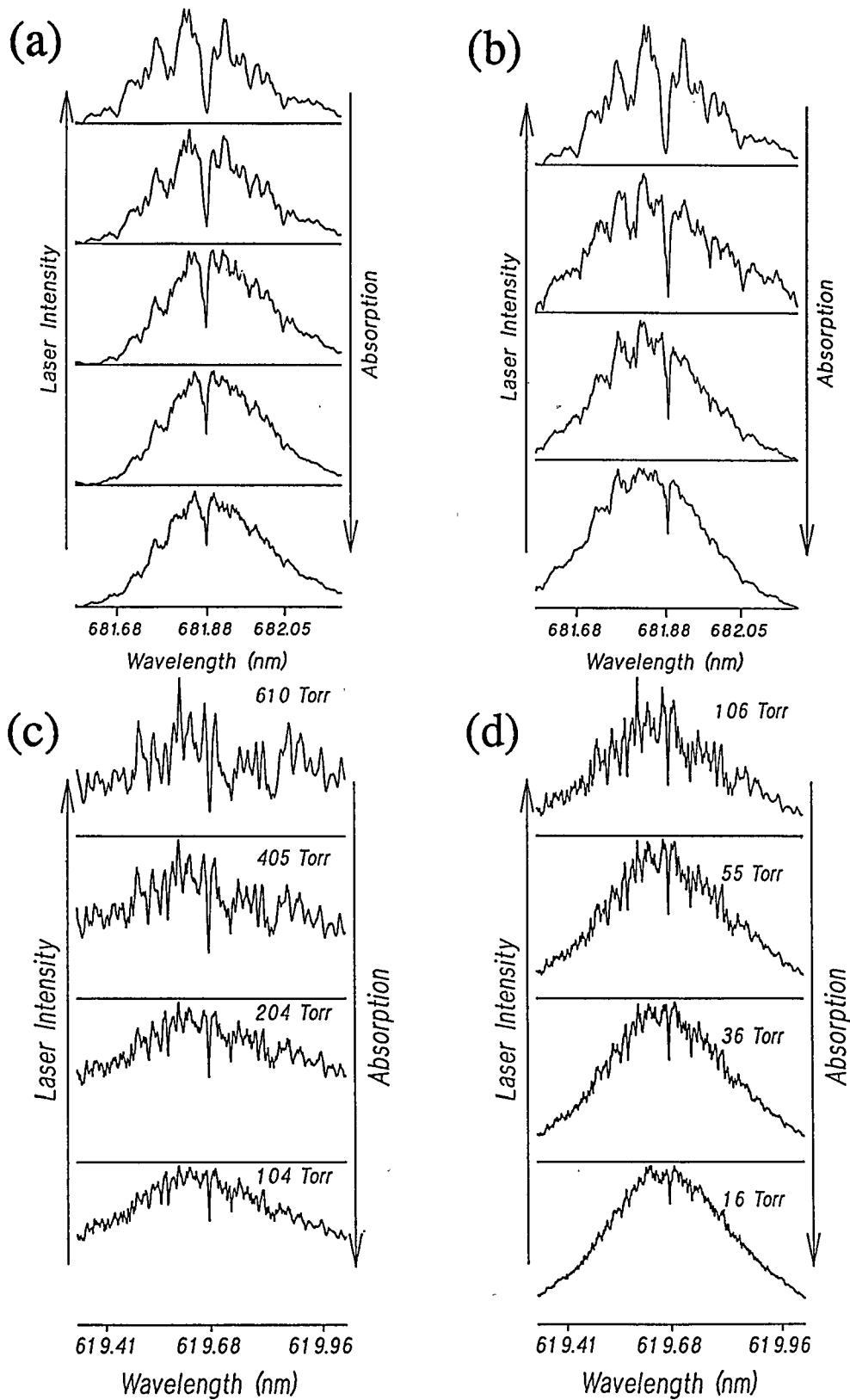
Figure 1. ILS spectral profiles for CH 4 absorption in the 681.86 nm (top panels) and 619.68 nm (bottom panels) bands under various conditions: (a) \sim 180 K, CH 4 pressures from top to bottom profile: 364, 184, 95, 45, 22 Torr, t_s=170 \mu s, effective absorption pathlength ( L_{eff} )=36 km; (b) L_{eff} =36 km, conditions from top to bottom profile: 364 Torr & 175K, 70 Torr & 110-160 K, 20 Torr & \sim 110 K, 10 Torr & <110 K; (c) 295 K, t_s=10 \mu s; (d) 295 K, t_s=100 \mu s.
