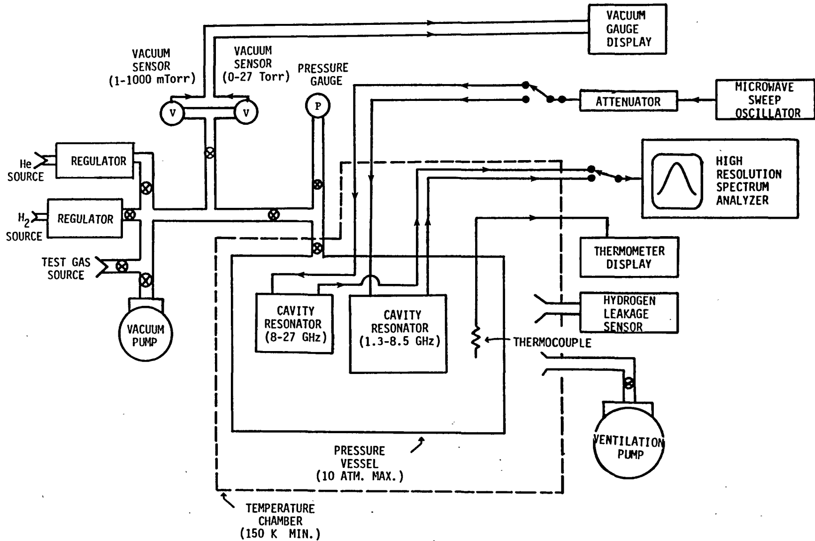
Figure 2: Block diagram of the atmospheric simulator, as configured for measurements of the refraction and microwave absorption of test gases ( \text{NH}_3 , \text{CH}_4 , and \text{H}_2\text{O} ) under simulated Jovian conditions.
