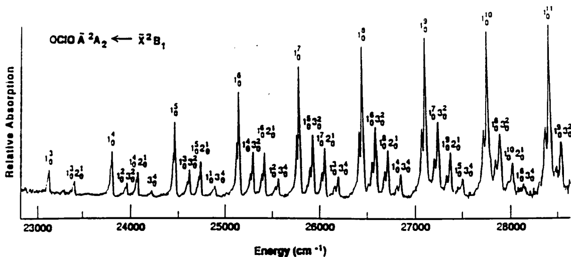
Figure 1: Portion of the jet cooled absorption spectrum of chlorine dioxide. Recorded at 5\text{cm}^{-1} resolution and 2 atm total stagnation pressure (3% OClO in He).
