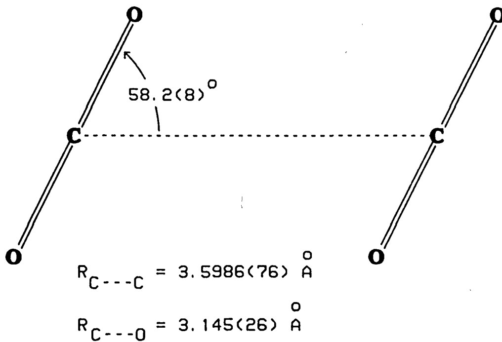
Fig. 1. Structures of CO 2 Dimer and Trimer
