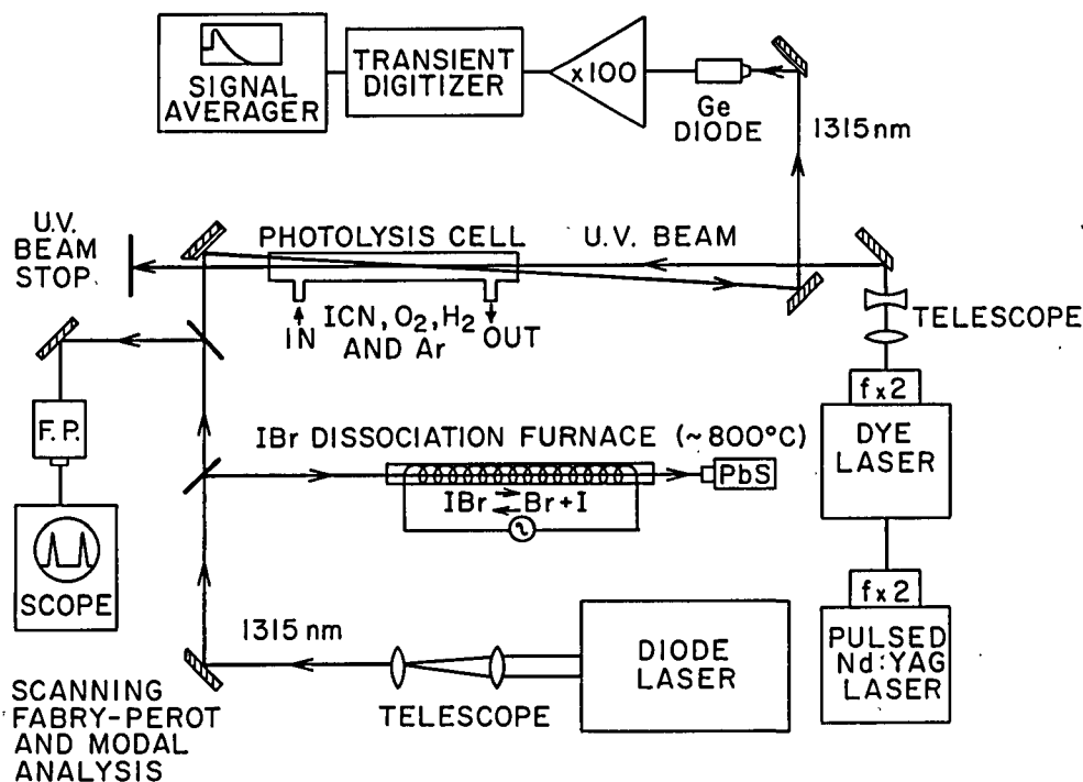
Fig. 6 . Laser gain-versus-absorption apparatus using a diode laser to study I^* quantum yields. The heated IBr cell is for tuning the diode laser to the I atom transition.
