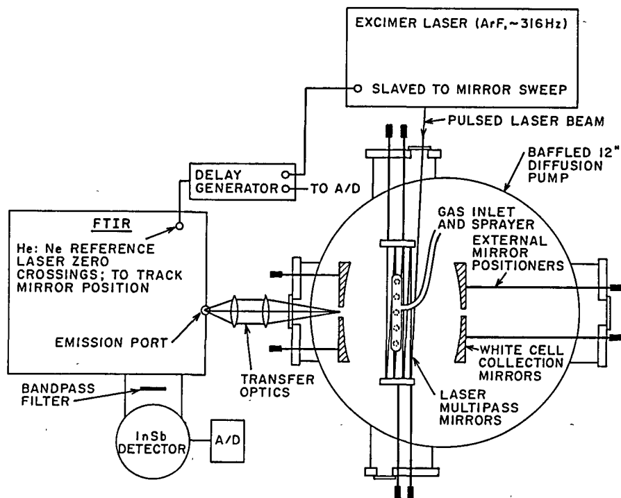
Fig. 1. Experimental apparatus for time-resolved FTIR emission experiments initiated by laser photodissociation.
