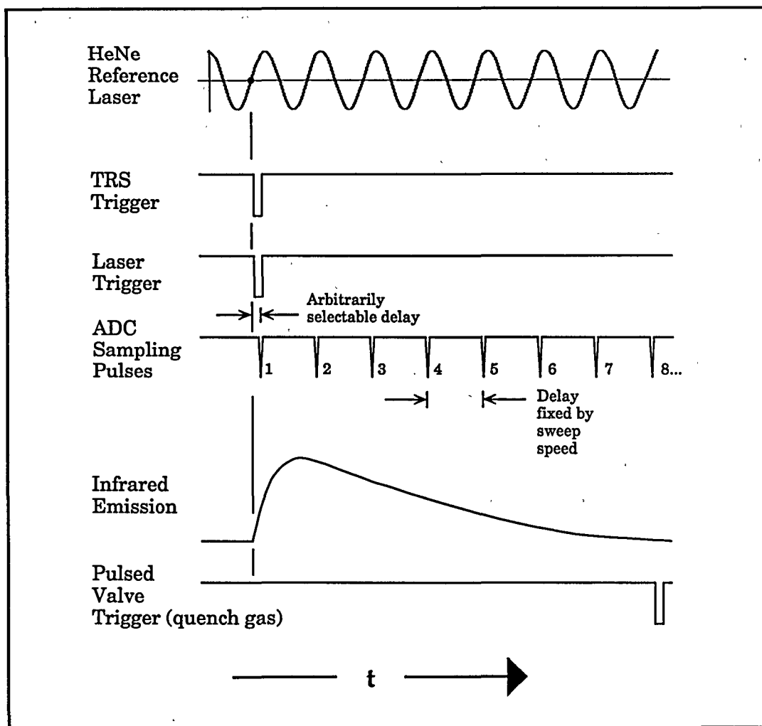
Fig. 2. Timing diagram for time resolved FTIR emission experiment, showing 8 time samples after each laser pulse.
