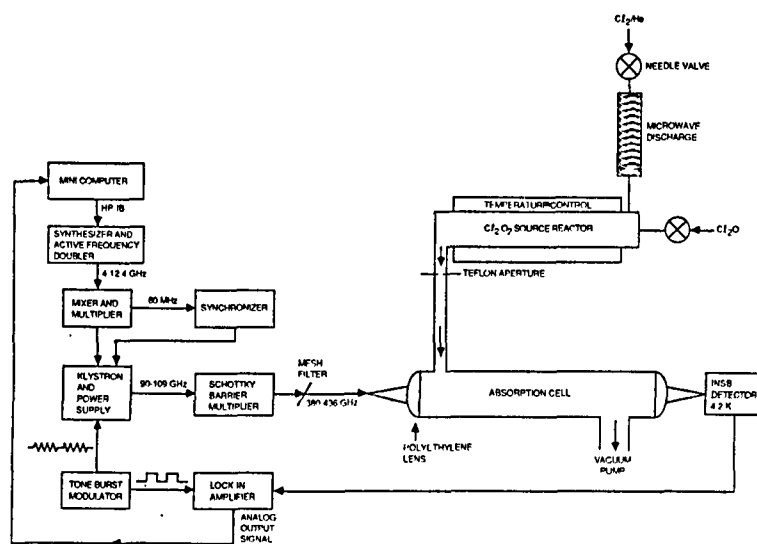
Fig. 1: Submillimeter Spectrometer Using Harmonic Generation
