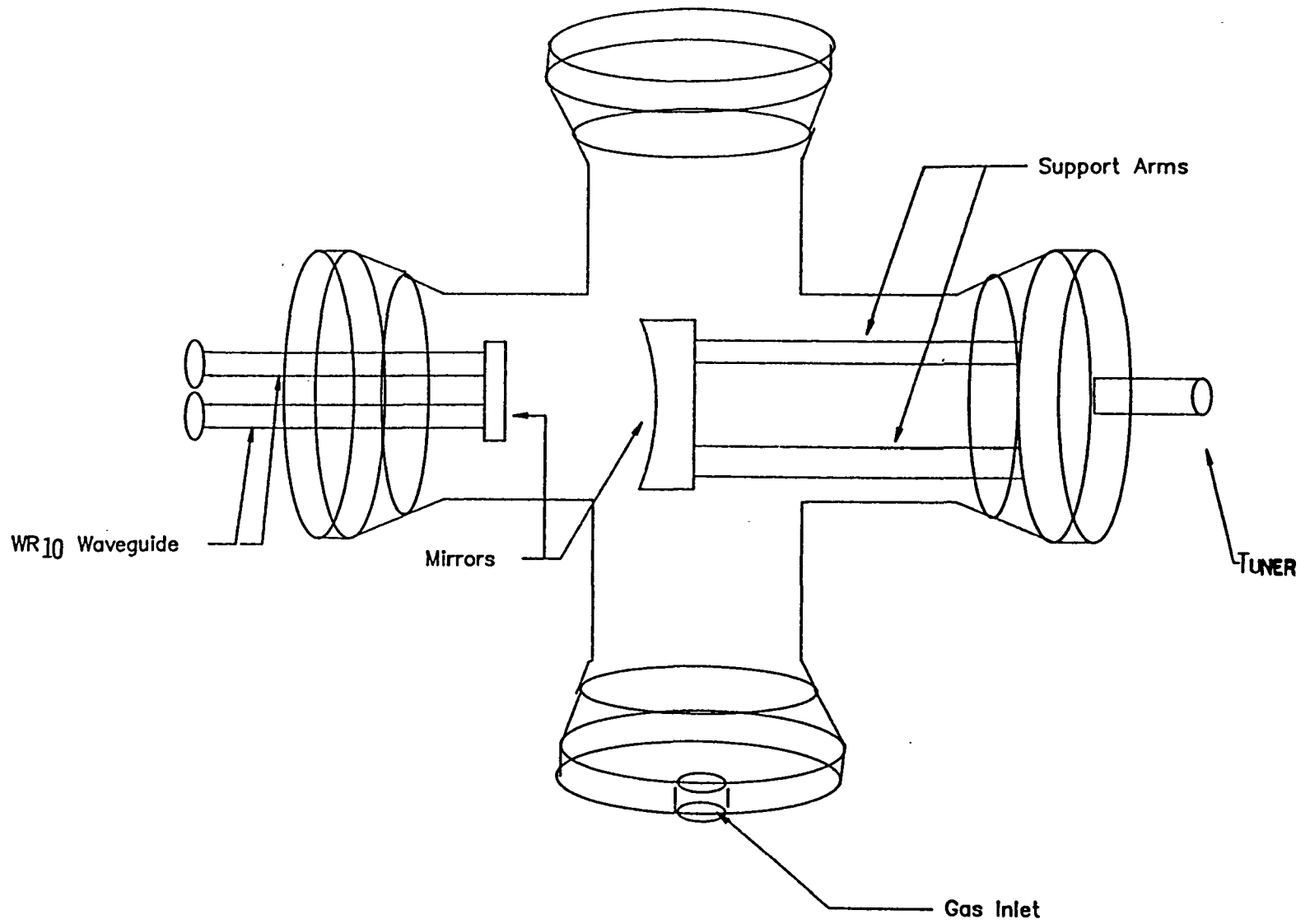
Figure 4: DIAGRAM OF FABRY-PEROT RESONATOR (94GHz)
