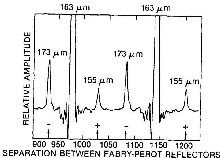
Fig. 7: Fabry-Perot Scan of Laser Sideband Output
