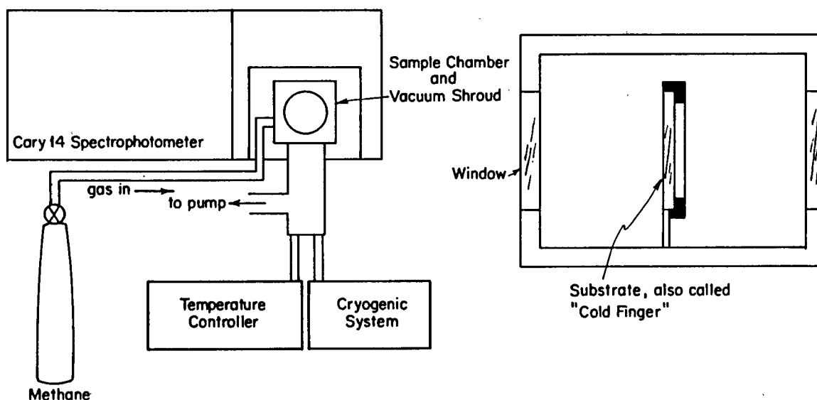
Fig. 1. Experimental set-up to measure transmission through methane film at 10°K
