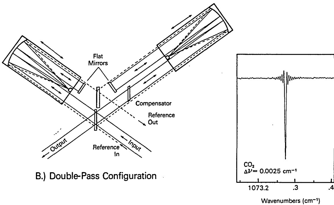
Figure 6. Single-pass (A) and double-pass (B) configurations of the 1-meter FTS at Kitt Peak (Jennings et al. 1985).
