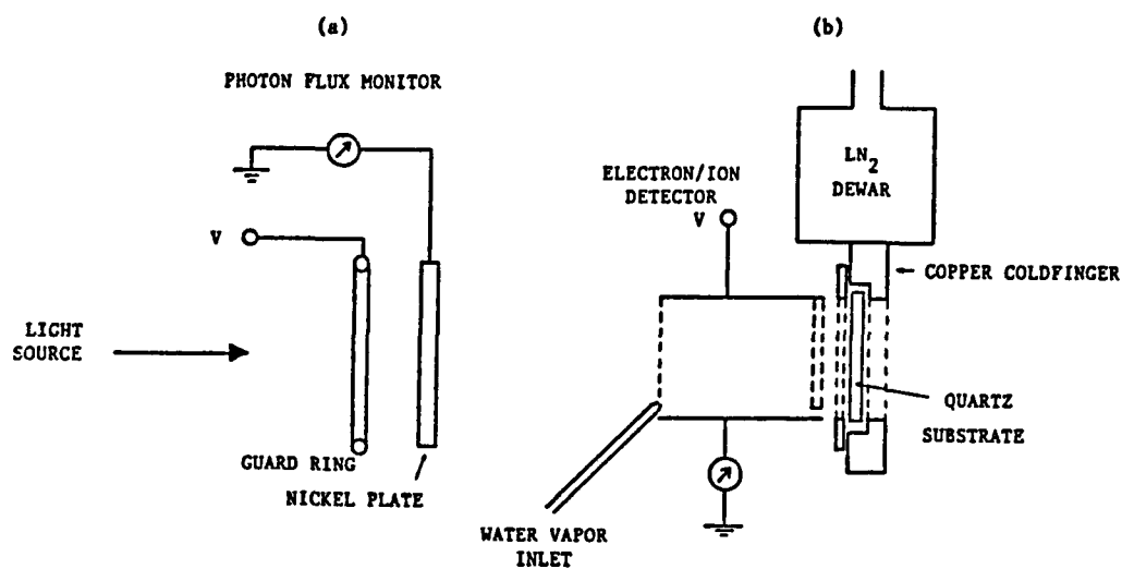
Fig.2. Detailed diagrams for (a) the photon flux monitor and (b) the photon-water ice interaction region.
