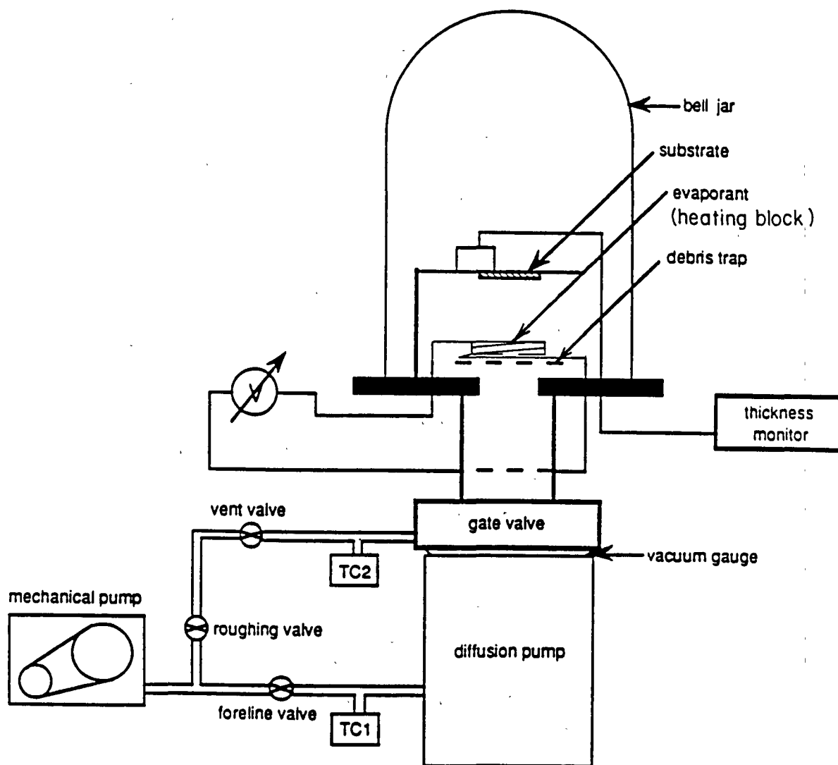
Fig. 1. Apparatus for vacuum-evaporation and film deposition.
