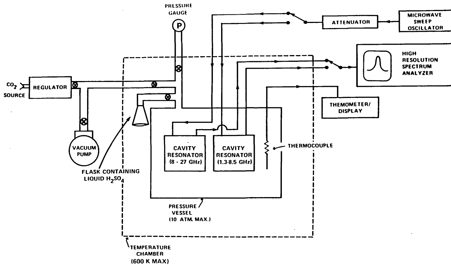
Figure 1: Block diagram of the atmospheric simulator as configured for measurements of the microwave absorption and refraction of gaseous \text{H}_2\text{SO}_4 under Venus atmospheric conditions over the 1.2-22.3 cm wavelength range.
