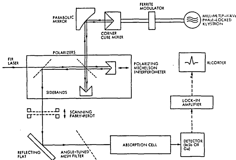
Fig. 6: Laser Sideband Generator
