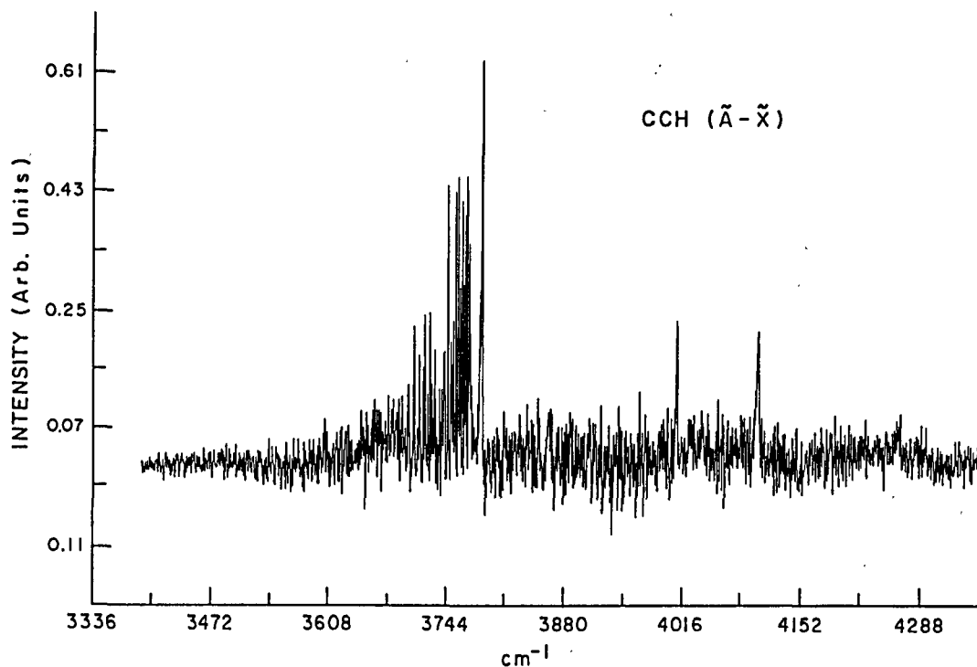
Fig. 3. Infrared emission spectrum of CCH taken with the FTIR at 0.6 cm -1 resolution at a time of 7 \mu s after the photolysis of acetylene.
