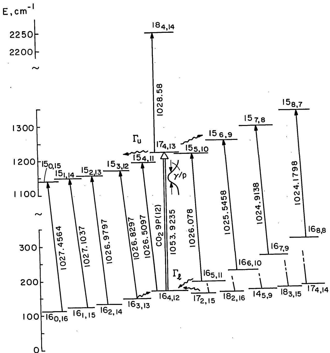
Figure 2. Infrared double-resonance level scheme for \text{CO}_2 laser 9P(12) pumping of ozone, showing probe frequencies for three- and four-level IRDR configurations.
