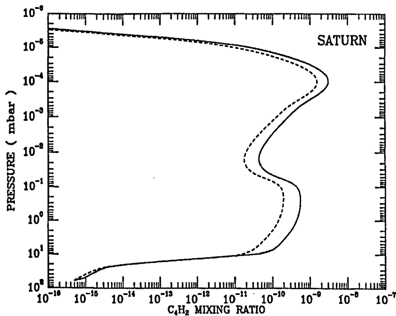
Figure 2 - Diacetylene mixing ratio vs. pressure in the stratosphere of Saturn. Solid line is for Set 1 C_2H reaction rates, dashed line Set 2 reaction rates, both assume (a) pathway for C_2 + CH_4 . Rapid decrease in mixing ratio for pressures greater than 10 mbar is due to condensation.
