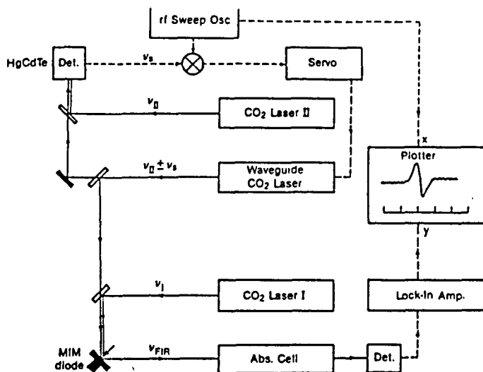
Fig. 3: Two Photon Laser Difference Generation
