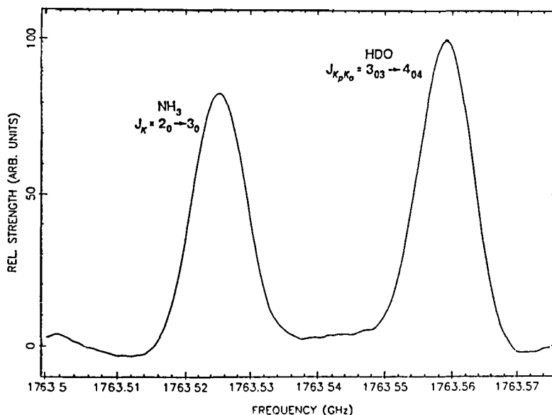
Fig. 8: Laser Sideband Spectrum of NH 3 and HDO
