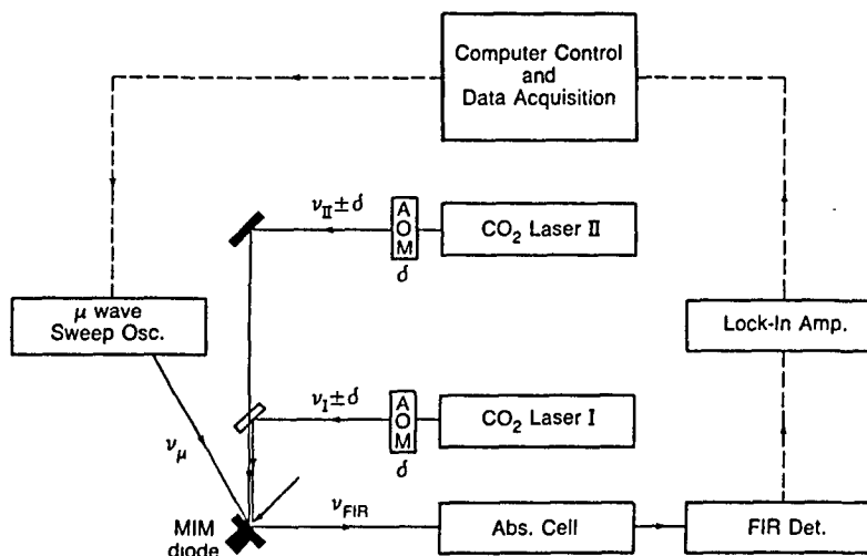
Fig. 4: Three Photon Laser and Microwave Difference Generation
