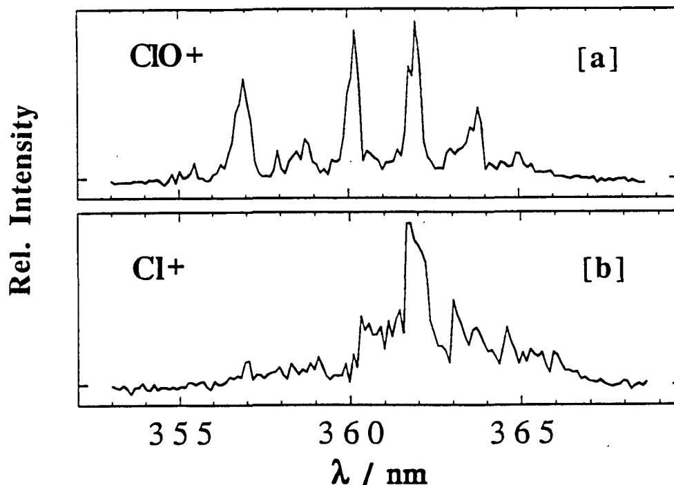
Figure 3: Resonance enhanced multiphoton ionization (REMPI) spectrum of ClO + [a], and Cl + [b] between 353 and 369 nm.
