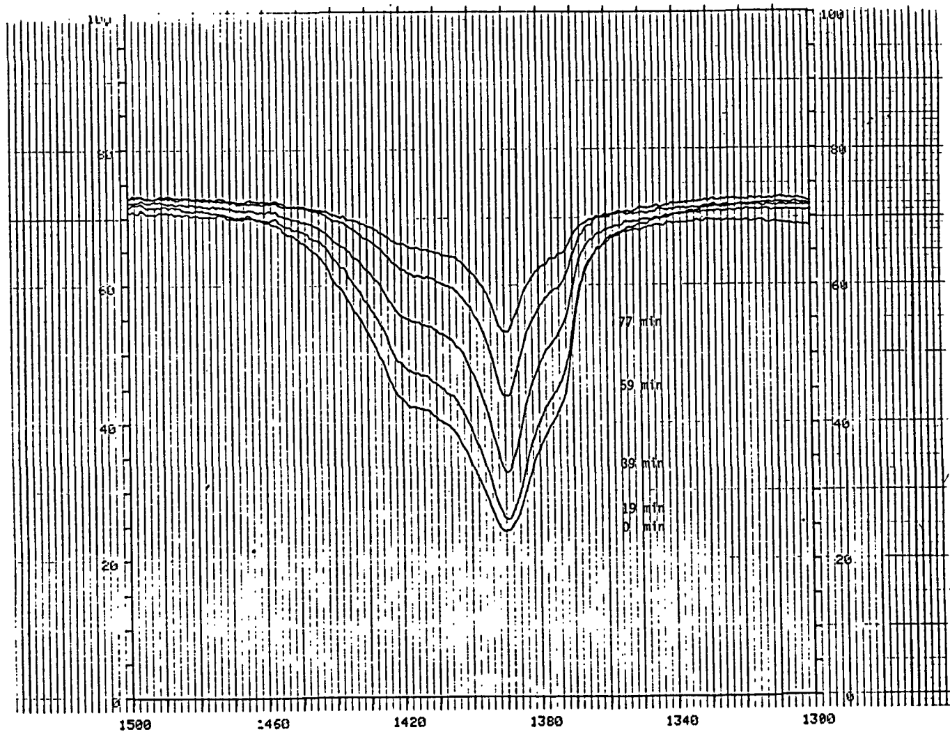
Figure 2. Transmission spectra, at different times of acetylene at 80K.
