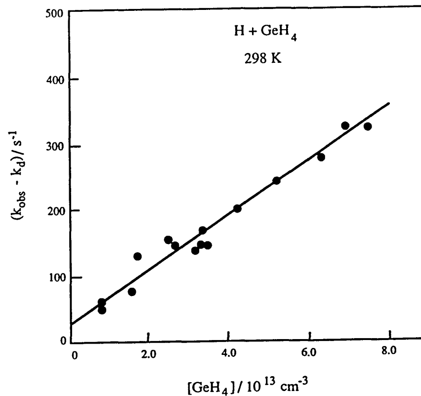
Figure 3. First-order decay constants vs. germane concentrations. The line is the linear least-squares fit of these data. The slope of this line is the reaction rate constant, k , for H + GeH 4 at 298 K.
