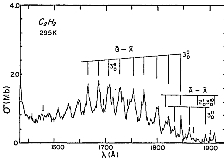
Fig.5. The absolute photoabsorption cross section of C_2H_2 in the 1520 - 1900Å region. The data are obtained with a spectral bandwidth (FWHM) of 0.8Å and at a temperature of 295^\circ K .
