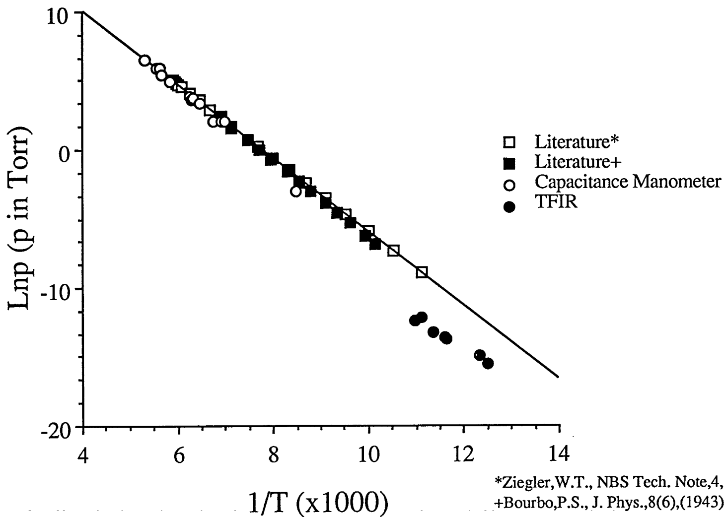
Figure 3. Plot of the literature, capacitance manometer and TFIR vapor pressure data for acetylene.
