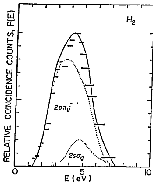
Fig.11. Relative coincidence counts vs. energy.
