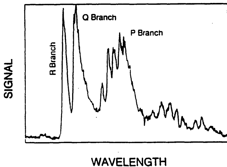
Figure 3. CN FRAGMENT QUANTUM YIELD
