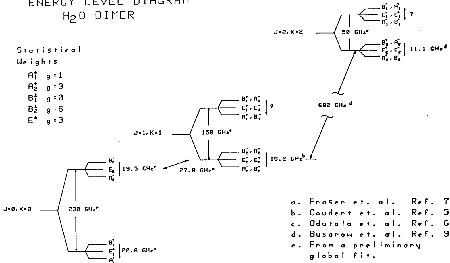
Figure 1. Energy level diagram for (H 2 O) 2 showing the positions of the K_a and tunneling states as determined from previous studies (Ref. 6 and references cited therein). For the J=1, K_a=1 and J=2, K_a=2 states, two symmetry species are shown for each level to indicate the asymmetry doubling. Frequencies marked with a superscript e are not directly measured but are estimated from a global fit (Ref. 7) of the reported microwave and far-infrared results to a rotational-tunneling Hamiltonian for (H 2 O) 2 .
