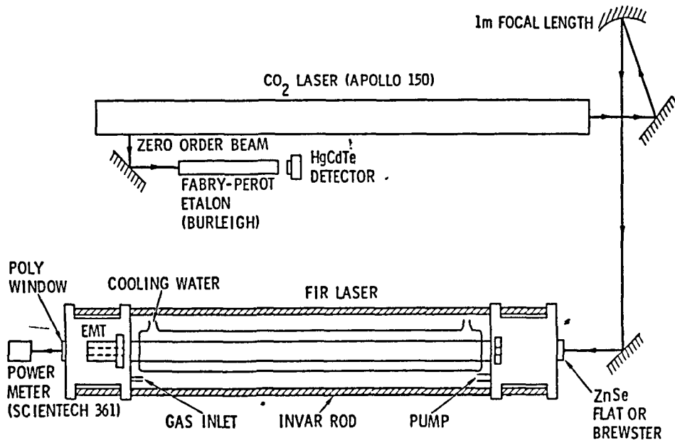
Fig. 5: Far Infrared Laser
