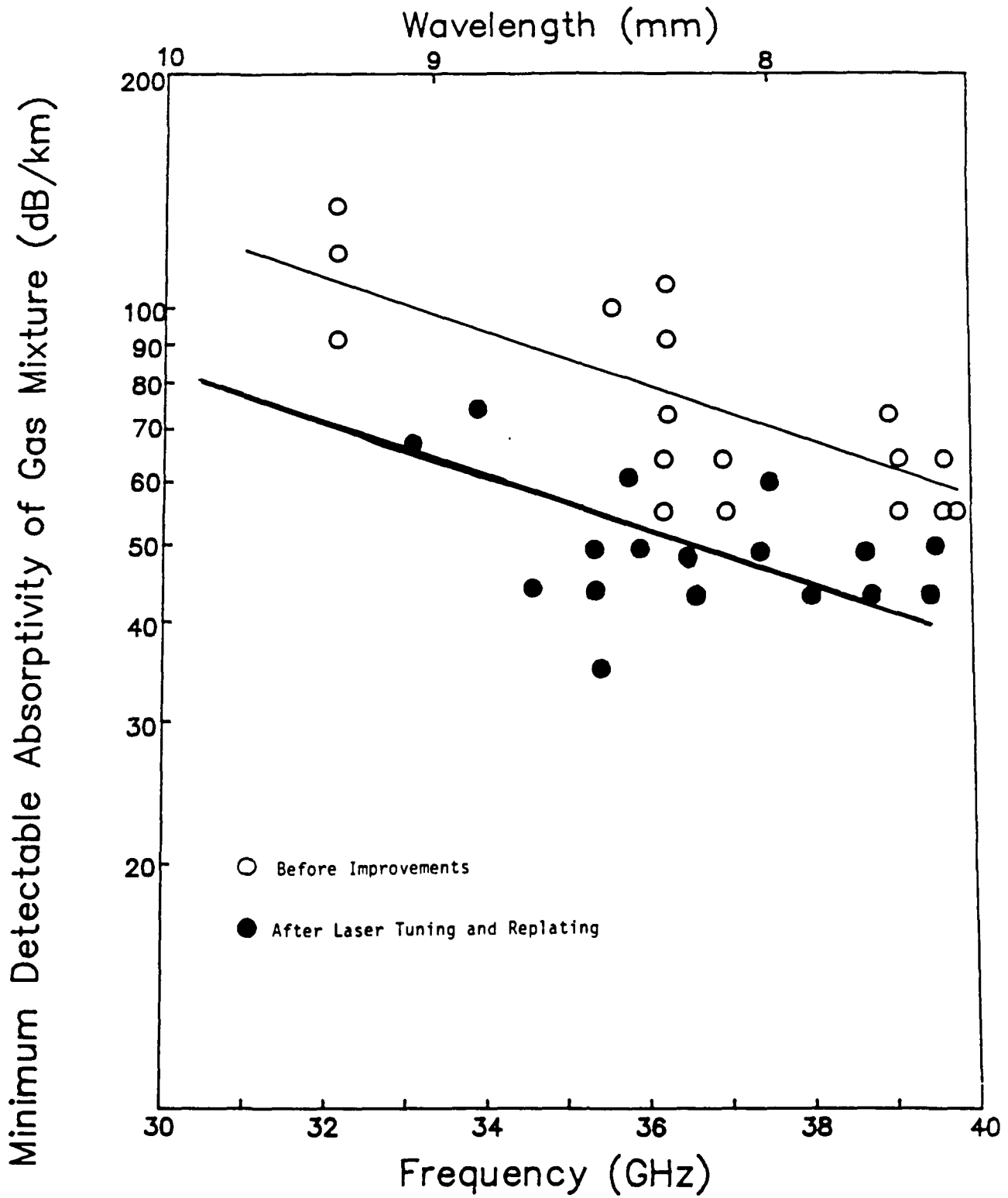
Figure 6: Performance (minimum detectable absorptivities) for the 32-40 GHz resonator system (operating at 200 K). Note improvement in average performance (solid lines) after laser tuning.
