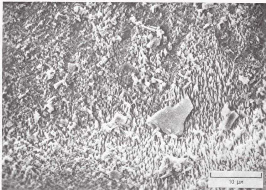
(n) ROCKETDYNE PANEL-8 C-C COMPOSITE AFTER ATOMIC OXYGEN DIRECTED EXPOSURE AT A FLUNECE OF 5.8 \times 10^{20} ATOMS/CM 2 .
