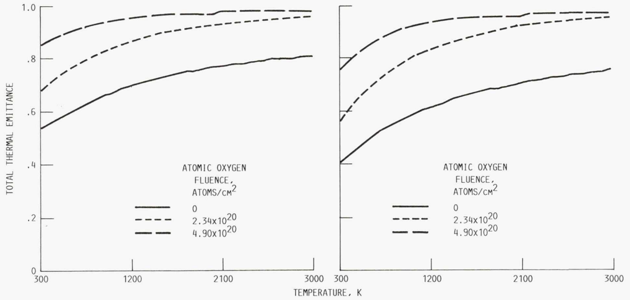
(i) ROCKETDYNE C773-1 C-C COMPOSITE.
