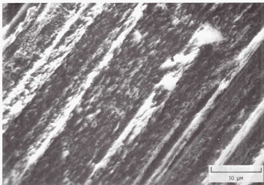
(f) KAISER C C-C COMPOSITE AFTER ATOMIC OXYGEN DIRECTED EXPOSURE AT A FLUENCE OF 4.2 \times 10^{20} ATOMS/ \text{cm}^2 .
