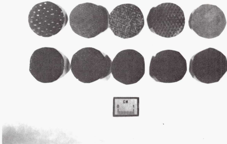
(a) C-C COMPOSITES FROM BATCH 1 AS RECEIVED (TOP) AND AFTER TEXTURING WITH ATOMIC OXYGEN (BOTTOM). LEFT TO RIGHT, ROHR, KAISER A, KAISER C, FIBER MATERIAS 4-D WEAVE, AND FIBER MATERIASL ISOSTATICALLY PRESSED.
