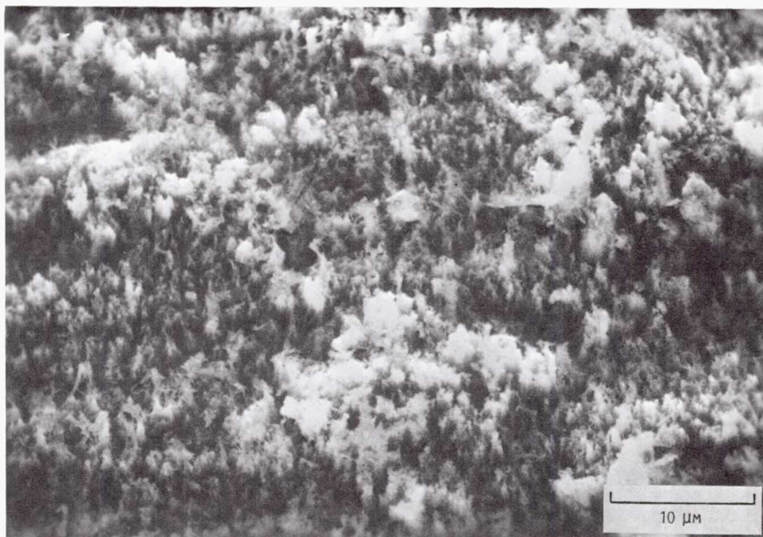
(d) KAISER A C-C COMPOSITE AFTER ATOMIC OXYGEN DIRECTED EXPOSURE AT A FLUENCE OF 4.2 \times 10^{20} ATOMS/ \text{cm}^2 .
