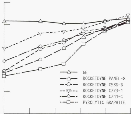
(b) BATCH 2, TOTAL THERMAL EMITTANCE AT 500 K.
