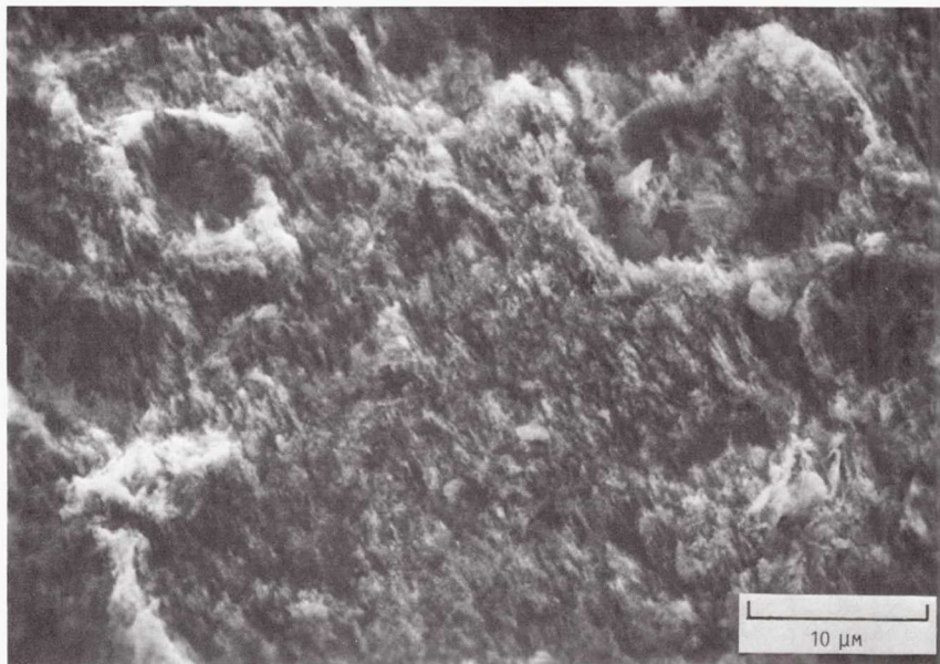
(j) FIBER MATERIALS ISOSTATICALLY PRESSED C-C COMPOSITE AFTER ATOMIC OXYGEN DIRECTED EXPOSURE AT A FLUENCE OF 4.2 \times 10^{20} ATOMS/ \text{cm}^2 .
