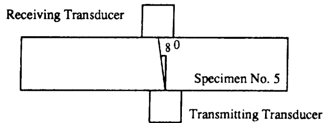
Fig. 10 Through transmission offset transducer arrangements for measuring input-output signals in experimental method I.
