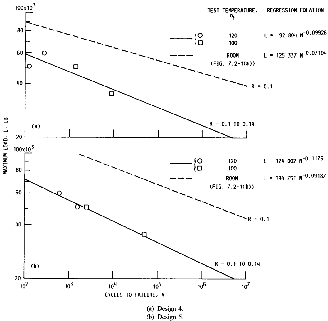
Figure 7.2-3.—Tension-tension fatigue strength at elevated temperature of two metal stud test specimen designs for stress ratios R of 0.10 to 0.14. Studs bonded with carbon-fiber-filled epoxy resin.
