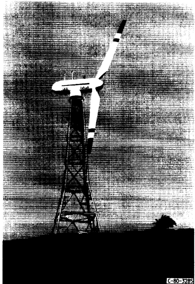
Figure 8.—DOE/NASA 200-kW Mod-0A experimental wind turbine near Kahuku Village, Oahu, Hawaii. Laminated Douglas fir/epoxy blades form the 125-ft-diameter rotor.
