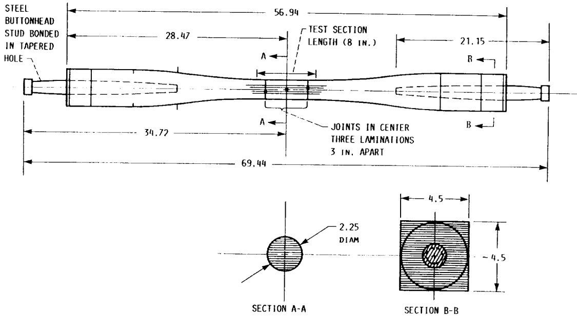
Figure 2.2-13.—Dogbone test specimen for fatigue testing. (Dimensions are in inches.)
