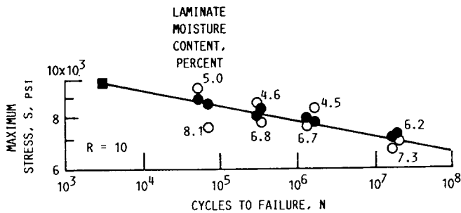
Figure 1.—Moisture correction of data for compression fatigue ( R = 10 ) parallel to grain in laminated Douglas fir/epoxy specimens. Veneer grade, A+. Data from figure 4.2-1 of chapter IV.
