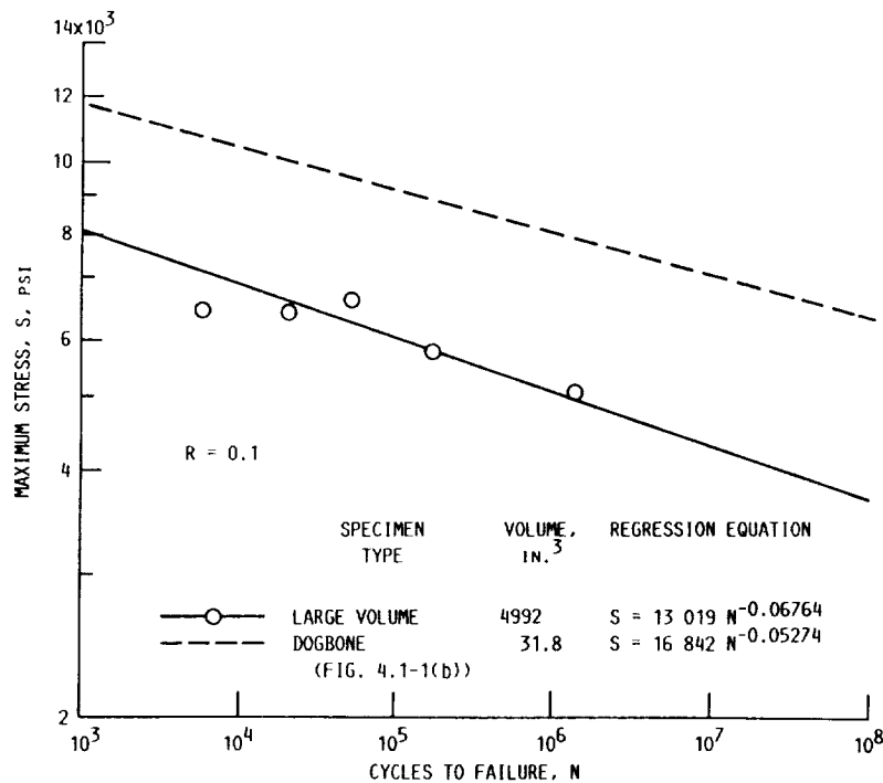
Figure 4.1-3.—Effect of tension-tension fatigue ( R = 0.1 ) parallel to grain for large-volume laminated Douglas fir/epoxy specimens. Specimens 2 in. thick (20 laminations) by 8 in. wide by 360 in. long (4992-in. 3 test volume) with 12:1 slope scarf joints staggered 3 in. apart in all adjacent laminations. Joints spaced 8 ft apart in each lamination. Data corrected to 6 percent laminate moisture content ( K = 1.21 ). Veneer grade, A+; test temperature, 70 °F. Static test data at 9497 psi and 300 equivalent cycles not shown.
