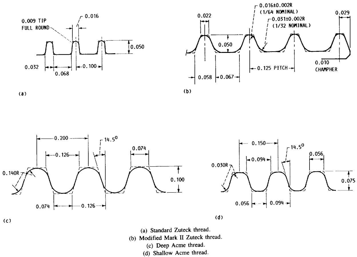
Figure 7.1-2.—Threads used on portion of metal studs embedded in laminated wood. All threads are ring shape (helix angle, 0°). (Dimensions are in inches.)
