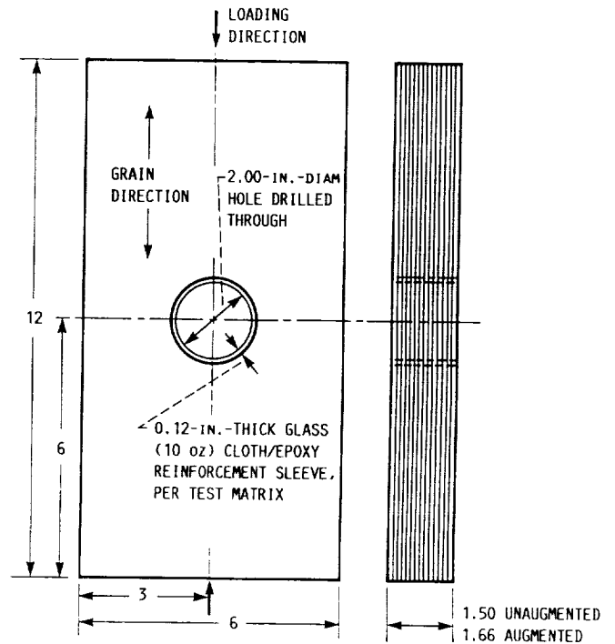
Figure 2.2-9.—Specimen for testing effects of unreinforced and glass-fiber-fabric-reinforced central hole. (Dimensions are in inches.)
