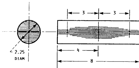
Figure 2.2-15.—Compression test specimen. (Dimensions are in inches.)
