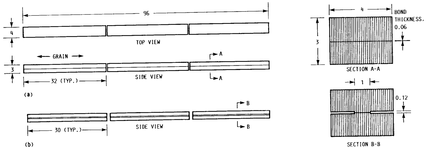
(a) Saw cut 96-in.-long strips into 32-in.-long pieces; bond two pieces at centerline with epoxy asbestos adhesive. (b) Saw cut 0.12-in.-thick slots; saw cut to 30 in. long; epoxy coat cut edges. (See section B-B.)
