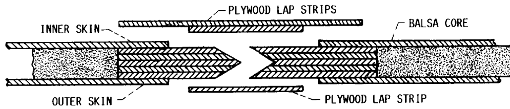
DETAILS OF SKIN JOINT WHERE FUSELAGE HALVES ARE MATED; PLYWOOD LAP STRIPS ARE GLUED AND SCREWED INTO SHELL MEMBERS
