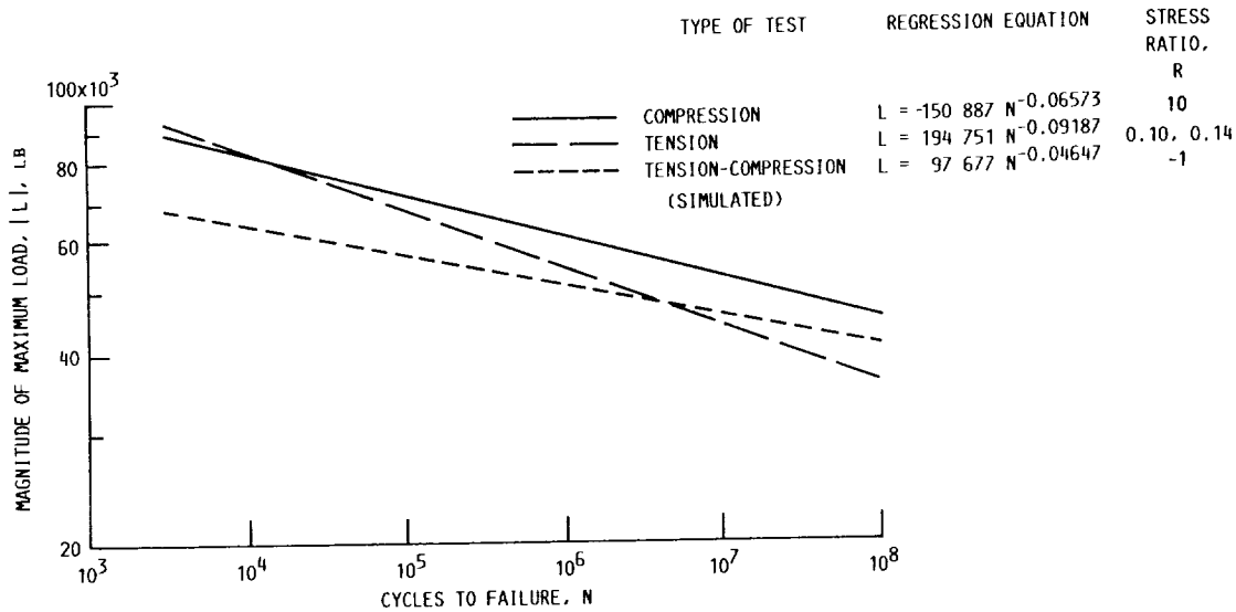
Figure 20.—Fatigue tests of metal studs (design 5) embedded in laminated Douglas fir/epoxy specimens with carbon-fiber-filled epoxy resin. Room-temperature tests. Reference figures 7.2-1(b) and 7.2-2(a) and (b) of chapter IV.
