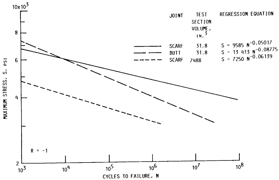
Figure 12.—Effect of specimen size and joint type on reverse axial tension-compression fatigue ( R = -1.0 ) parallel to grain for laminated Douglas fir/epoxy specimens. Data corrected to 6 percent laminate moisture content ( K = 1.57 ). Veneer grade, A+; test temperature, 70 °F. Reference figure 4.3-2 of chapter IV.
