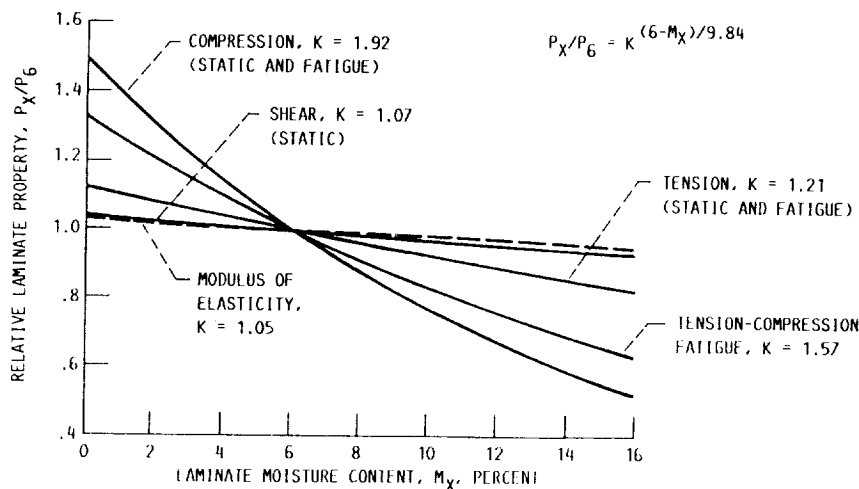
Figure 3.1-1.—Predicted variation with moisture content of mechanical properties of Douglas fir wood laminates parallel to grain (see eq. (8), chapter III).
