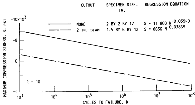
Figure 15.—Effect of 2-in.-diameter circular cutout on compression-compression fatigue ( R = 10 ) parallel to grain for laminated Douglas fir/epoxy specimens. Data corrected to 6 percent laminate moisture content ( K = 1.92 ). Veneer grade, A+; test temperature, 70 °F. Reference figure 4.2-7(a) of chapter IV.
