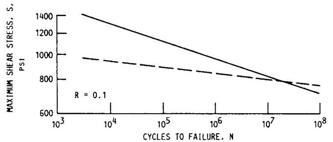
Figure 18.—Three-point-bending fatigue tests ( R = 0.1 ) on longitudinal wedge and butt joints. Epoxy-asbestos adhesive in joints 1 in. wide. Data corrected to 6 percent laminate moisture content ( K = 1.26 ). Test temperature, 70 °F. Reference figure 6.4-1(c) of chapter IV.
