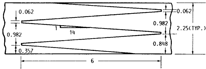
Figure 2.3-7.—Detail of machined fingers in augmented specimens for tensile tests. Pitch, 2.344 in. (Dimensions are in inches.)
