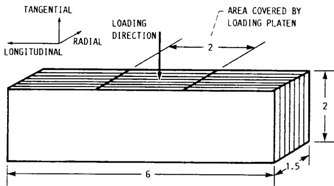
Figure 2.2-8.—Test specimen for compression perpendicular to grain. (Dimensions are in inches.)
