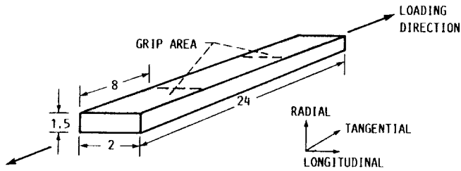
Figure 2.2-6.—Test specimen for tension perpendicular to grain (tangential direction). (Dimensions are in inches.)
