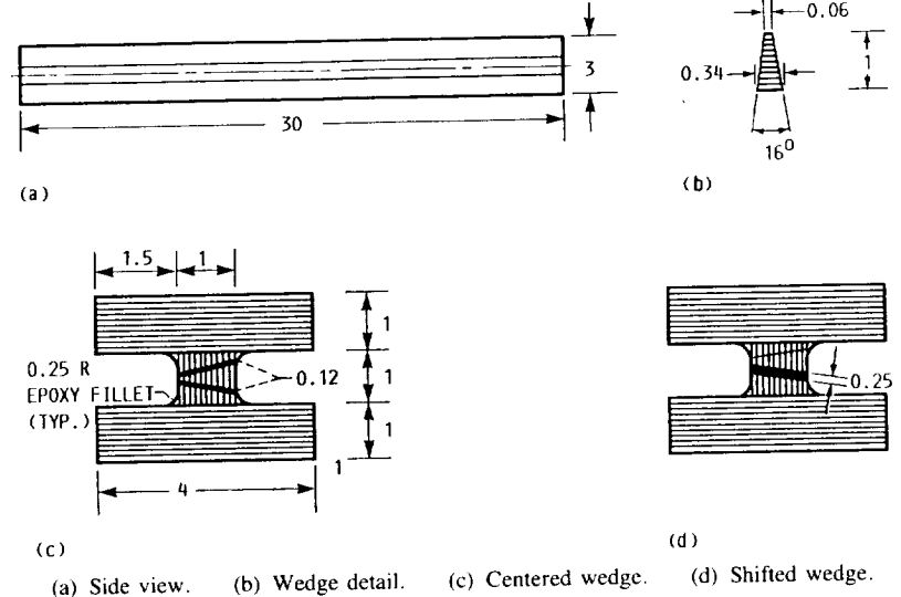
Figure 2.3-11.—Longitudinal wedge joint test specimens. (Dimensions are in inches.)
