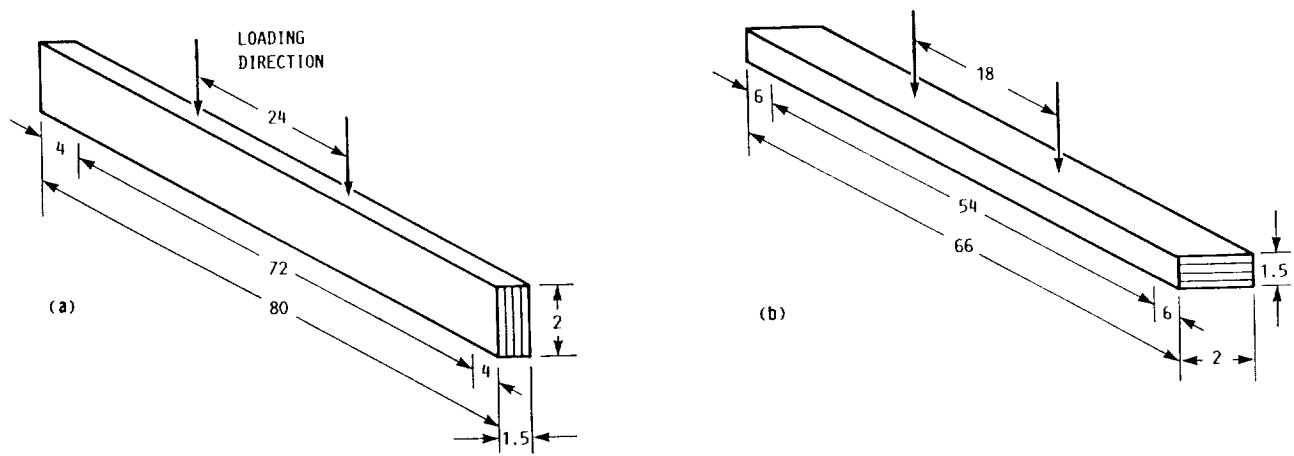
Figure 2.2-12.—Specimens for bending with vertical and horizontal laminations. (Dimensions are in inches.)
