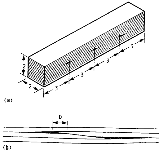
(a) Staggered scarf joint test sample configuration. (Control specimens have same overall dimensions but contain no scarf joints.) (b) Overlap joint: 50 percent overlap, D = 0.50 in.; 25 percent overlap, D = 0.25 in. (Overlap joints tend to distort somewhat within the laminate.)
