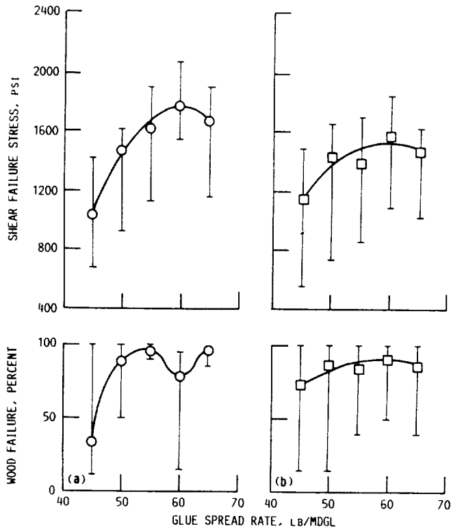
Figure 3.3-1.—Effect of glue spread rate on shear strength and percent of failure in wood surface for laminated Douglas fir/epoxy specimens. Shear parallel to grain and laminations. Strength corrected to 6 percent laminate moisture content ( K = 1.07 ).
