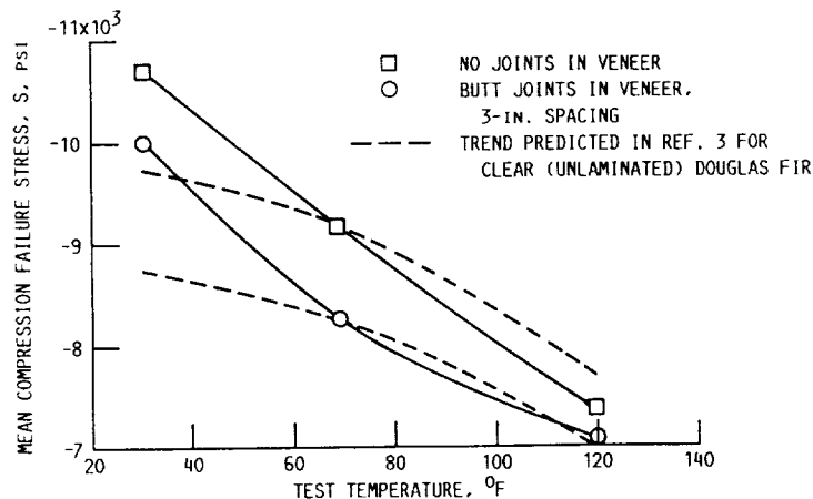
Figure 3.2-1.—Effect of test temperature on compression failure stress parallel to grain of laminated Douglas fir/epoxy test specimens. Each data point is mean of 10 specimens corrected to 6 percent laminate moisture content ( K = 1.92 ).
