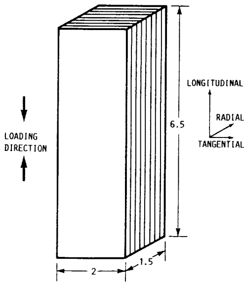
Figure 2.2-7.—Test specimen for compression parallel to grain. (Dimensions are in inches.)
