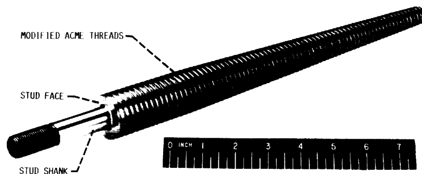
Figure 11.—Steel stud typical of type bonded into end of 60-ft wind turbine blade for attachment to rotor hub.
