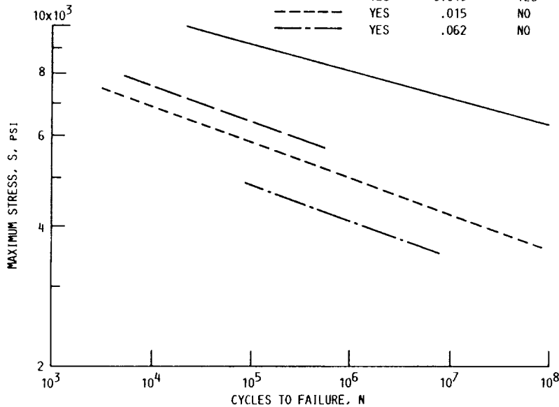
Figure 19.—Effect of finger joints on tension-tension fatigue ( R = 0.1 ) parallel to grain for laminated Douglas fir/epoxy dogbone specimens. Finger joints 10 in. long; finger slope, 1:10. Dogbone specimens, 2.25 in. in diameter at test section and 57 in. long. Data corrected to 6 percent laminate moisture content ( K = 1.21 ). Veneer grade, A+; test temperature, ~68 °F. Reference figure 6.2-1 of chapter IV.
