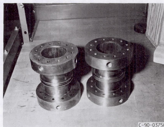
FIGURE 7. - PHOTOGRAPH OF "GROWN ON" STIFFENING RINGS.
