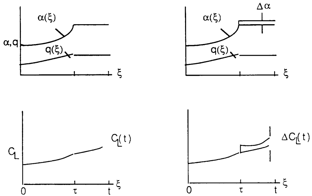
Fig. 2 Indicial response
