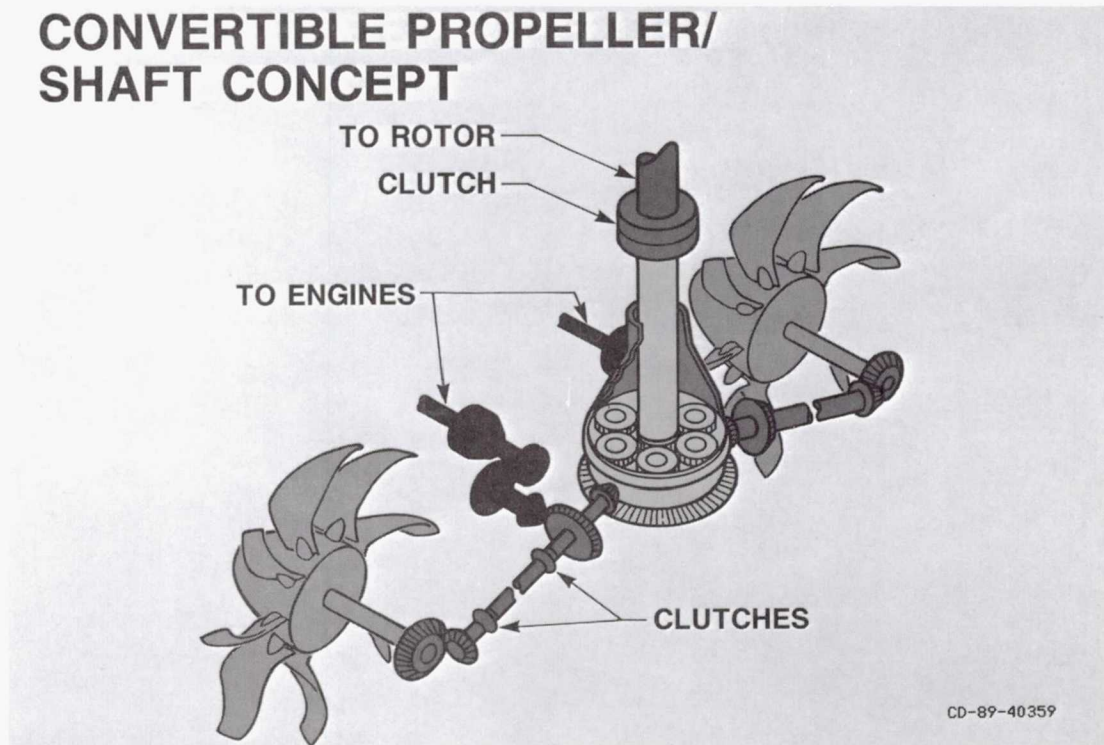
Figure 7. EXAMPLE OF SHAFT /CLUTCH SYSTEM WITH PROPULSORS REMOTE FROM ENGINES
