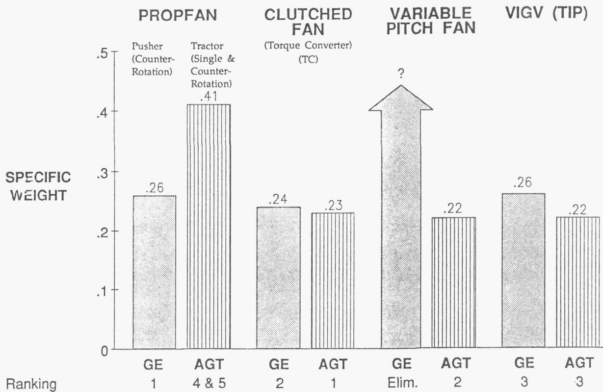
Figure 10. CONVERTIBLE ENGINE SPECIFIC WEIGHTS (Pounds Per Horsepower At Sea Level)
