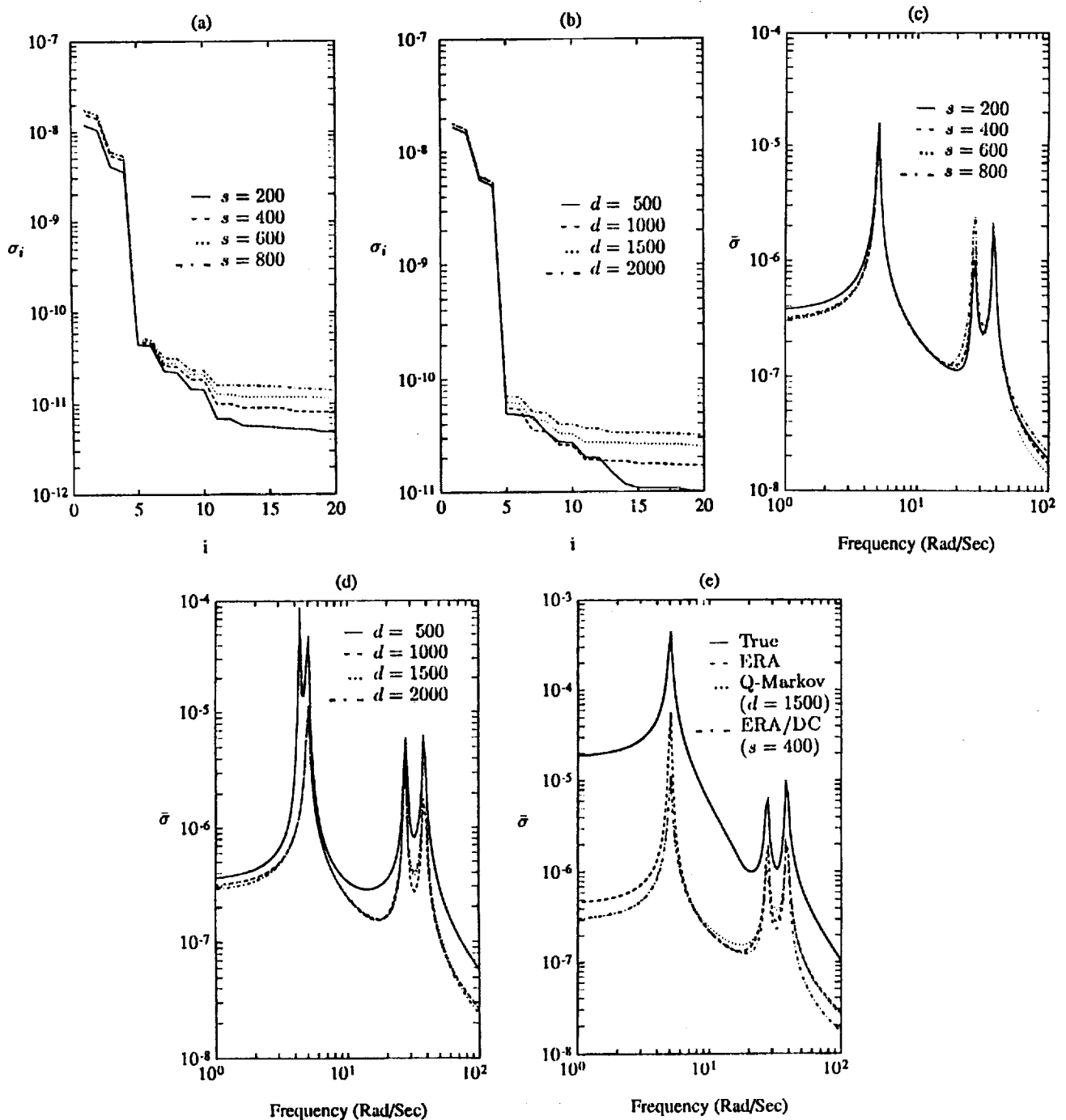
Figure 5 High noise identification results:
