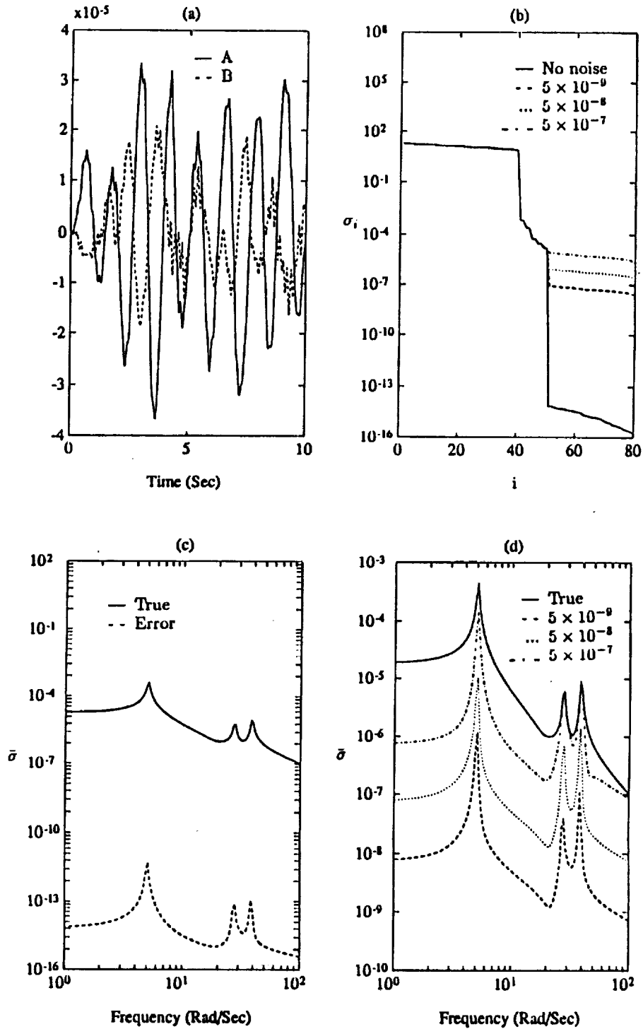
Figure 8 Identification results for the MDVV algorithm:
