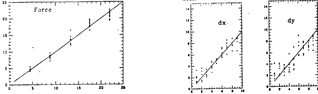
Figure 5: Actual vs Calculated Values for Holding Force and Position Offset
