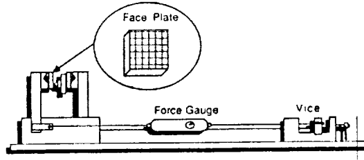
Figure 4: Experimental Setup for Accurate Force Measurements
