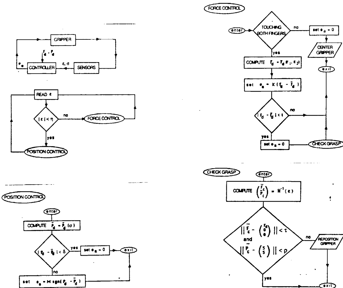
Figure 7: Control System Block Diagram
