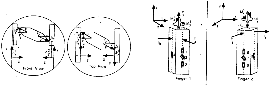
B. Force and Moment Diagram
