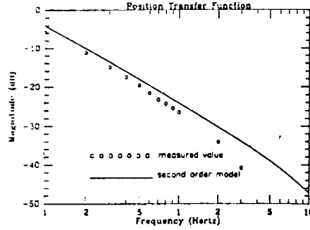
Figure 1: Theoretical vs. Actual Position Transfer Function
