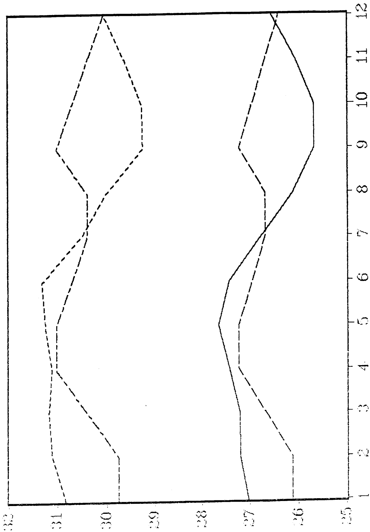
Figure 6 Historical and Predicted Average Monthly Temperatures
