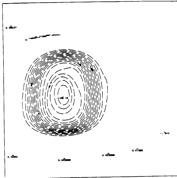
Figure 26: Plot of vorticity contours at time t^* = 10 , C_e = 0
