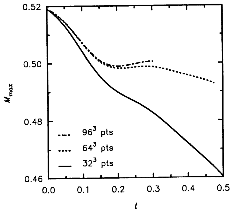
Figure 23: Time history of maximum Mach number, 3D.
