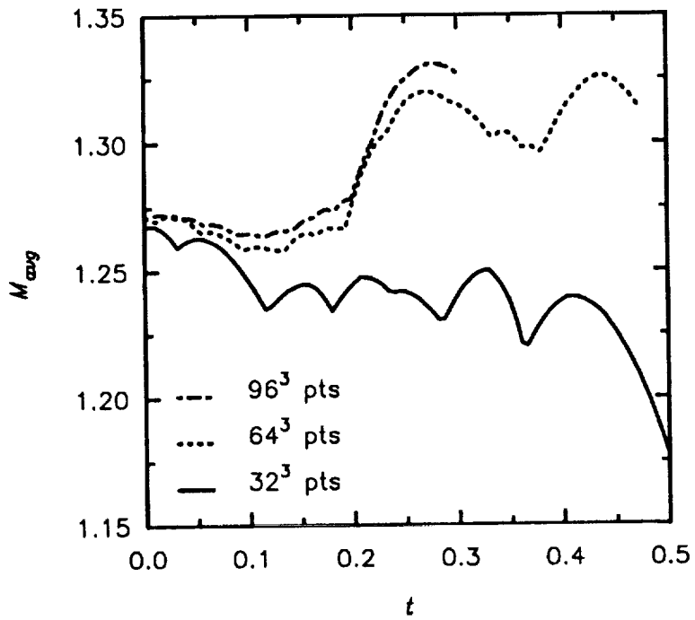
Figure 22: Time history of average Mach number, 3D.
